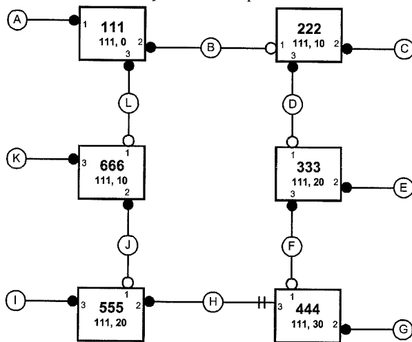
Figure 17-6—“Ring Backbone” example
