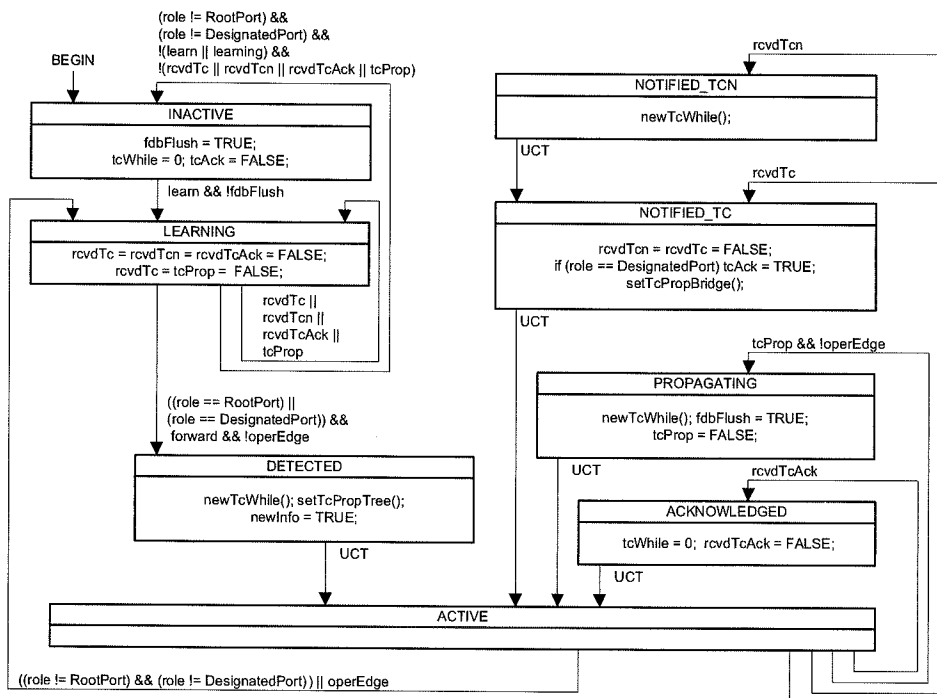
Figure 17-25—Topology Change state machine
