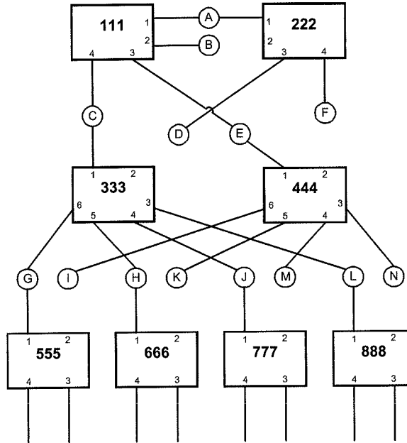
Figure 17-3—Active topology example
