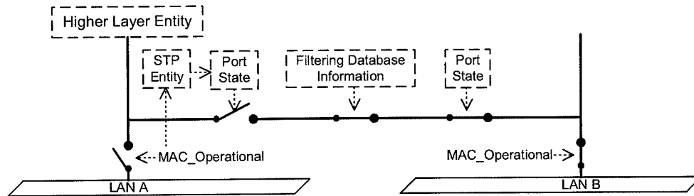
Figure 7-14—Effect of Port State
