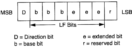
Figure C-5—Base and extended LF bits on the second octet of the RC field
