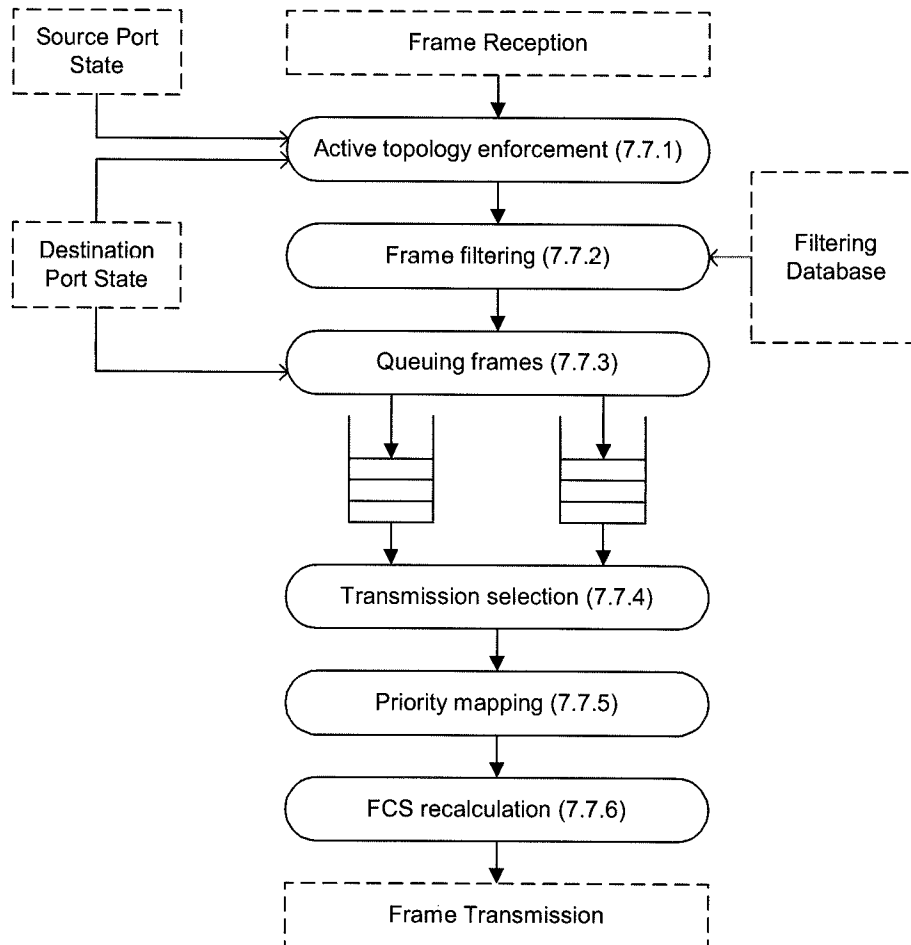
Figure 7-8—Operation of the Forwarding Process
