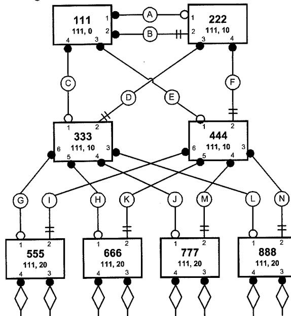
Figure 17-4—Port Roles and Port States
