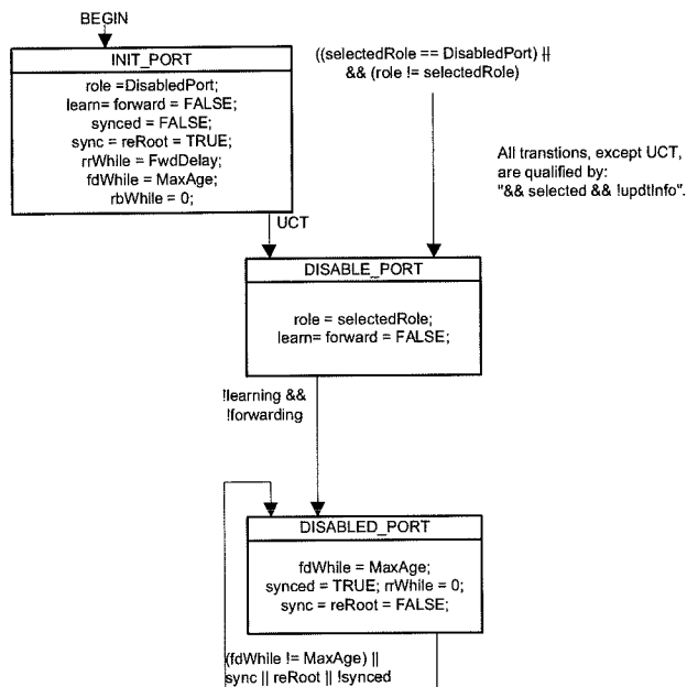
Figure 17-20—Disabled Port role transitions
