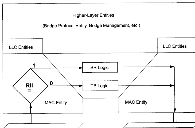
Figure C-1—SRT Bridge operation logic
