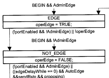
Figure 17-16—Bridge Detection state machine
