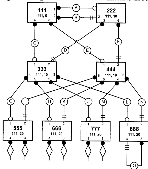
Figure 17-5—Backup Port example
