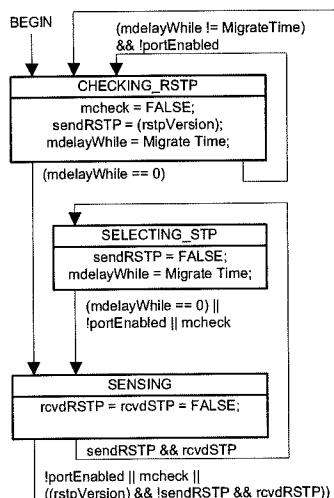
Figure 17-15—Port protocol migration state machine
