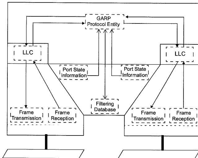
Figure 7-7—Operation of GARP
