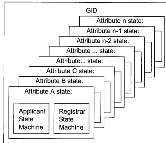
Figure 12-5—GID architecture
