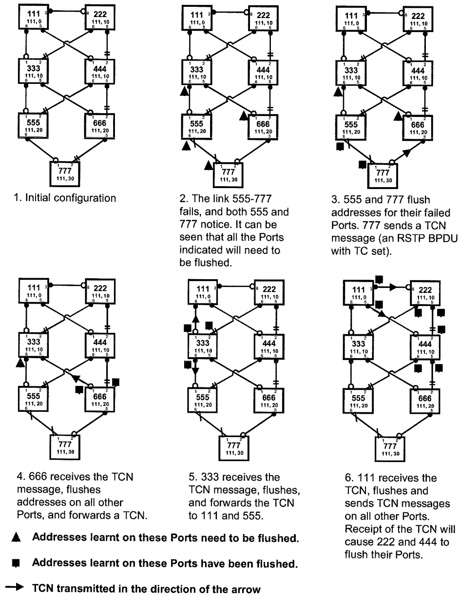
Figure 17-10—Address flushing—worked example
