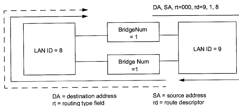
Figure C-9—Duplicate bridge number test illustration
