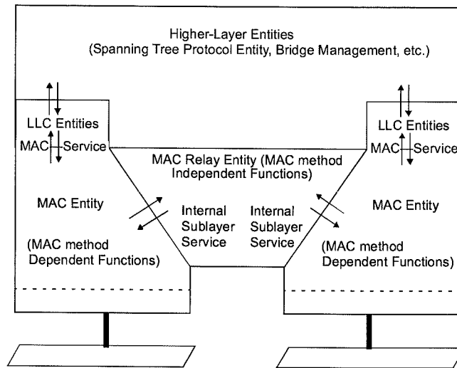
Figure 7-3—Bridge architecture
