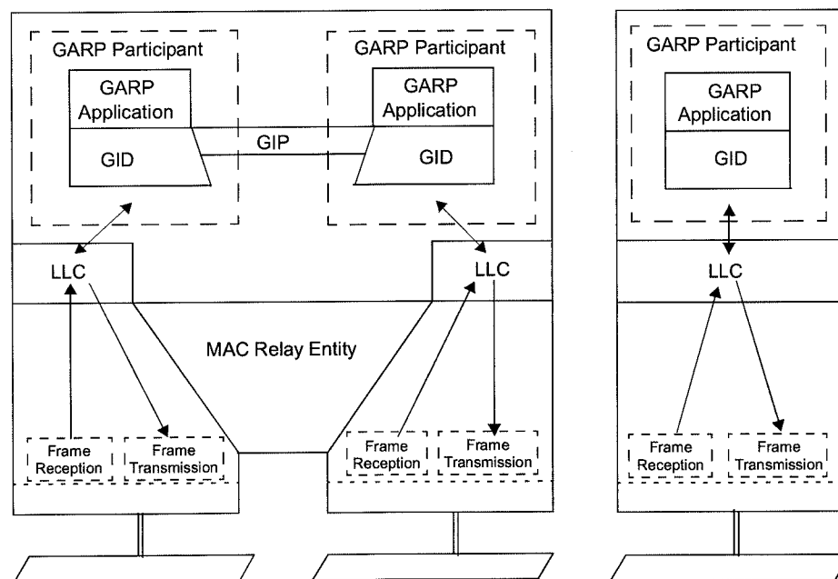
Figure 12-4—GARP architecture
