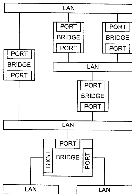
Figure 7-1—A Bridged Local Area Network
