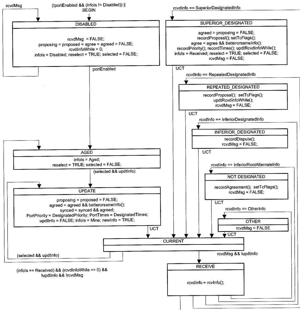
Figure 17-18—Port Information state machine
