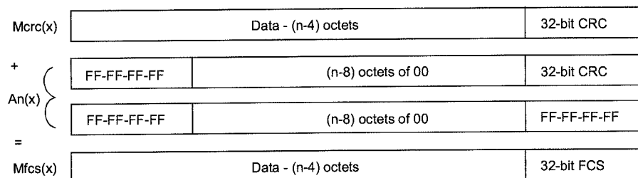
Figure F-1—Converting a CRC to an FCS
