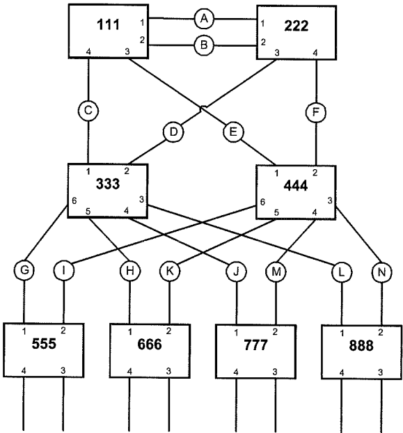
Figure 17-2—Physical topology example
