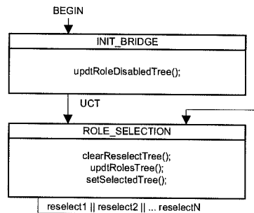
Figure 17-19—Port Role Selection state machine
