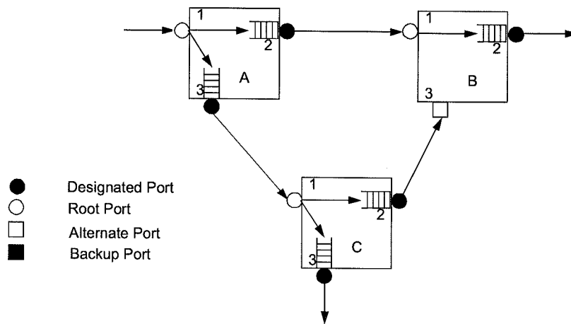
Figure K-1—Frame duplication scenario
