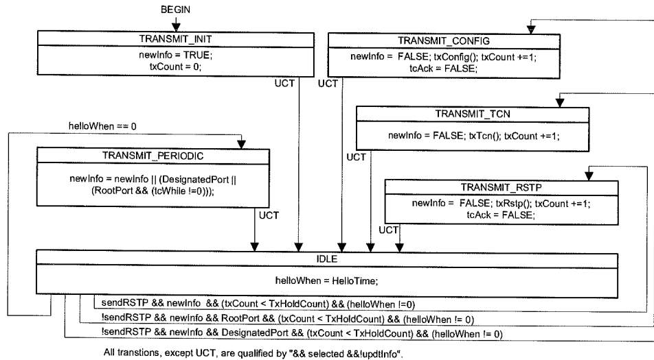
Figure 17-17—Port Transmit state machine
