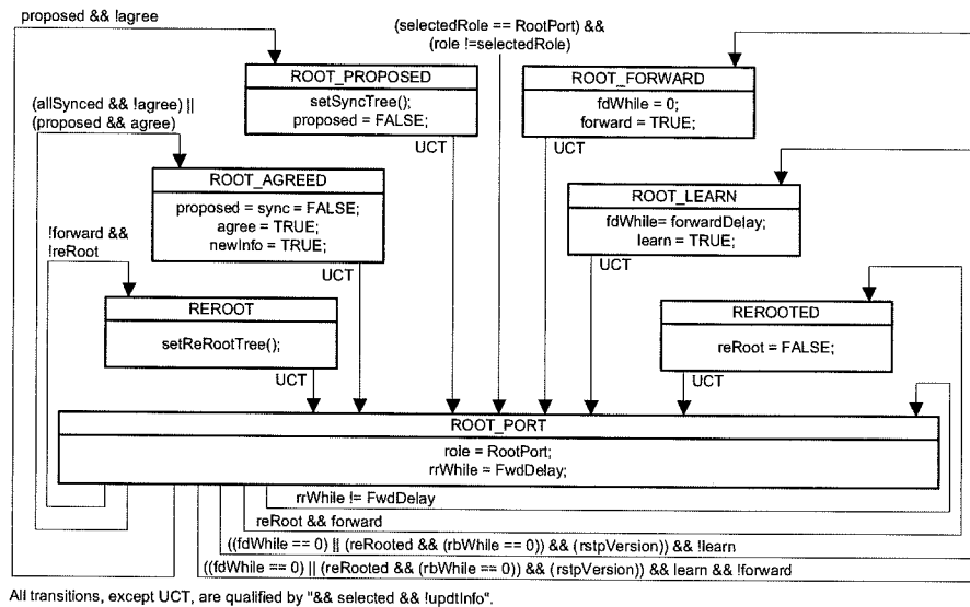
Figure 17-21—Root Port role transitions
