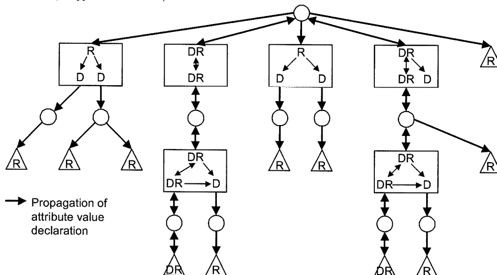
Figure 12-2—Example —Attribute value propagation from two stations
