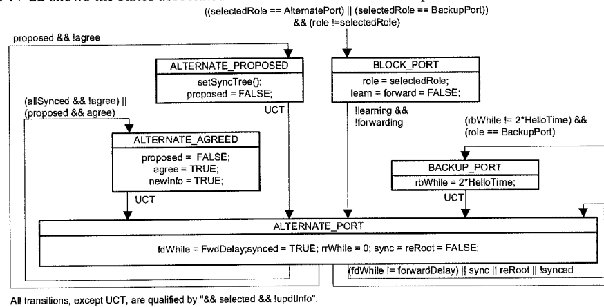
Figure 17-23—Alternate and Backup Port role transitions
