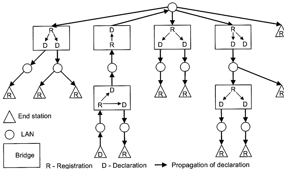
Figure 12-1—Example—Attribute value propagation from one station
