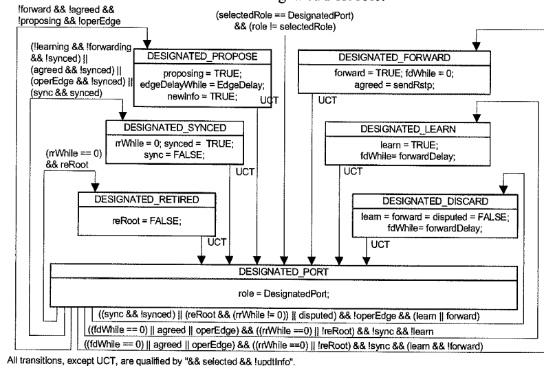
Figure 17-22—Designated port role transitions
