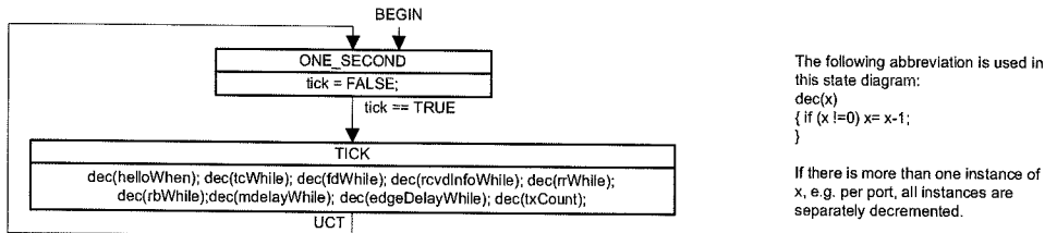
Figure 17-13—Port Timers state machine
