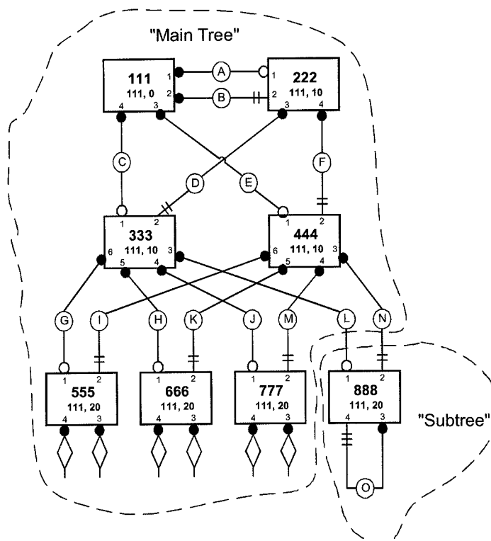
Figure 17-11—Root Port transition—tree partitioning
