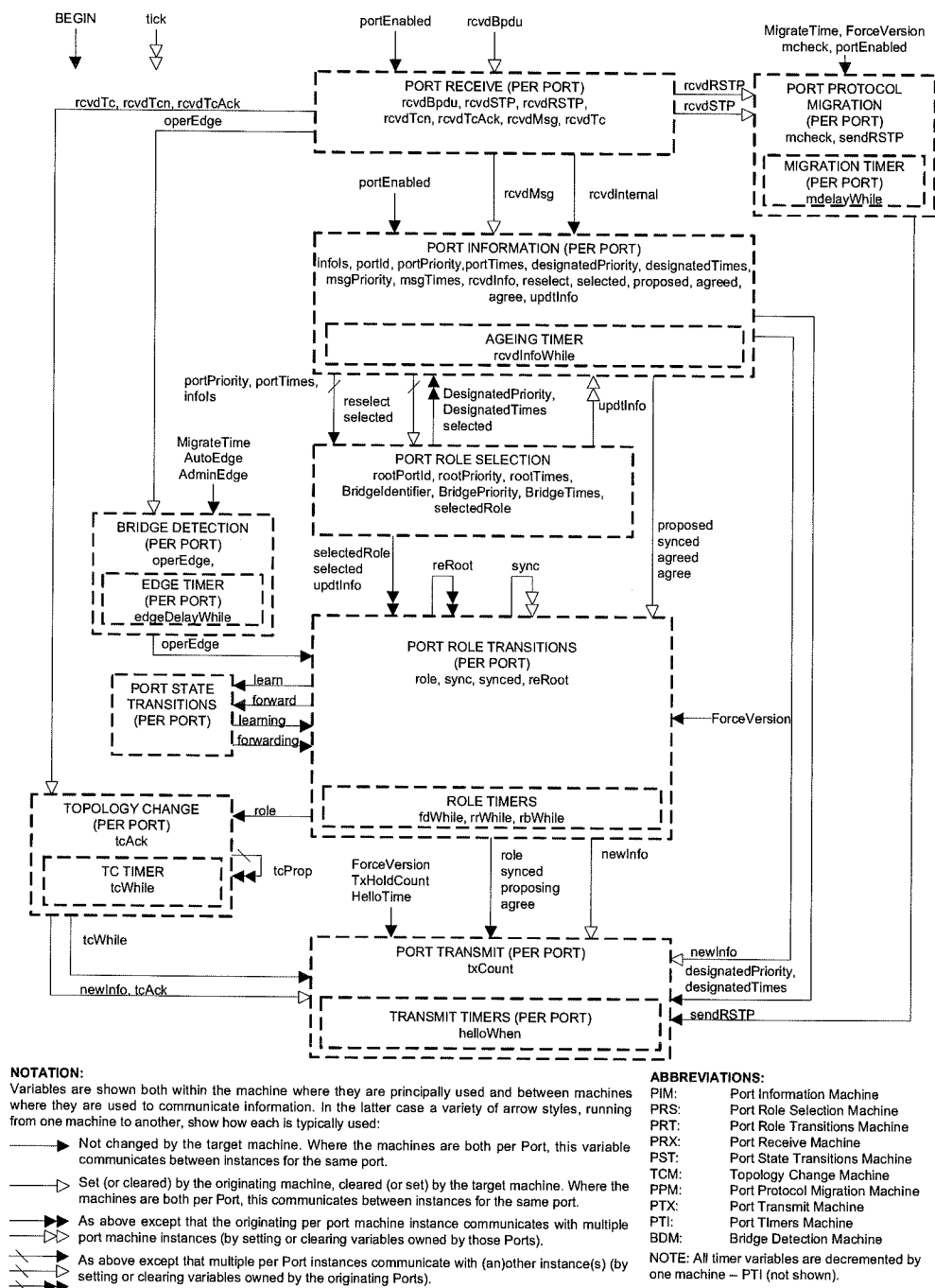
Figure 17-12—RSTP state machines—overview and interrelationships
