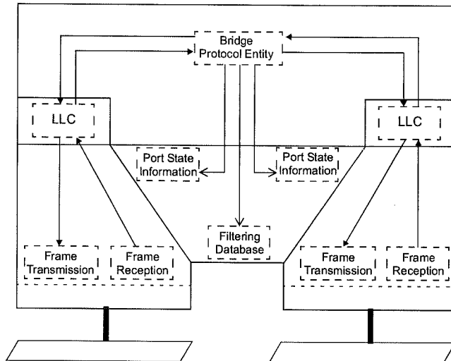
Figure 7-6—Operation of inter-bridge protocol
