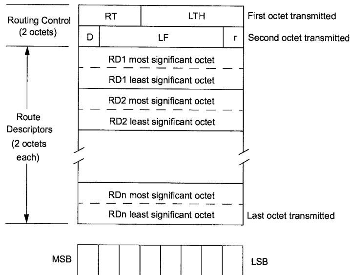
Figure C-4—Routing information field
