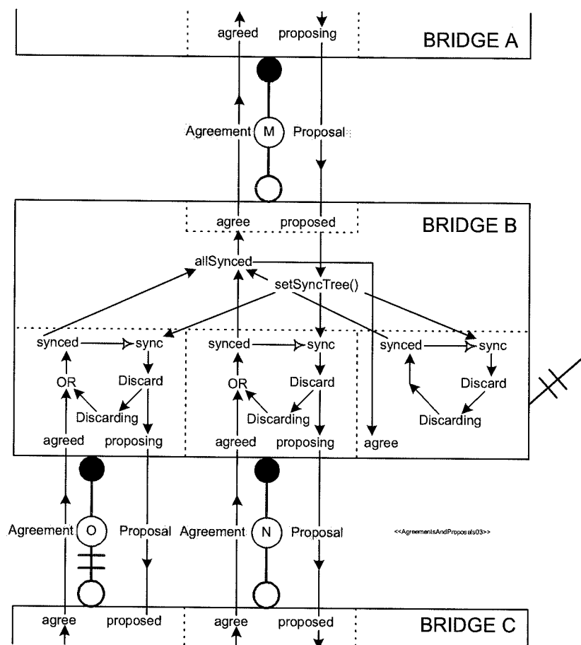
Figure 17-8—Agreements and proposals
