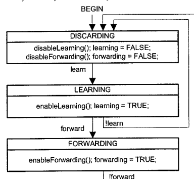
Figure 17-24—Port State Transition state machine
