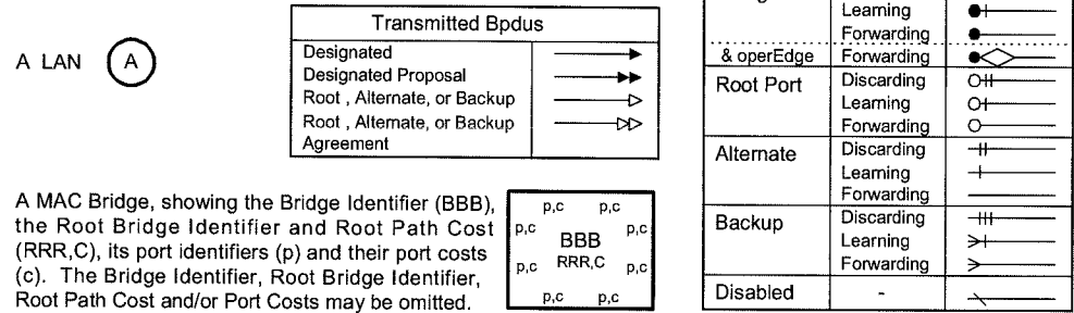
Figure 17-1—Diagrammatic conventions
