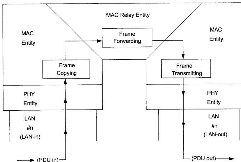
Figure C-2—Elements of a Source-Routed Bridge
