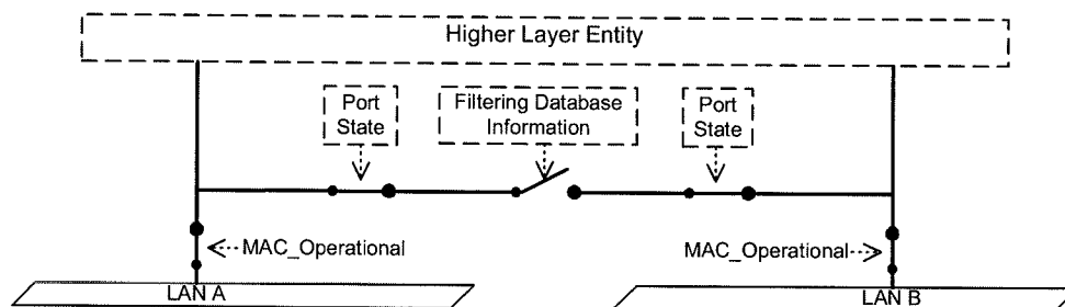
Figure 7-11—Per-Port points of attachment
