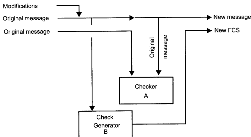
Figure F-2—Detection Lossless Circuit
