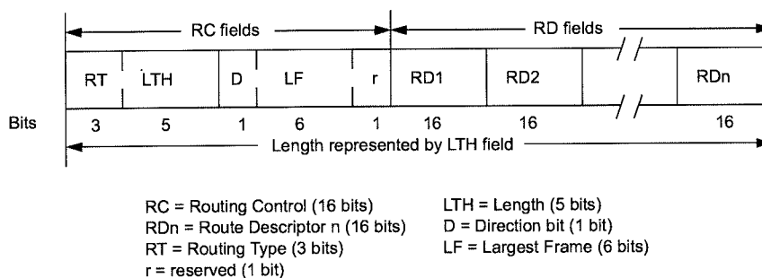
Figure C-3—Structure of the routing information field
