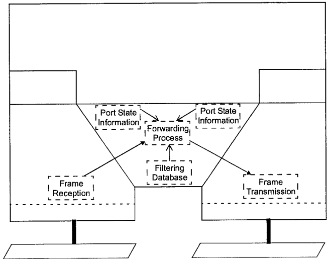
Figure 7-4—Relaying MAC frames
