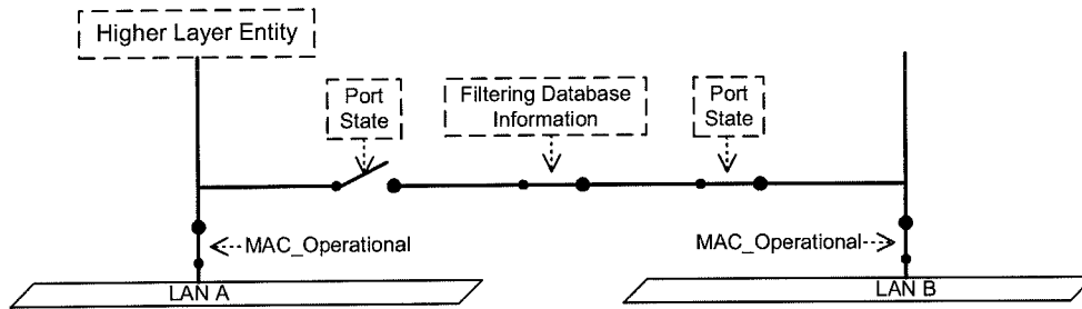
Figure 7-13—Single point of attachment—relay not permitted
