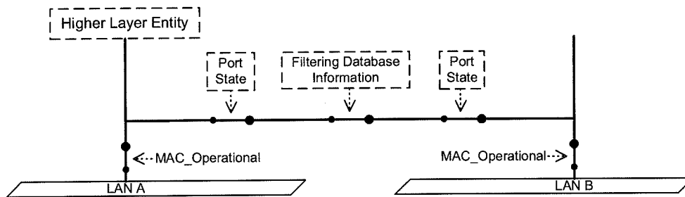
Figure 7-12—Single point of attachment—relay permitted
