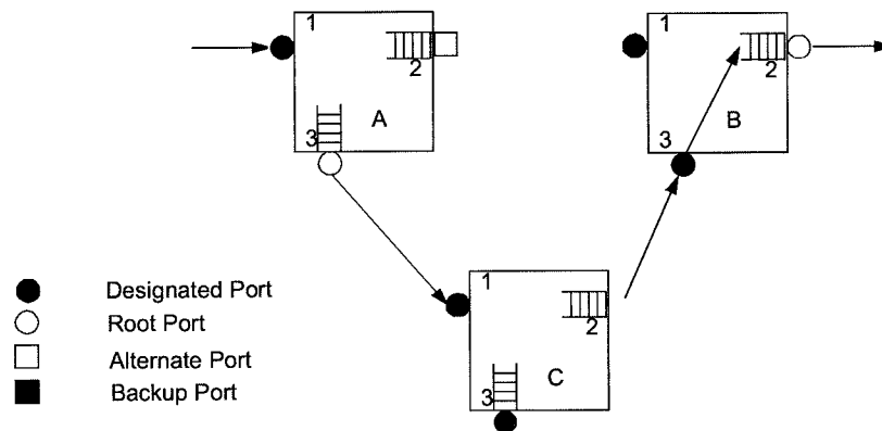
Figure K-2—Frame misordering scenario
