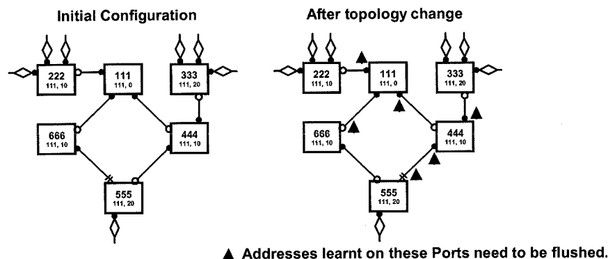
Figure 17-9—Address flushing example
