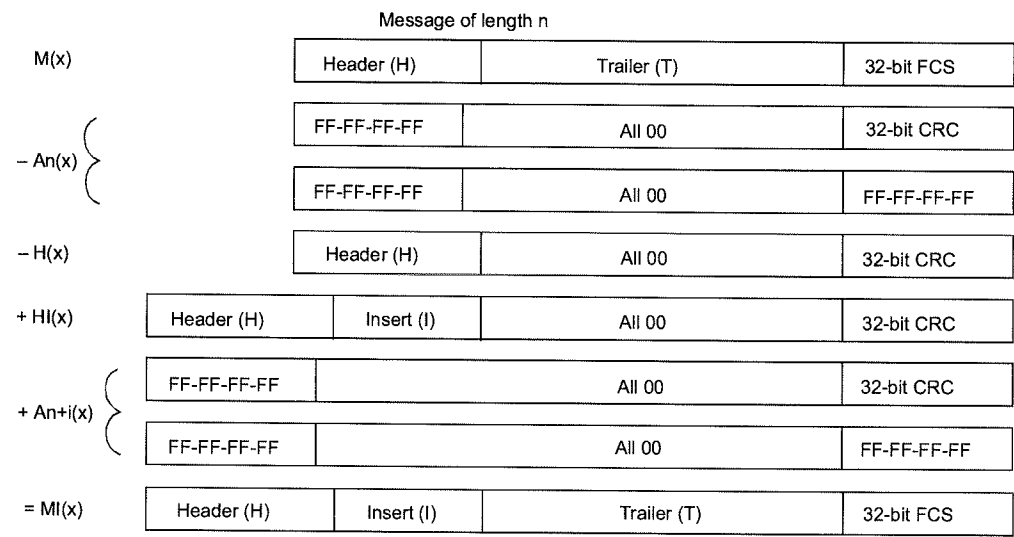
Figure F-4—Field insertion adjustment
