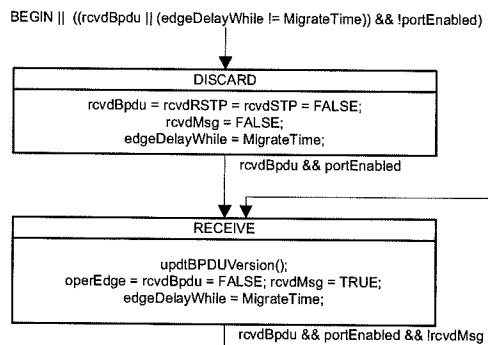
Figure 17-14—Port Receive state machine
