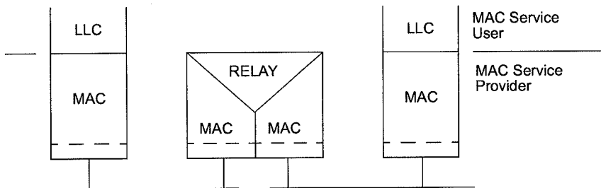
Figure 6-1—Internal organization of the MAC sublayer
