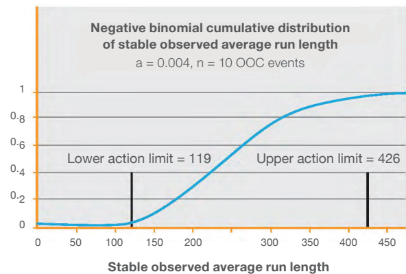
Figure 2 Negative binomial sampling distribution of (RL) for n = 10 OOC events
