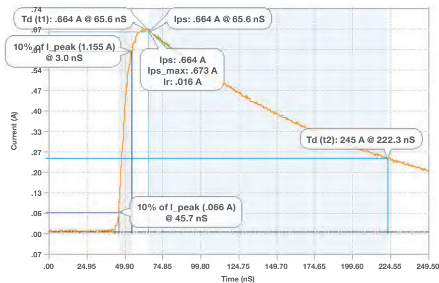
Example waveform, 1kV HBM through short
