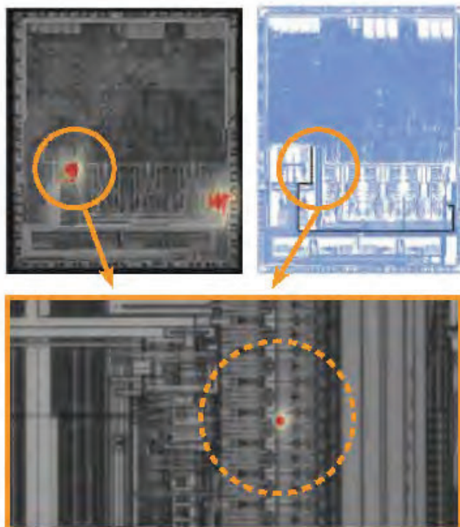
Hotspot observed on the device
