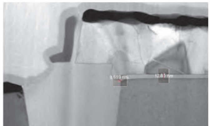
STEM Image
