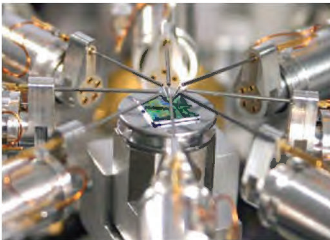
Nanoprober
