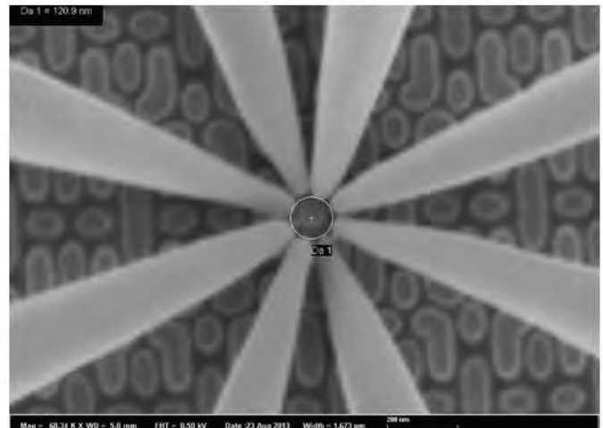
Nanoprober
