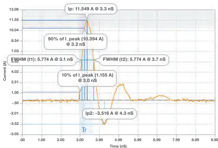
Example waveform, 1kV HBM through short
