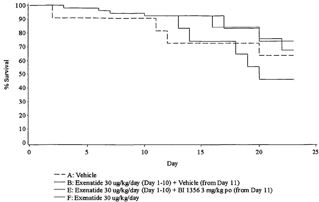
Figure 2: Survival plots
