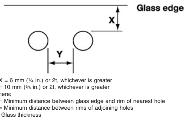
FIG. 1 Placement of Holes
