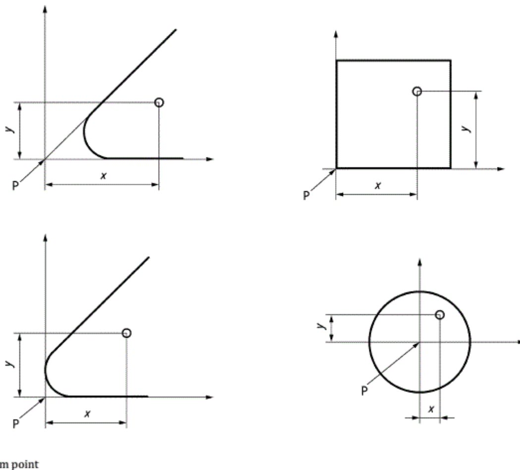
Figure 19 — Examples of the positioning of holes relative to the datum point
