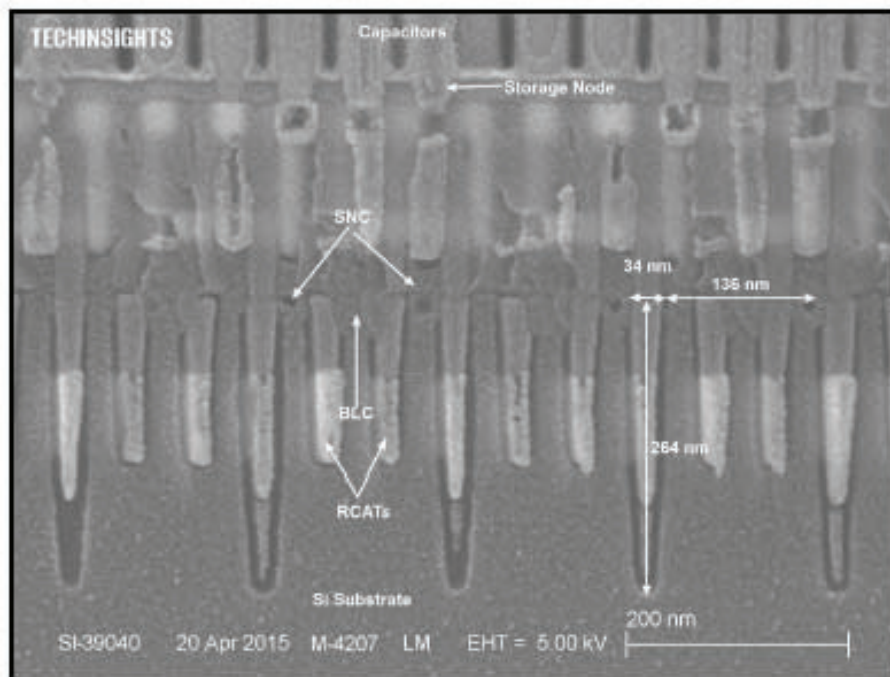
Figure 3.2.6: Recessed channel access transistors, bitline contacts and storage node contact, SEM cross-section in the direction 20 degree to bitline (parallel to active).
