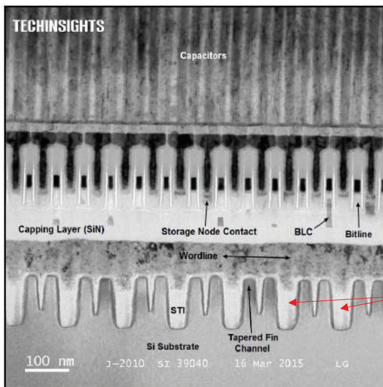
Figure 3.3.6: Bitlines, buried wordline, silicon fin under buried wordline, TEM cross-section along a wordline.
