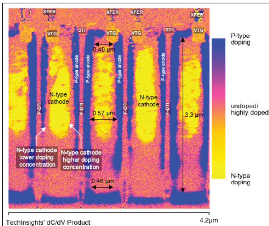
Figure 4.4.4 Pixel Array Photodiode and VTG – SCM
