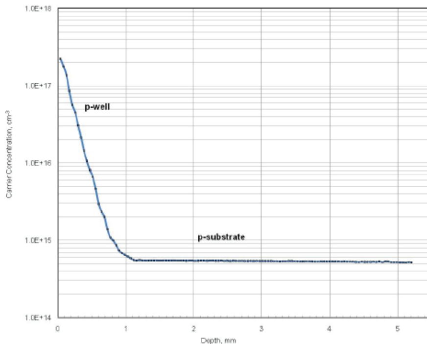
Figure 2.1.1: Spreading resistance profile of a peripheral P-well.
