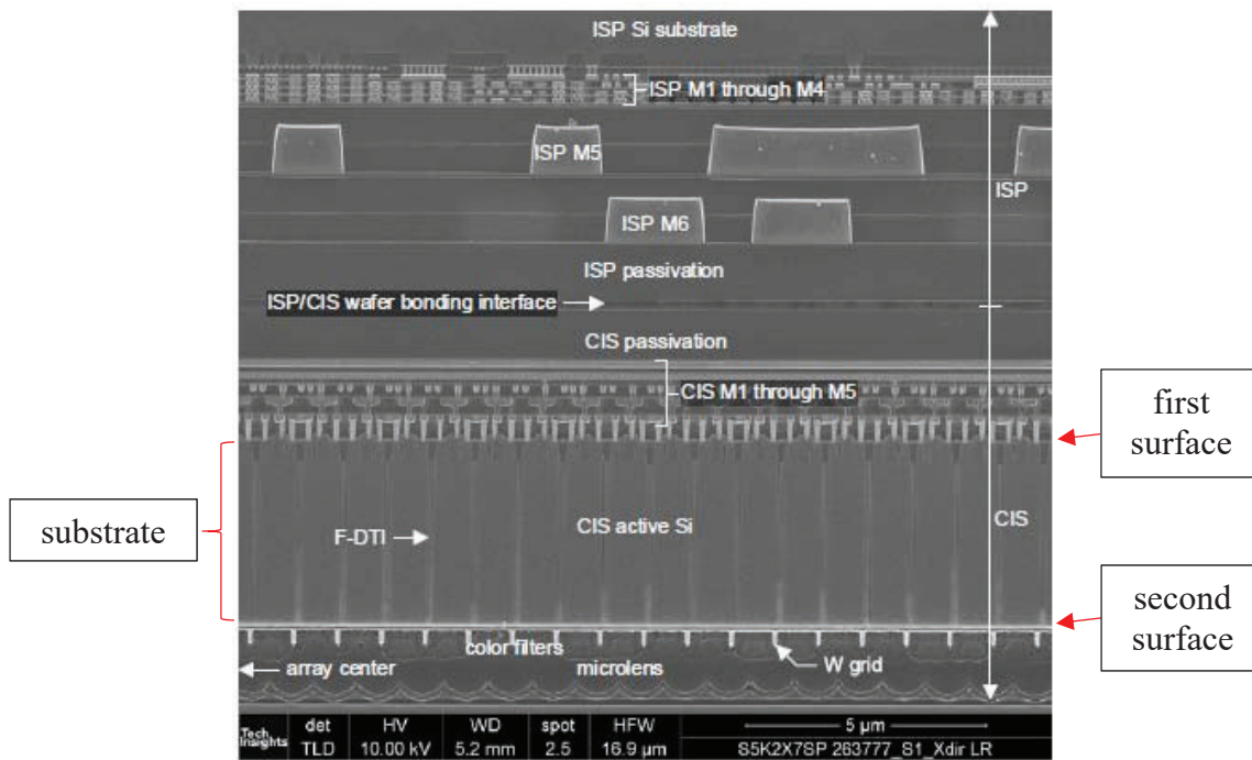
Figure 4.3.10 CIS Pixel Array General Structure – SEM
