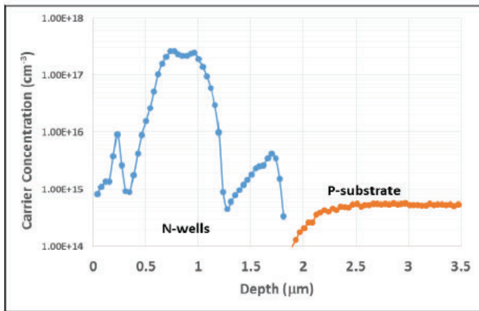
Figure 2.1.3: SRP profile of peripheral n-wells
