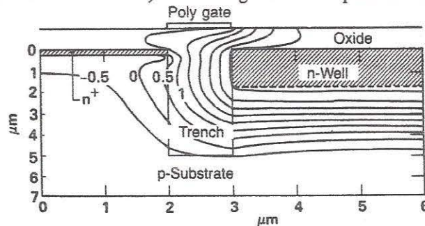
Fig. 6-33 The corresponding two-dimensional potential contours showing sidewall inversion; the simulation is done at Q_b = 5 \times 10^{10}\ \text{cm}^{-2} , N_A = 6 \times 10^{14}\ \text{cm}^{-3} , V_{GD} = 3\ \text{V} , V_{GS} = 0\ \text{V} , V_{SB} = -1\ \text{V} . 120 (© 1983 IEEE).
