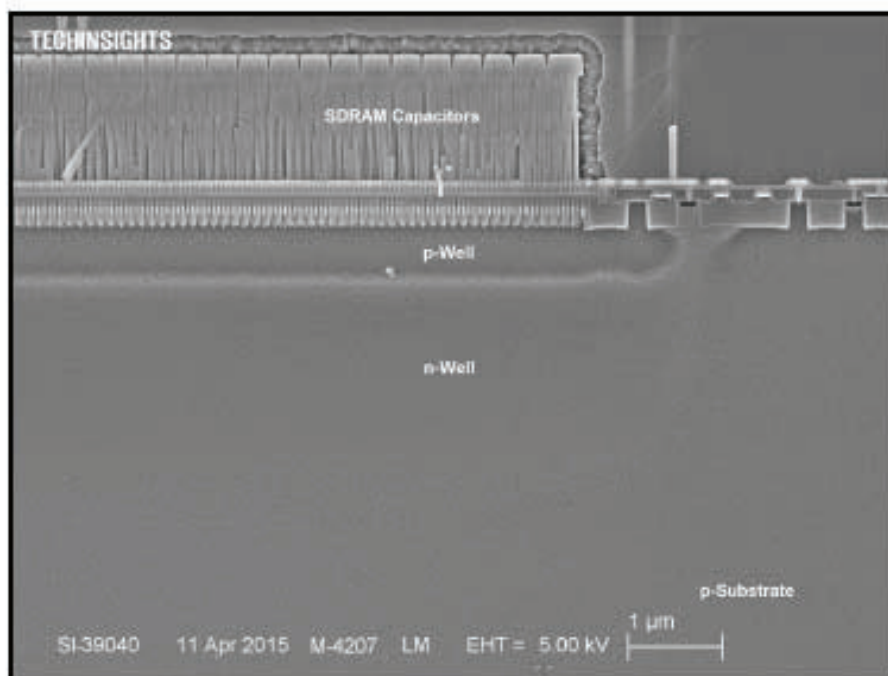
Figure 2.1.3: SDRAM array well structure, SEM cross-section through edges of SDRAM array in bitline direction, silicon etch.
