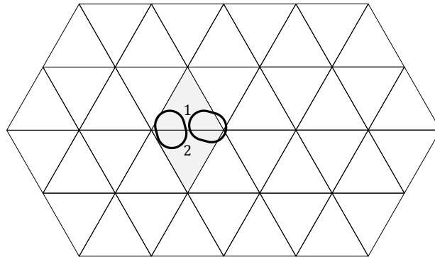
Figure C-3: Two Power Receivers covering a single Primary Cell
