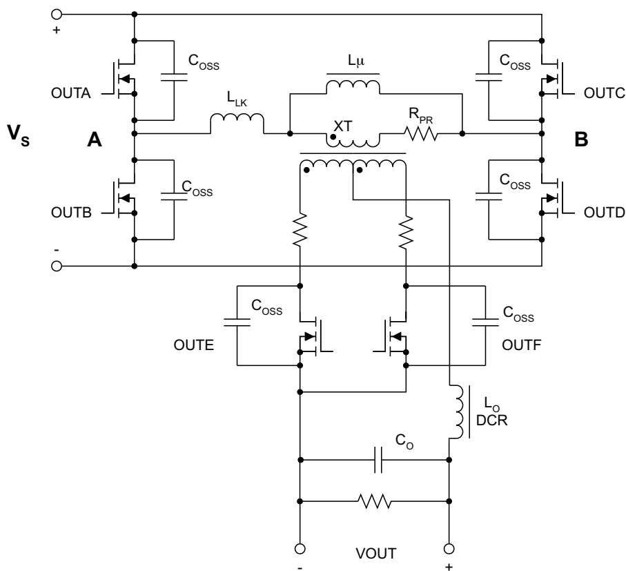
Figure 21. Power Stage
