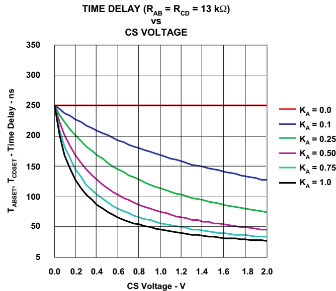
Figure 5. Delay Time Set T_{ABSET} and T_{CDSET} (Over CS voltage variation and selected K_A for R_{AB} and R_{CD} equal 13 kΩ)
