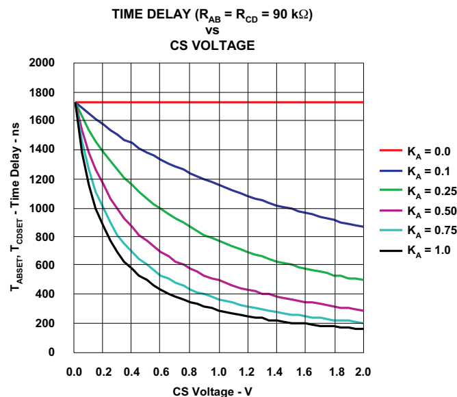
Figure 6. Delay time set T_{ABSET} and T_{CDSET} (Over CS voltage variation and selected K_A for R_{AB} and R_{CD} equal 90 kΩ)
