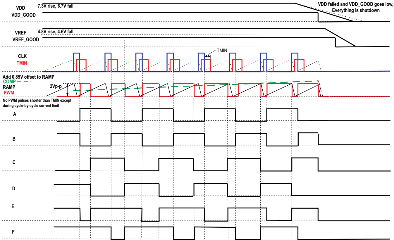
Figure 3. UCC28950 Timing Diagram
