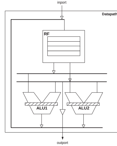
Figure 15. Target datapath organization for ones's counter
