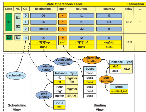
Figure 5. Scheduling & Binding window for an SF-SMD
