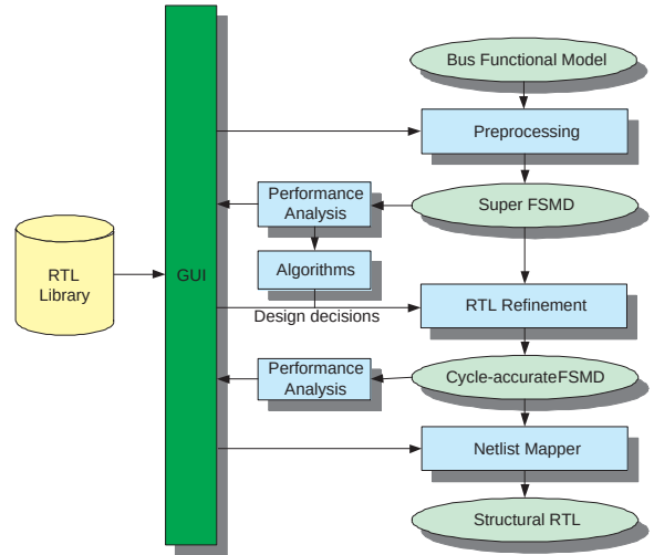
Figure 2. RTL design flow
