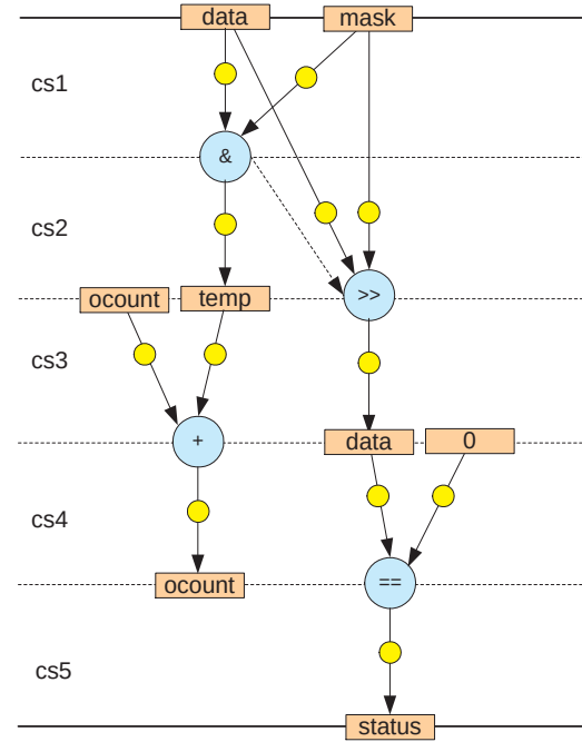
Figure 17. Scheduled CDFG for state S2 in one's counter
