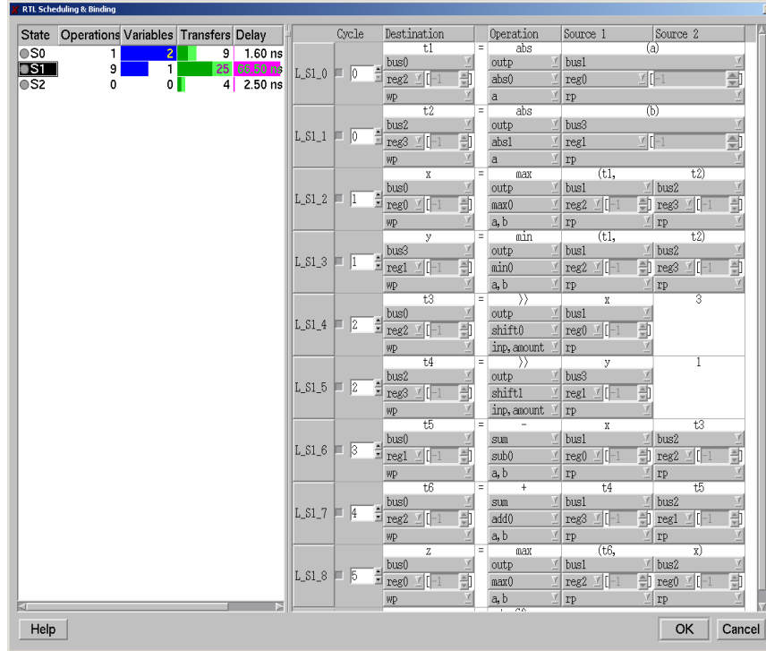
Figure 9. A scheduling and binding result of SRA
