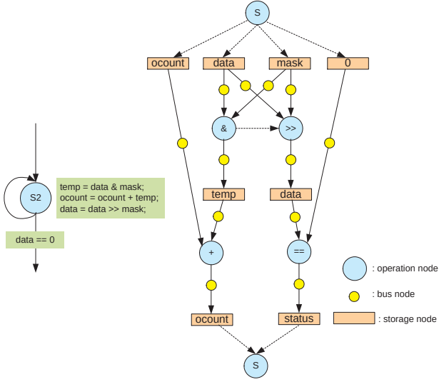
Figure 16. CDFG for state S2 in one's counter
