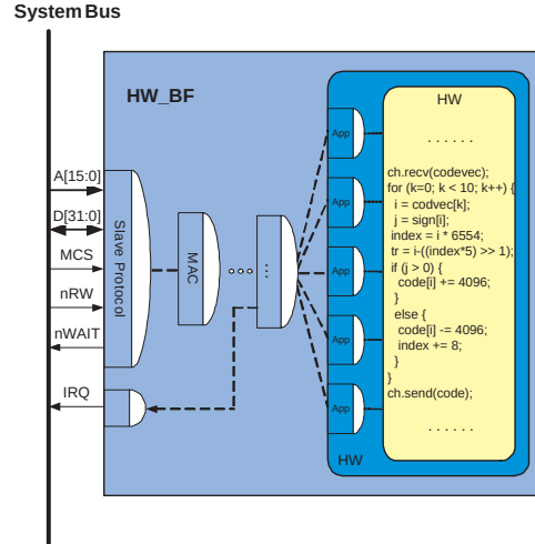
Figure 3. Bus functional model for custom hardware
