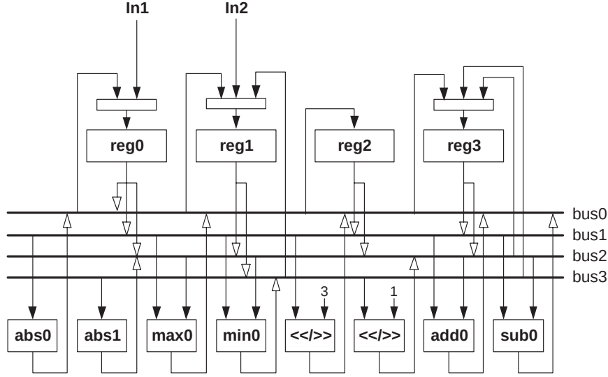
Figure 10. A datapath for SRA
