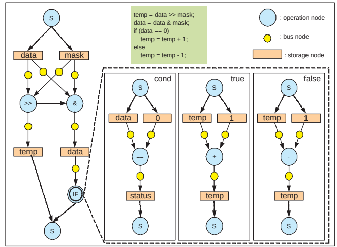
Figure 11. CDFG for unmapped (style 1) RTL description)
