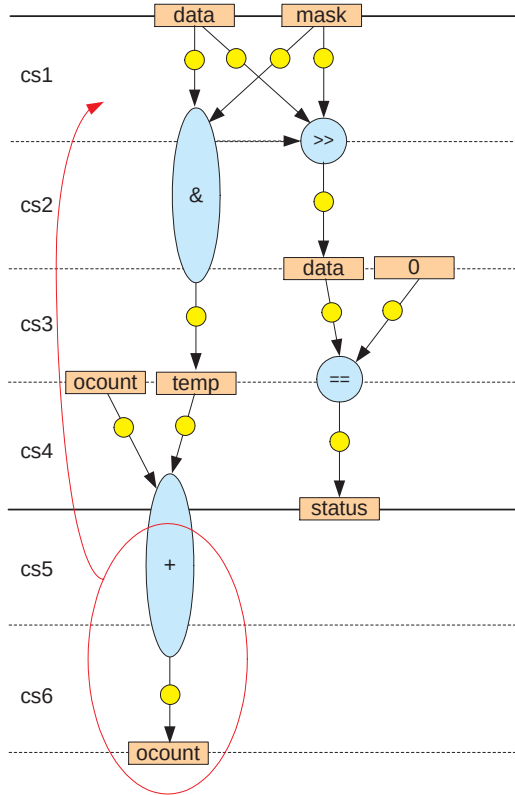
Figure 18. Scheduling process for one's counter (II)
