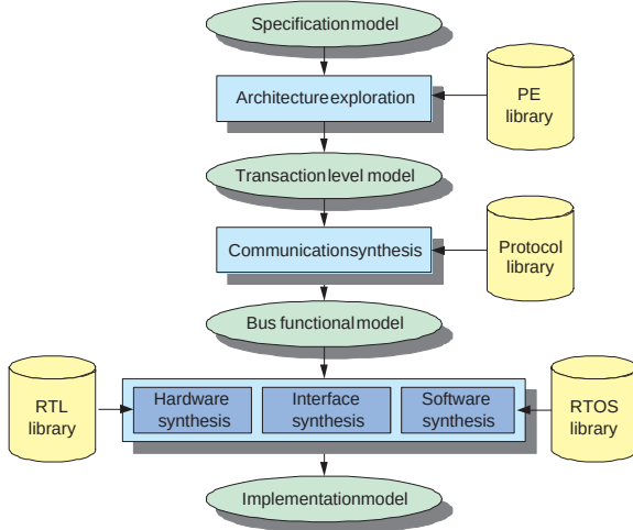
Figure 1. System design flow
