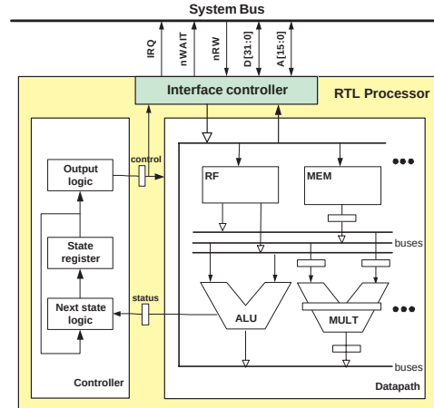
Figure 6. RTL processor architecture
