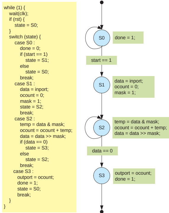
Figure 14. FSMD for one's counter
