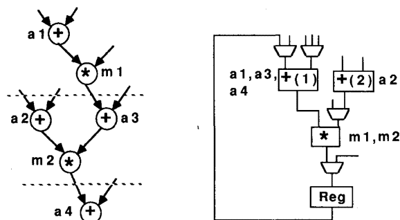
Fig. 9. Greedy data-path allocation.
