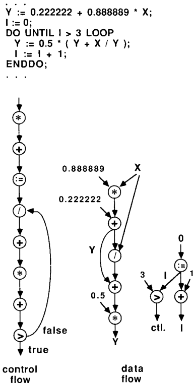
Fig. 1. High-Level specification and internal representation for sqrt.
