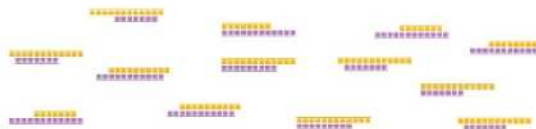
Figure 2 Fragmented DNA
