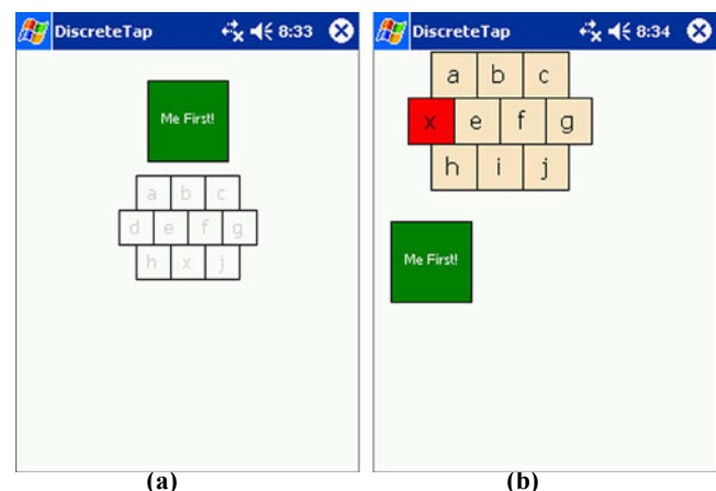
Figure 1. The experiment interface for the discrete target phase. (a) The startup view for a trial testing a 5.8 mm target in the center zone. (b) The display for a trial in the upper left zone as the user selects the 7.7 mm trial target (x).
