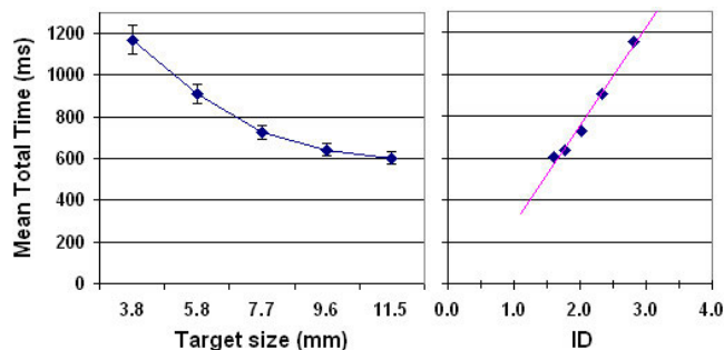
Figure 3. (a) Mean total time between the release of the start button and 'x' for each target size in the discrete target phase. (b) Relationship between movement time (MT) and index of difficulty (ID).
