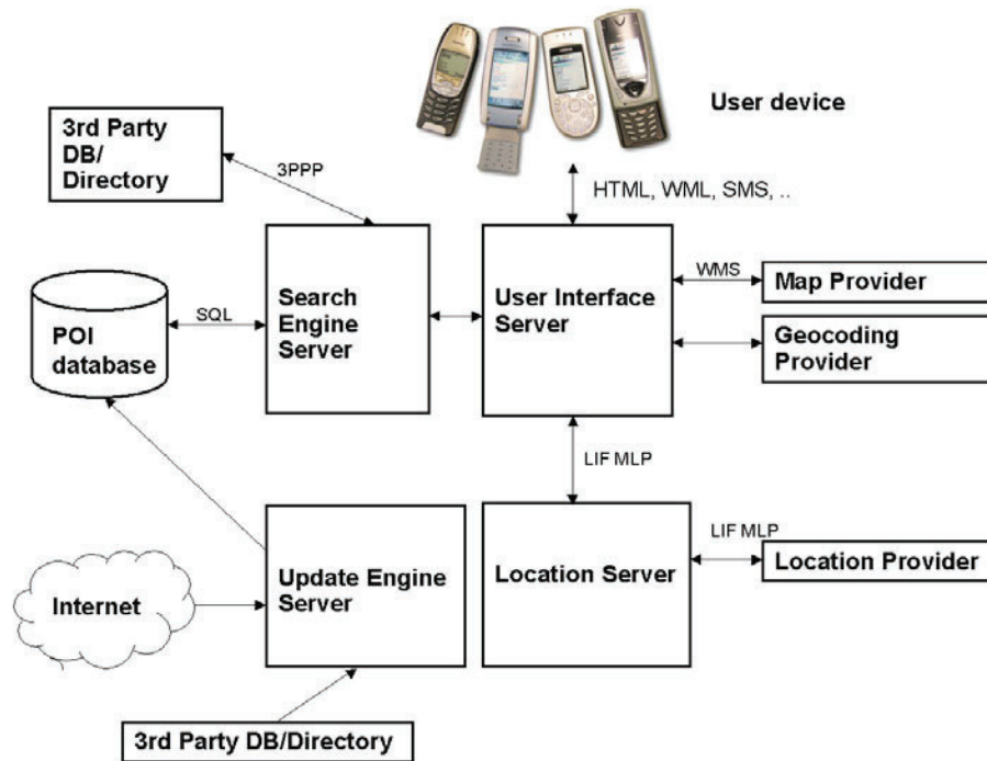
Figure 26. Architecture of NAVISearch location-aware integrated directory service.
