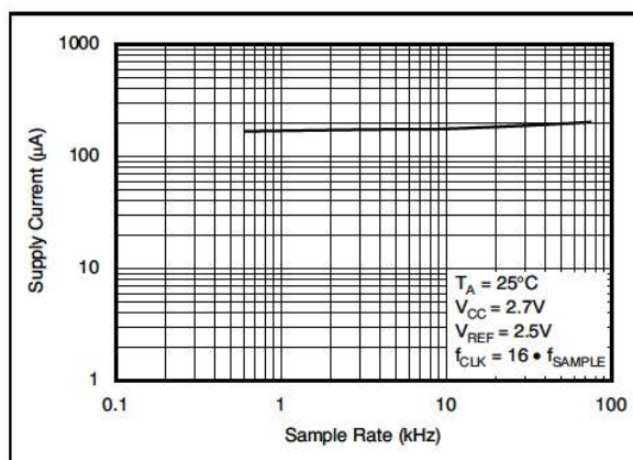
Figure 25. Scaling f_{CLK} Reduces the Supply Current Only Slightly with the Sample Rate
