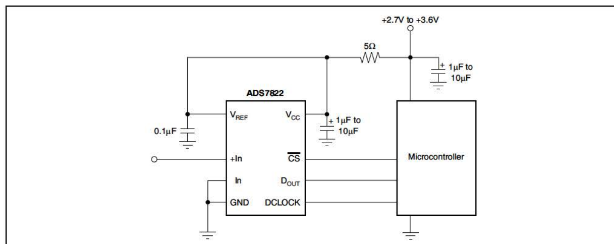
Figure 28. Basic Data Acquisition System
