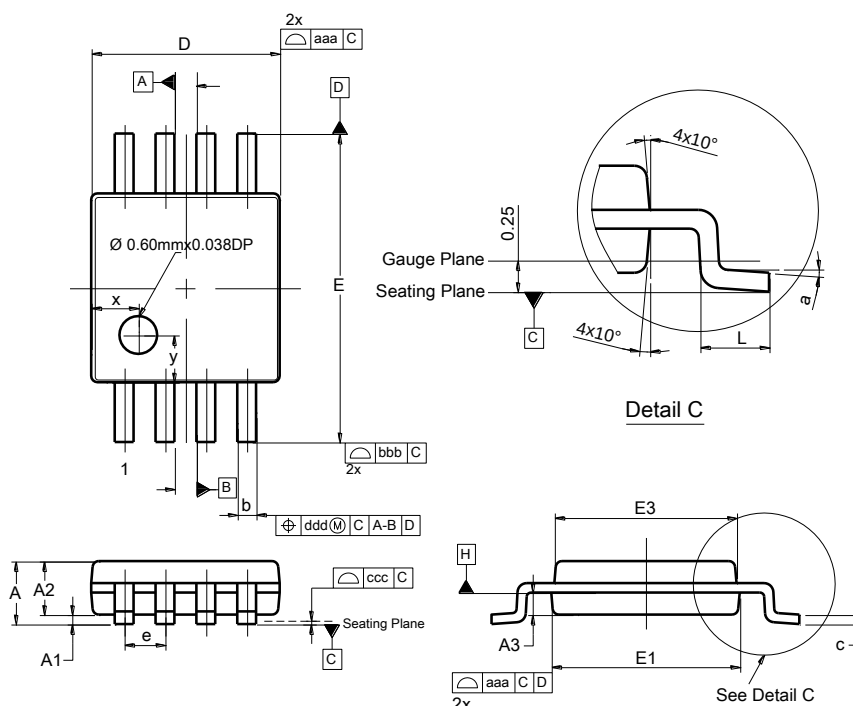
MSOP-8
