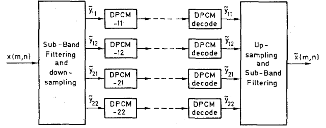
Fig. 9. A subband coding system with four bands.
