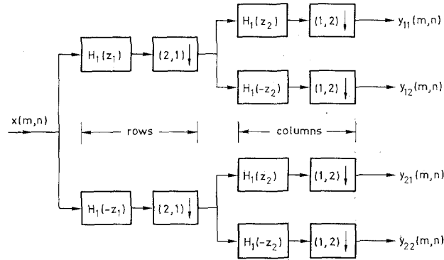
Fig. 7. Separable 4-subband filter.
