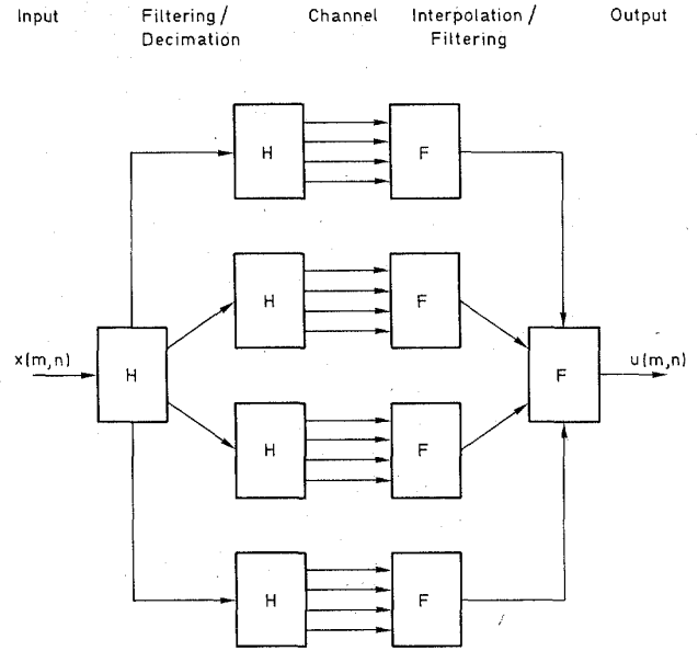
Fig. 3. System diagram of full 16-band system.
