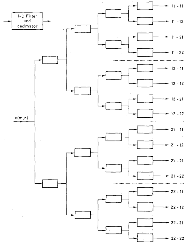
Fig. 8. Tree structure for 16-band separable subband filter.
