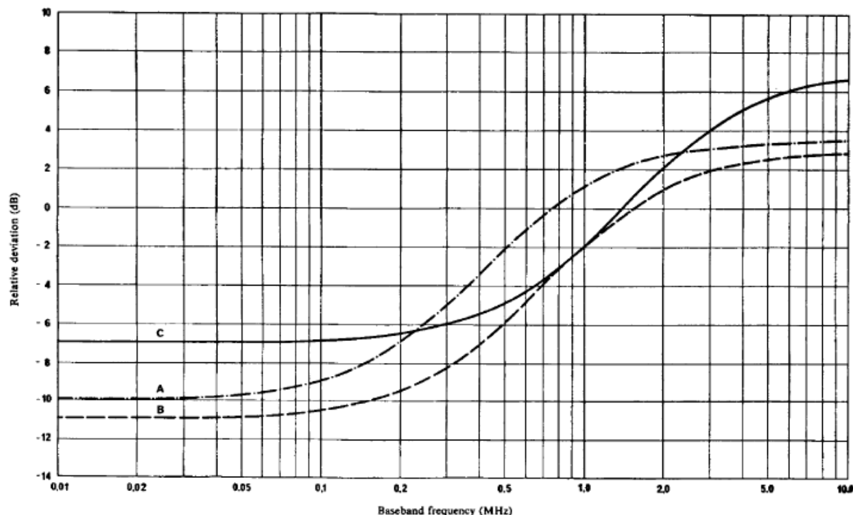
FIGURE 1 Pre-emphasis characteristic for television on 525-, 625-, and 819-line systems
