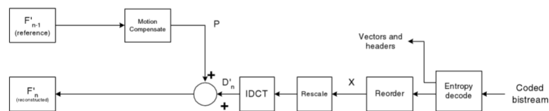
Figure 3.51 DPCM/DCT video decoder
