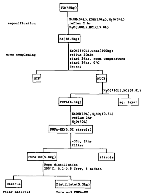
Fig. 1. Flow scheme for concentration of fatty acids in commercial oil by urea complexation, esterification and short-path wiped-wall distillation
