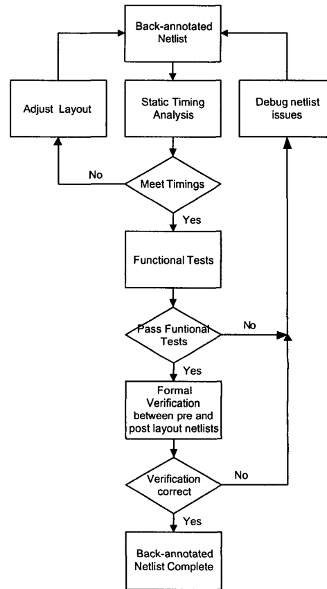
Figure 3. Layout to release flow
