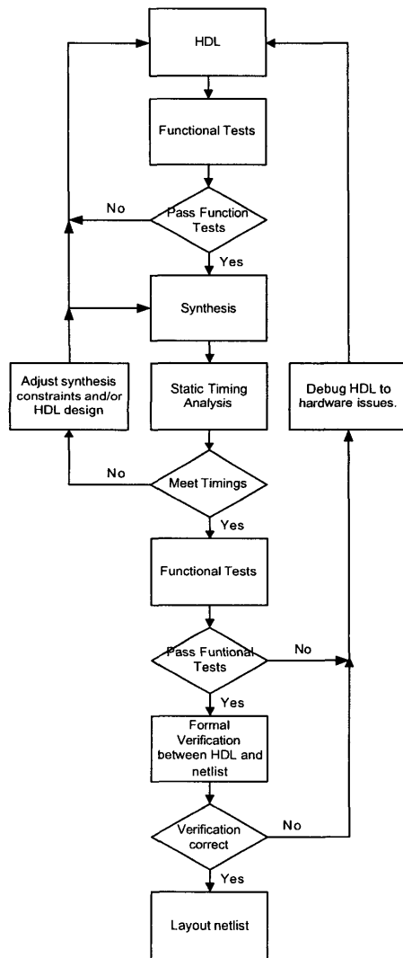
Figure 2. HDL to netlist flow.
