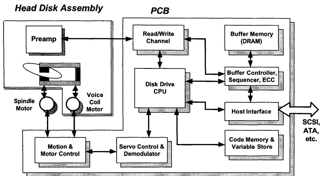
Figure 1. Hard disk drive subsystem
