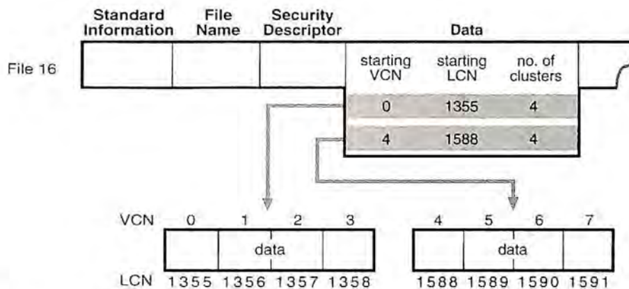
Figure 3-12. VCN-to-LCN Mappings for a Nonresident Data Attribute
