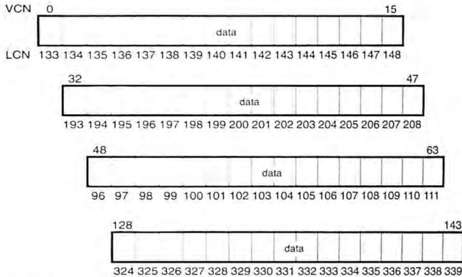
Figure 6-3. Runs of a Compressed Sparse File
