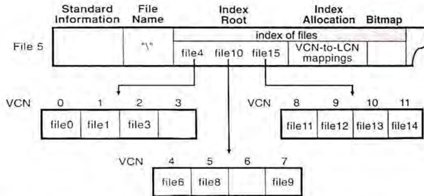
Figure 3-13. File Name Index for a Volume's Root Directory
