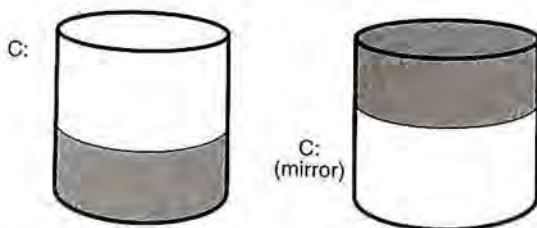
Figure 5-4. Mirror Set
