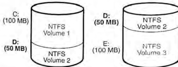
Figure 5-1. Volume Set
