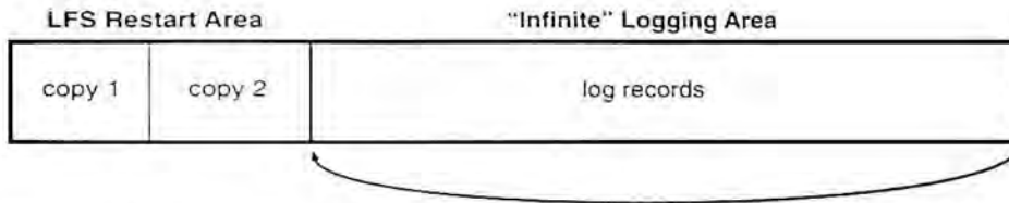
Figure 4-2. Log File
