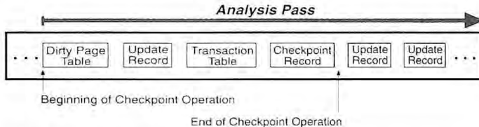
Figure 4-5. Analysis Pass
