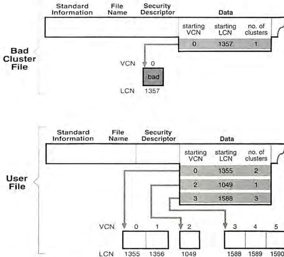
Figure 5-7. Bad-Cluster Remapping
