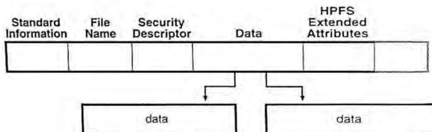
Figure 3-9. MFT File Record for a Large File with Two Data Runs
