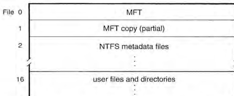
Figure 3-3. NTFS Metadata and User File Records in the MFT
