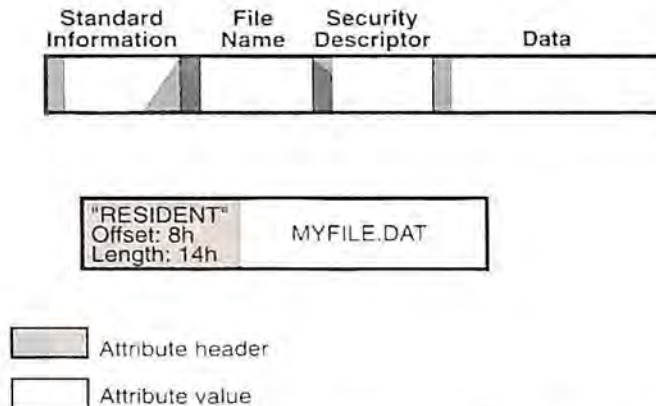
Figure 3-7. Resident Attribute Header and Value
