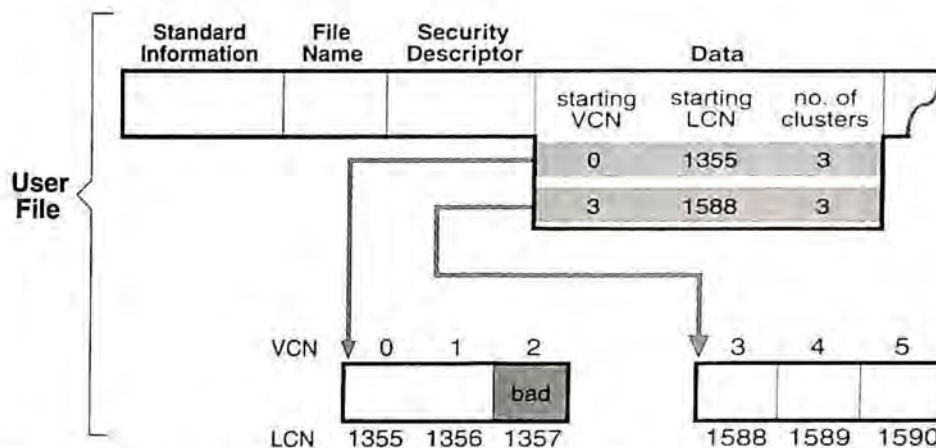
Figure 5-6. MFT Record for a User File with a Bad Cluster
