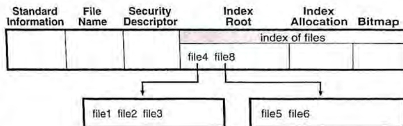
Figure 3-10. MFT File Record for a Large Directory with a Nonresident File Name Index
