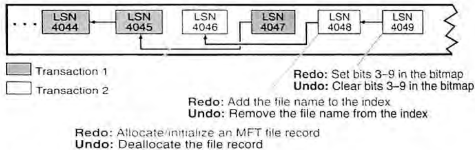
Figure 4-8. Undoing a Transaction
