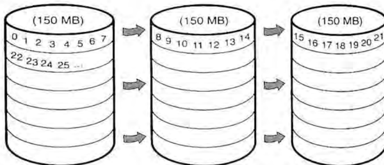
Figure 5-3. Logical Numbering of Physical Sectors on a Stripe Set
