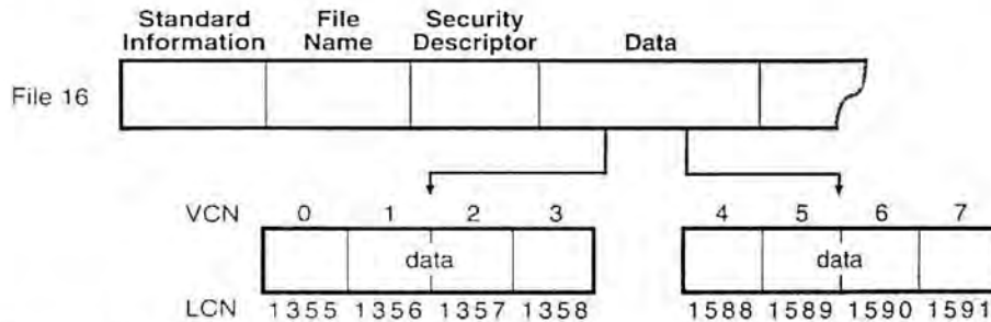
Figure 3-11. Virtual Cluster Numbers (VCNs) for a Nonresident Data Attribute
