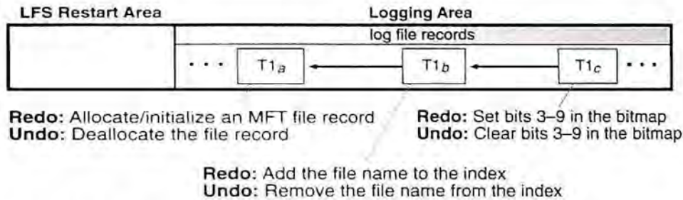
Figure 4-3. Update Records in the Log File
