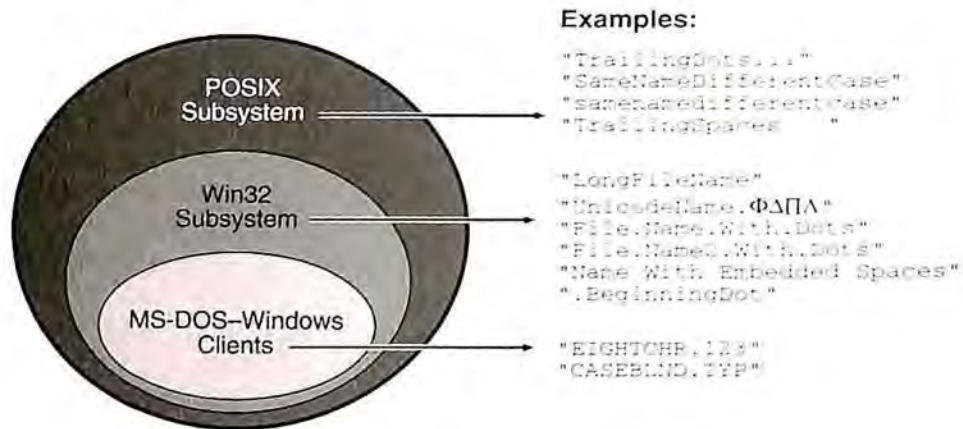
Figure 7-1. Windows NT File Namespaces
