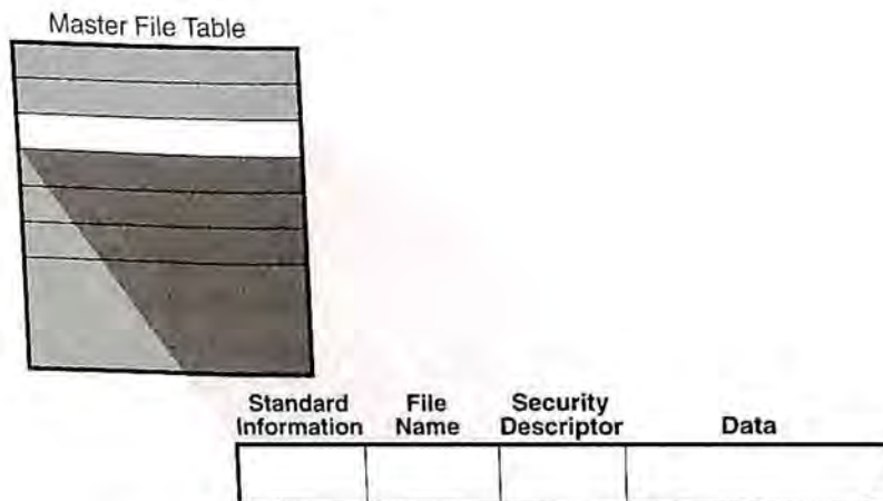
Figure 3-5. MFT Record for a Small File
