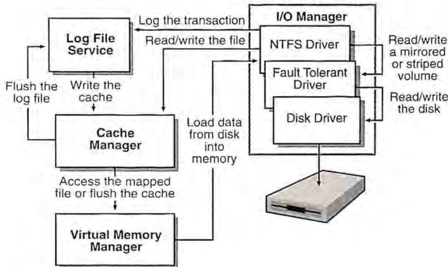
Figure 2-2. NTFS and Related NT Executive Components
