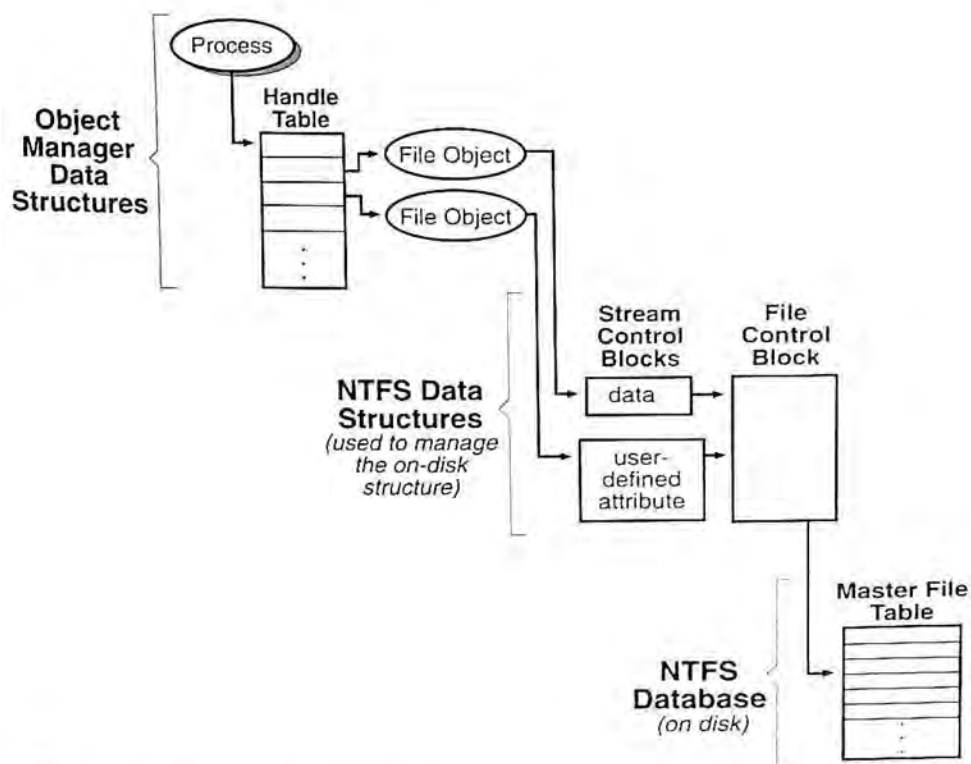
Figure 2-5. Locating an NTFS File
