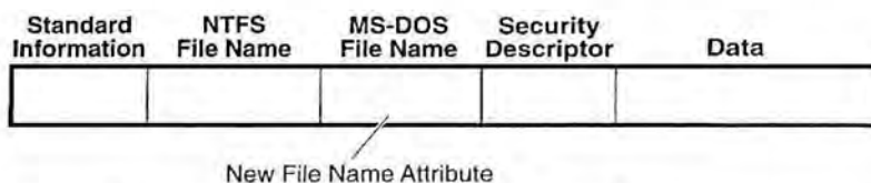
Figure 7-2. MFT File Record with an MS-DOS File Name Attribute
