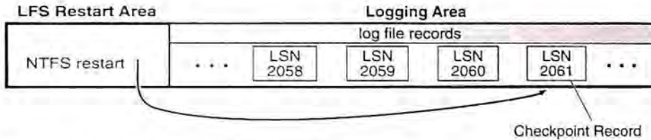
Figure 4-4. Checkpoint Record in the Log File
