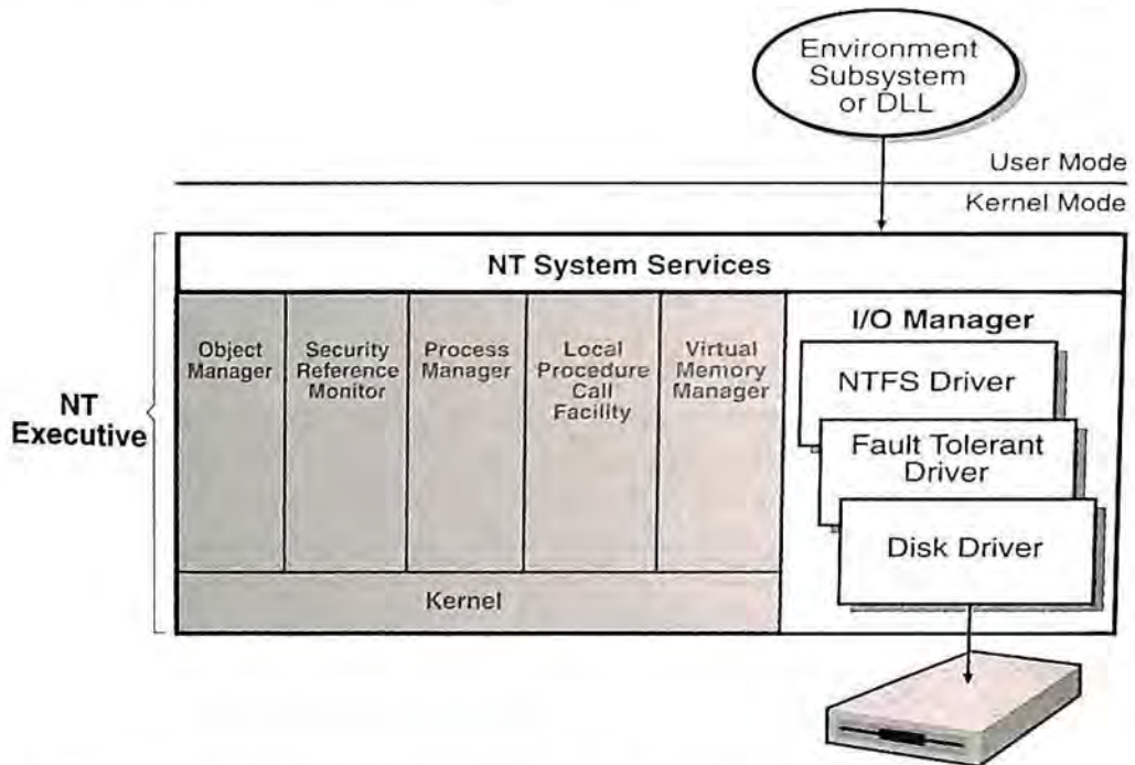
Figure 2-1. Components of the Windows NT I/O System
