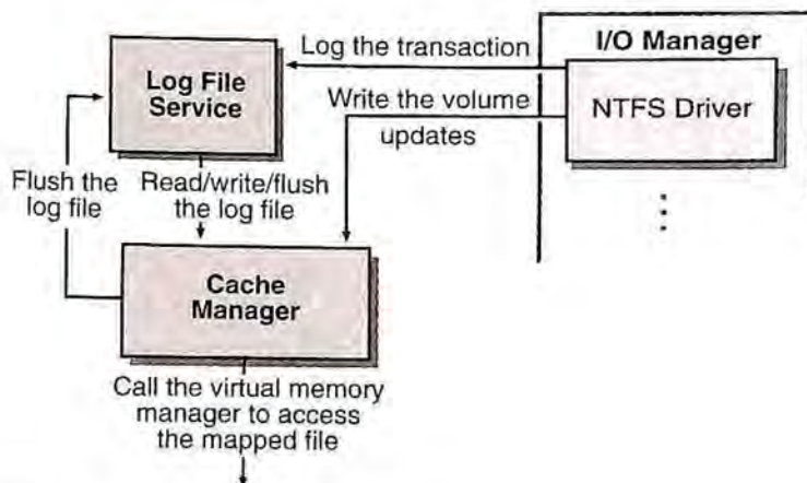
Figure 4-1. Log File Service (LFS)
