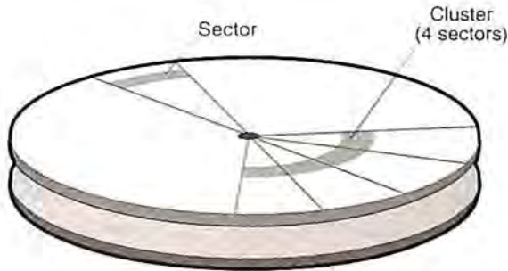
Figure 3-2. Sectors and a Cluster on a Disk
