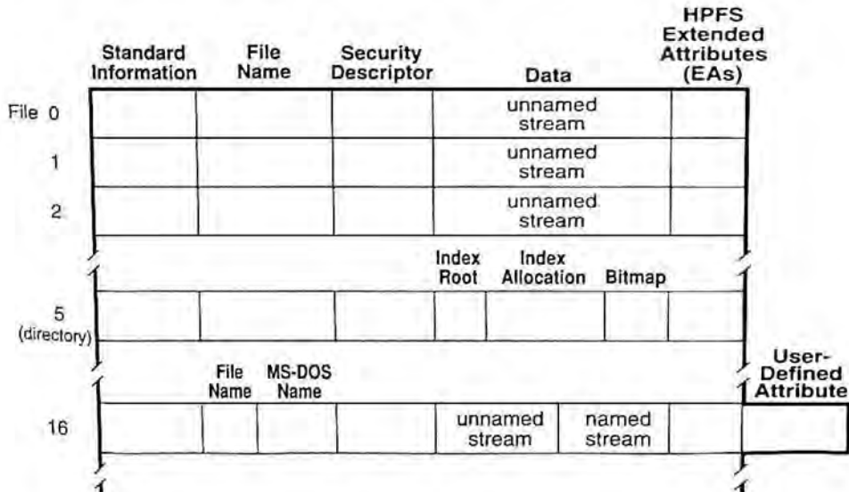
Figure 2-4. Adding Attributes and a Data Stream to an MFT Record
