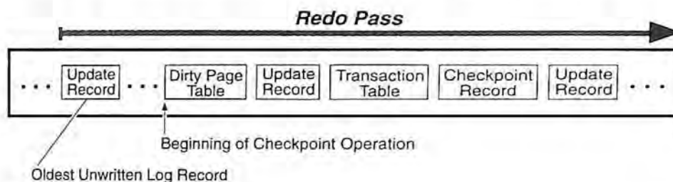
Figure 4-6. Redo Pass
