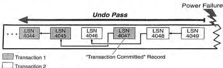
Figure 4-7. Undo Pass
