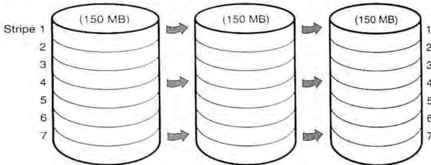
Figure 5-2. Stripe Set
