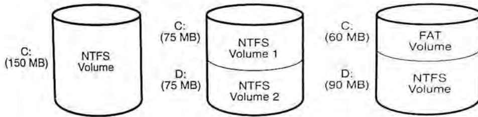
Figure 3-1. Sample Disk Configurations
