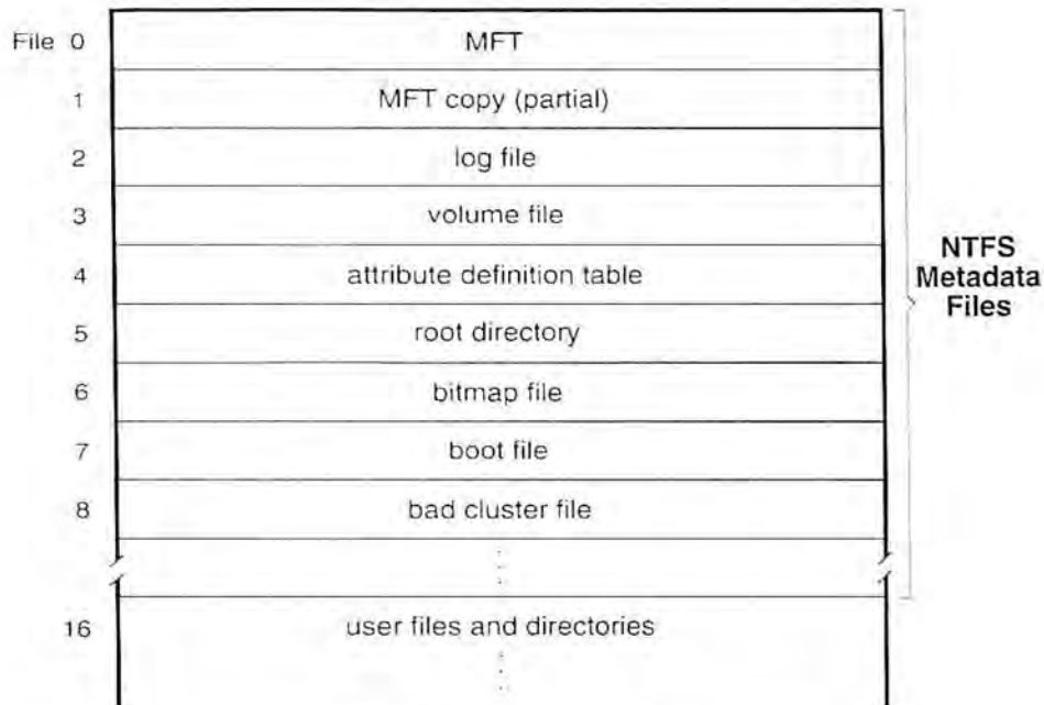
Figure 3-14. File Records for NTFS Metadata Files in the MFT
