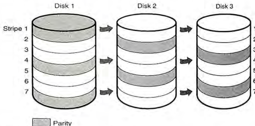
Figure 5-5. Stripe Set with Parity
