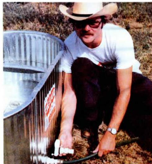
Free-Flo valve sells for $6.95 and mounts in sidewall or bottom of the tank. It automatically maintains a constant water level by sensing weight of the water column.
