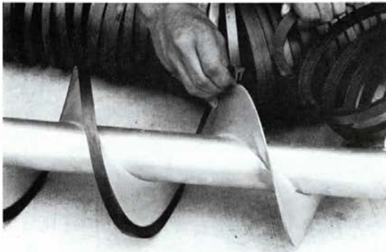
Nylatron wear strip comes already coiled and preformed to easily snap onto augers.
