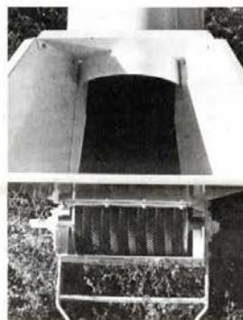
12-in. belt moves grain without breaking or cracking the kernels. Biggest use is for granular fertilizer.
