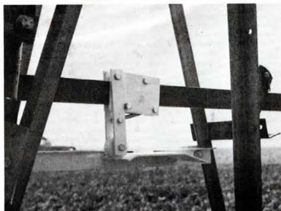
Closeup shows roller and ramp which lift the trojan bar so it won't drag over the wheel lug, causing excessive wear.
