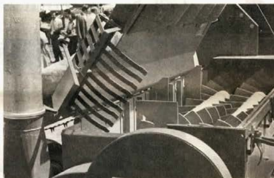
The JF straw processor requires about 70 pto hp and applies caustic soda solution as straw leaves the hammermill-type grinder. "Hard-mixing" occurs in the mixing chamber where liquid is rubbed into the straw by a beater-type mixer. Capacity is 2-2½ tons per hr. For more details, contact: FARM SHOW Followup, Terry Grace, Farmax, Box 8523, Mobile, Ala. 36608 (ph. 205 479-8663).
