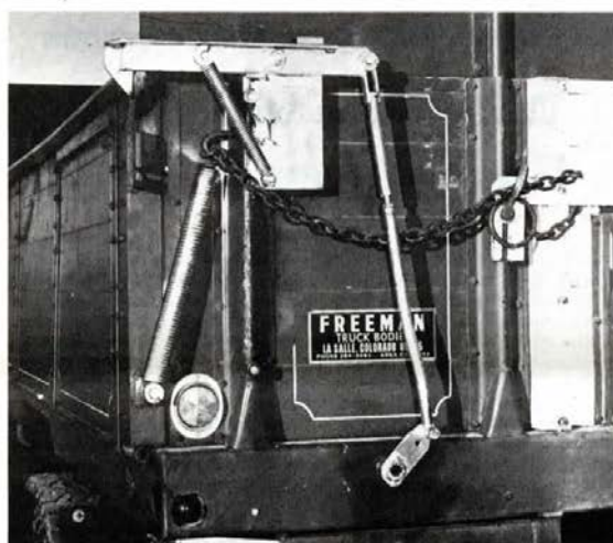
Electrically-controlled, hydraulically operated sideboard swings freely and can be closed any time while moving. Automatic latching system adapts to all makes of side-dump boxes.
