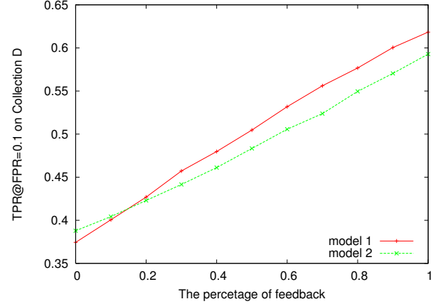
Figure 6: The true-positive rates at 0.1 false-positive rate of two user models when the feedback is limited. Model 1 assumes all uncaught spam messages are reported; model 2 includes a correction term that estimates the count of unreported junk mail messages.
