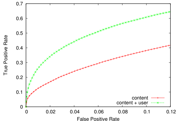
Figure 4: The ROC curves of the content-based filter and the model that incorporates user preferences.
