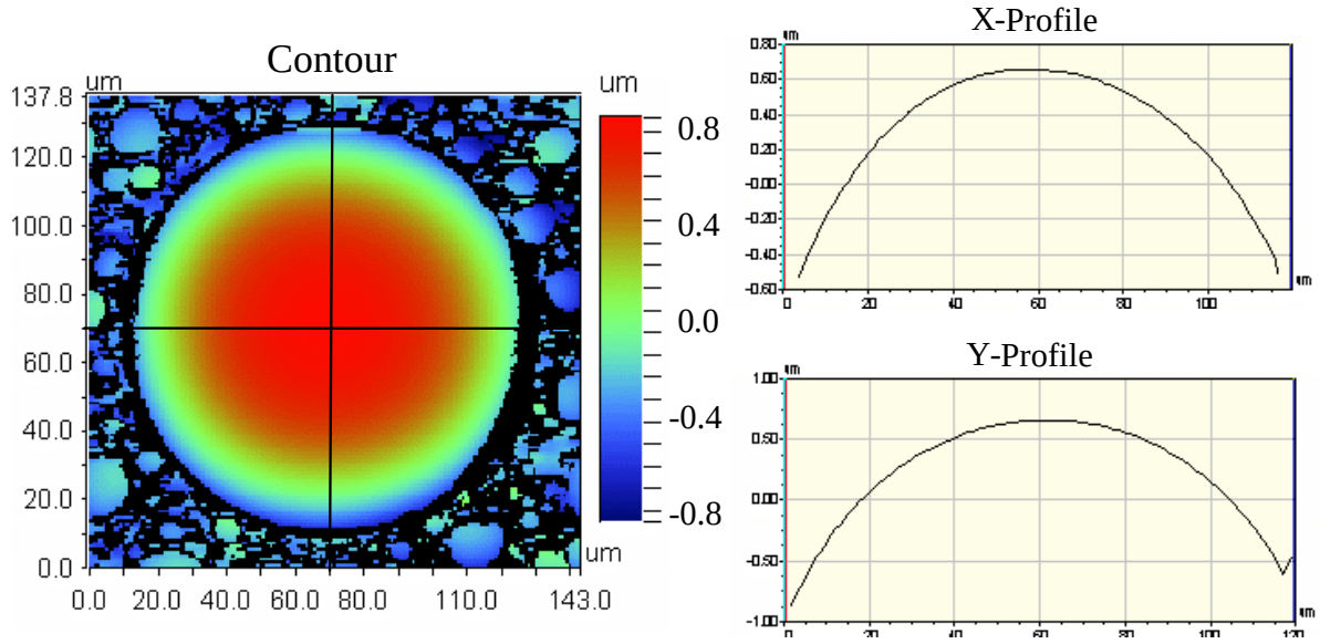
Figure 9: Typical interferometric endface analysis of fiber tip
