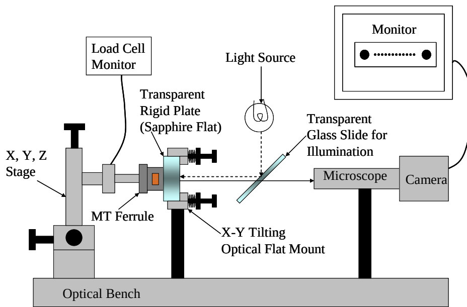
Figure 10: Apparatus for measuring fiber tip deflection vs. reaction force
