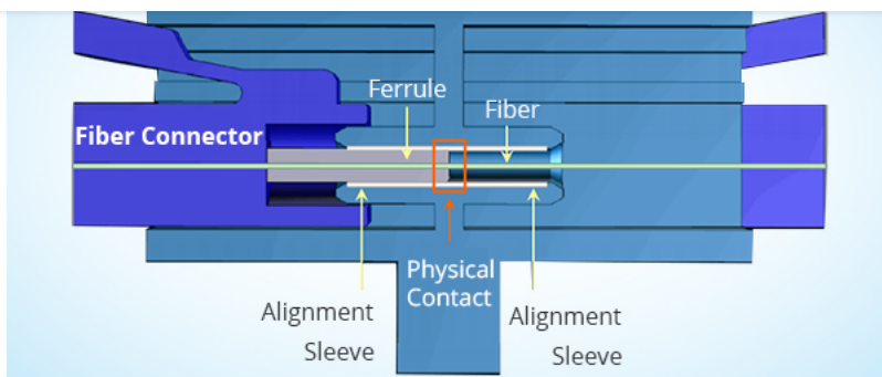
Figure 2: The Working Principle of Fiber Optic Adapter
