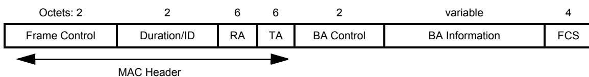
Figure 7-15—BlockAck frame
