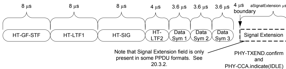
Figure 20-19—Packet alignment example (HT-greenfield format packet with short GI)
