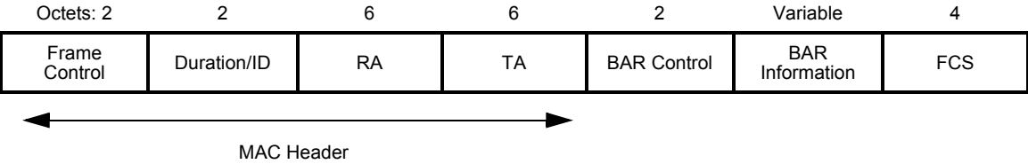
Figure 7-12—BlockAckReq frame
