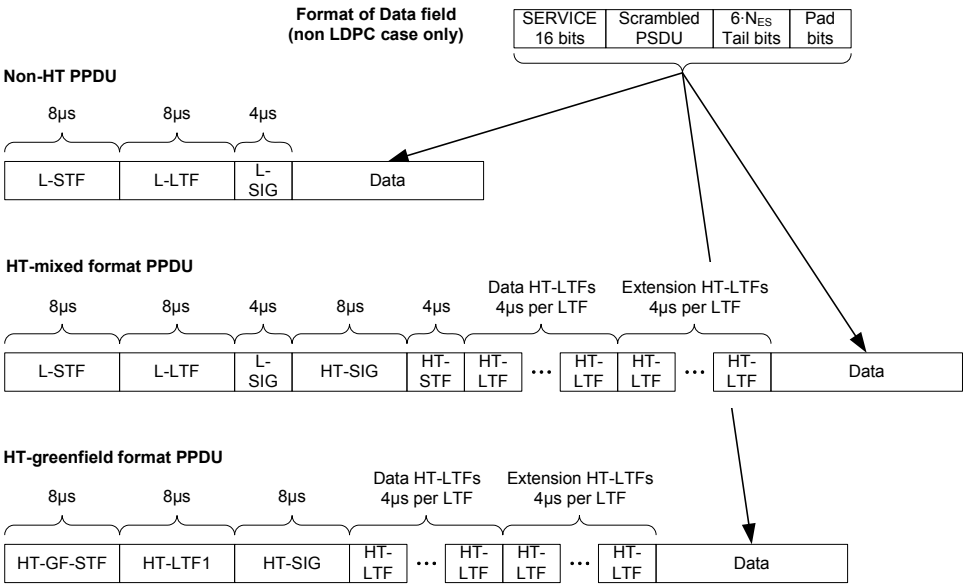
Figure 20-1—PPDU format
