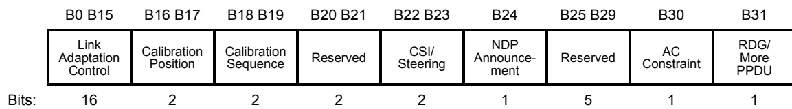
Figure 7-4a—HT Control field
