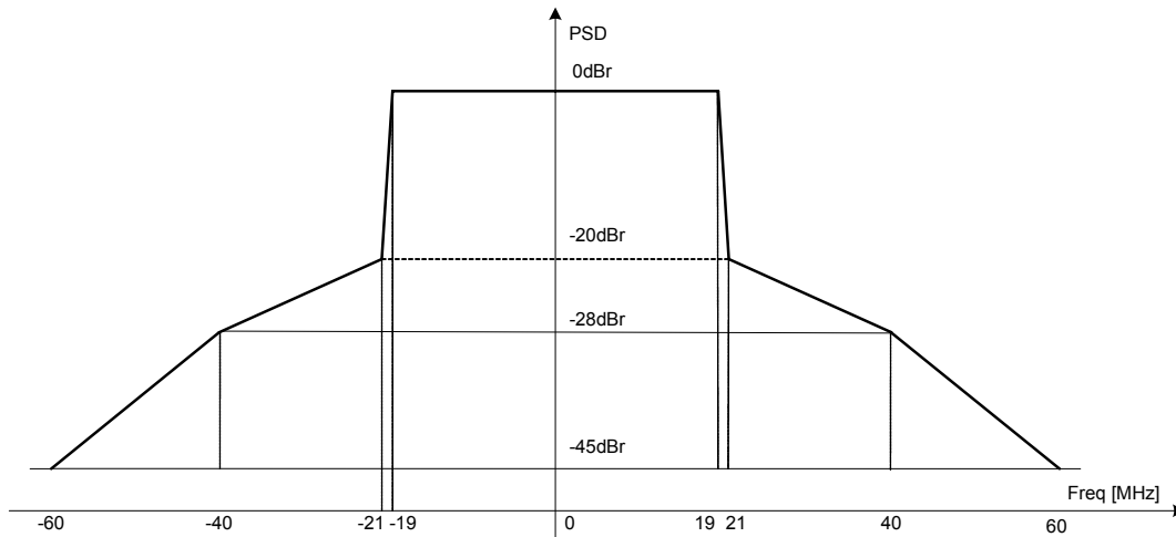
Figure 20-18—Transmit spectral mask for a 40 MHz channel
