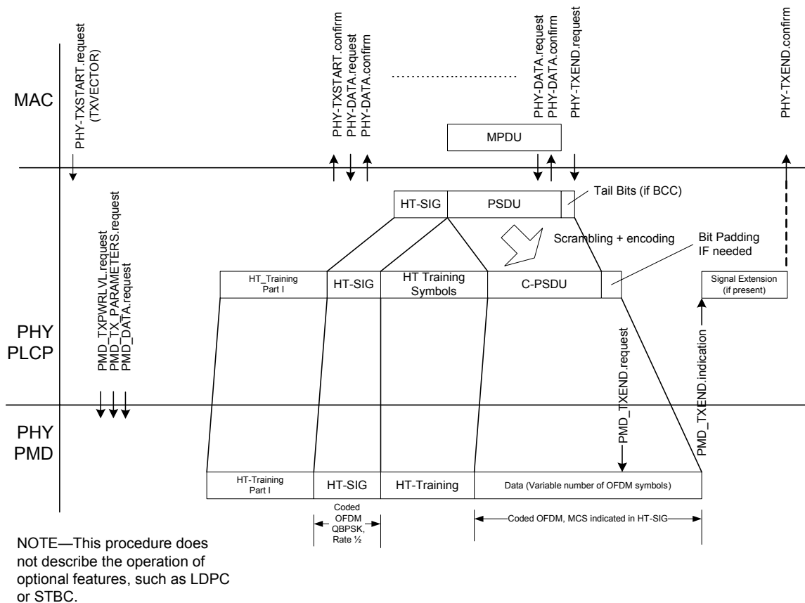
Figure 20-21—PLCP transmit procedure (HT-greenfield format PDU)
