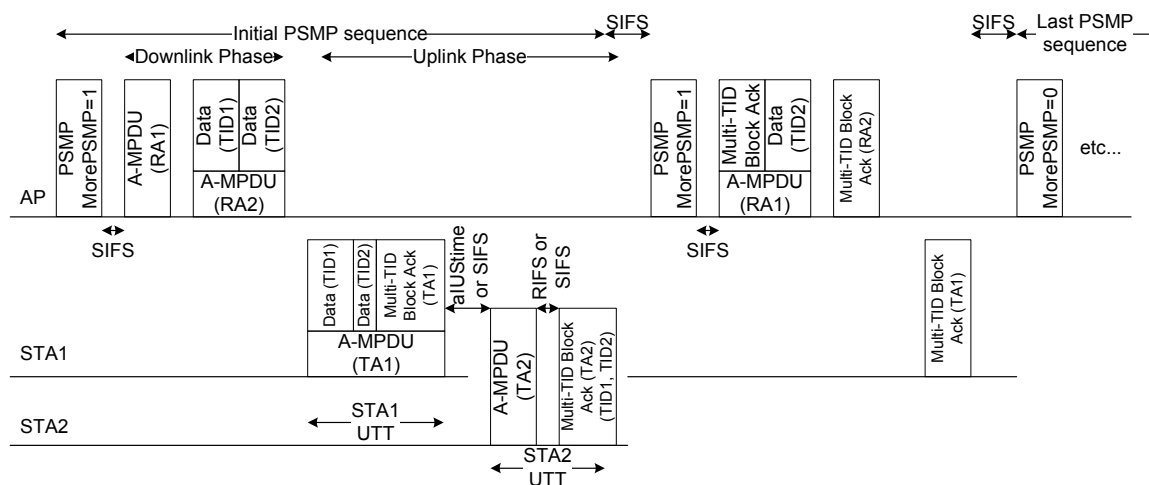
Figure 9-28—PSMP burst
