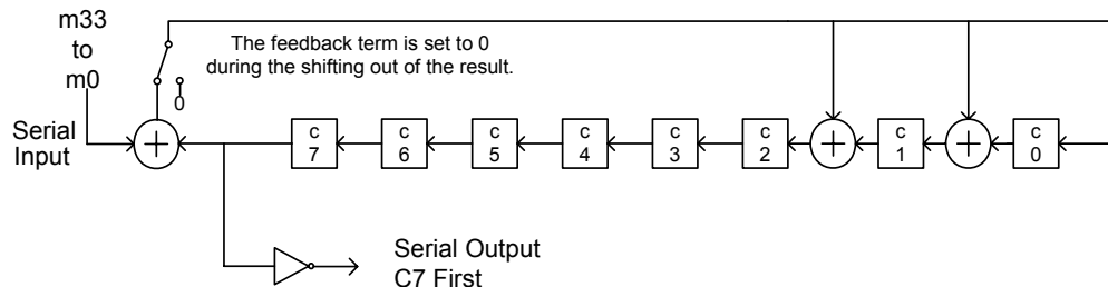
Figure 20-8—HT-SIG CRC calculation
