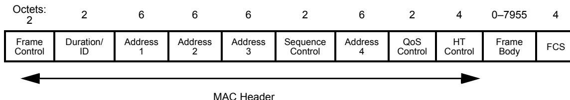
Figure 7-17—Data frame
