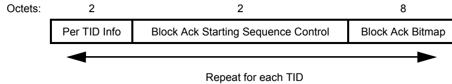
Figure 7-16c—BA Information field (Multi-TID BlockAck)
