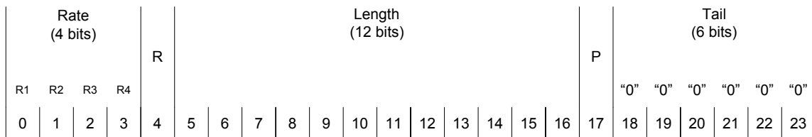
Figure 20-5—L-SIG structure
