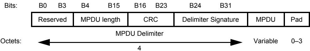
Figure 7-101p—A-MPDU subframe format
