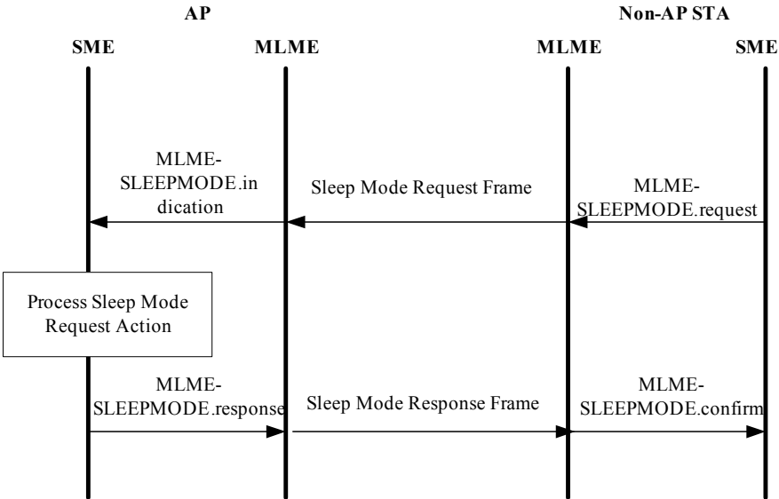
Figure 10-6o—Sleep Mode Request and Response Exchange
