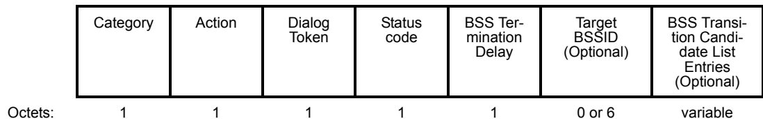
Figure 7-101n12— BSS Transition Management Response frame body format
