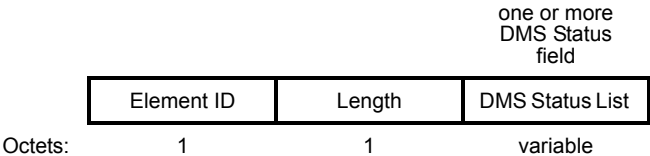
Figure 7-95o114—DMS Response element format
