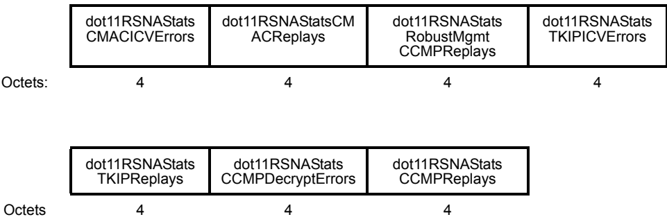
Figure 7-68l1—Measurement Report field format for RSNA Counters Group
