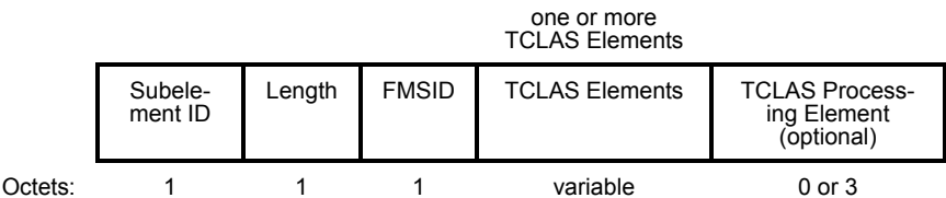
Figure 7-95o97—TCLAS Status Subelement format
