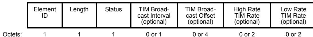
Figure 7-95o107—TIM Broadcast Response element format
