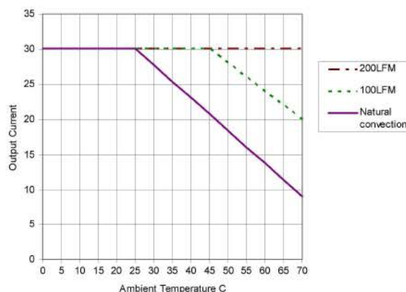
Derating @ 54VDC Input
