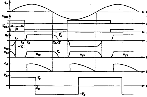
Fig. 11. Key waveforms for Series-SRLS resonant converter.
