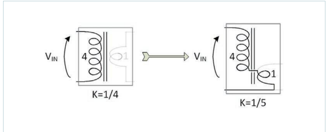
Figure 3 Comparison of volts-per-turn on magnetizing inductance in transformer and auto-transformer design
