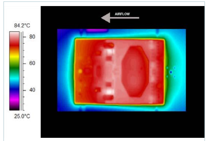
Figure 30 — Thermal plot, 600LFM, 25°C, 48V IN , 670W output power
