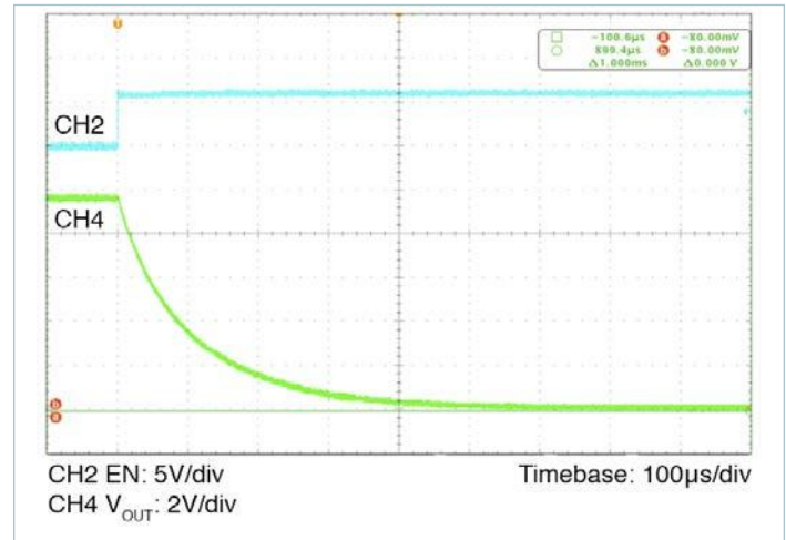
Figure 10 — Undershoot at turn off at nominal line, 15% load, 0 capacitance
