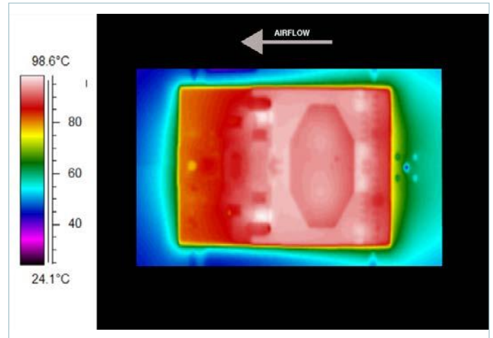
Figure 28 — Thermal plot, 400LFM, 25°C, 48V IN , 670W output power
