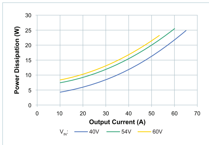
Figure 12 — Power dissipation at T_{CASE} = 85^{\circ}C
