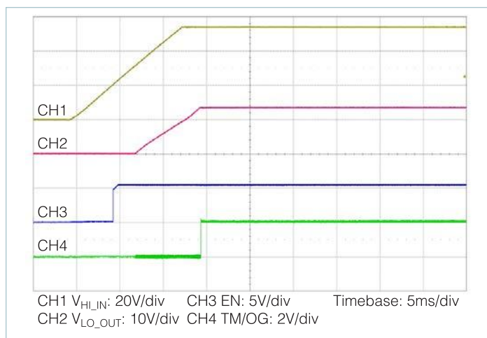
Figure 14 — Start up from application of V_{HI\_DC} = 54V , C_{LO\_OUT\_EXT} = 3000\mu F , no load; see start up description
