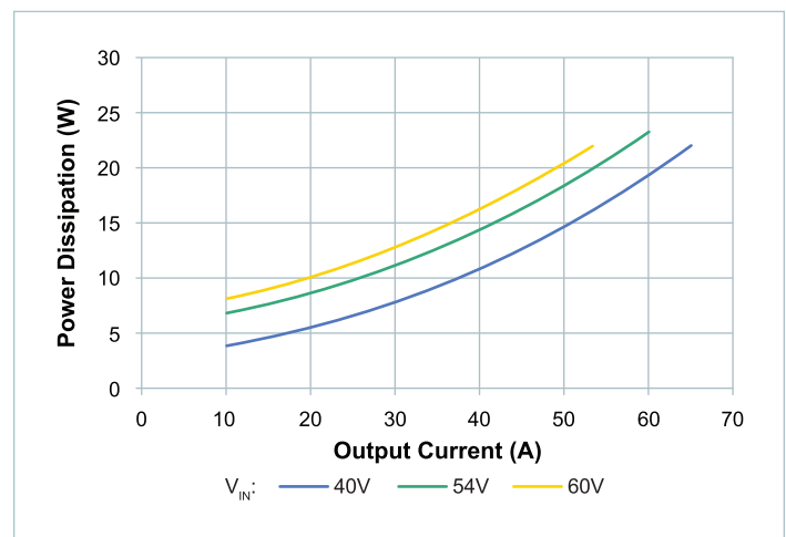
Figure 10 — Power dissipation at T_{CASE} = 25^{\circ}C
