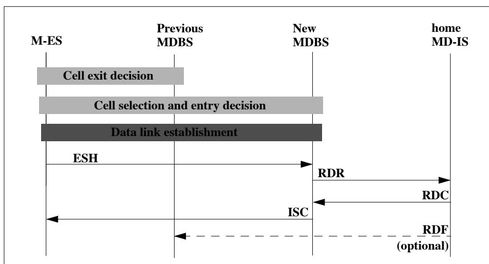
Figure 4.15: Inter-area Cell Transfer Protocol Events
