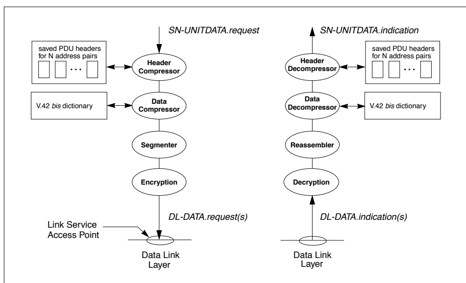
Figure 5.18: SNDCP Model for use of Acknowledged Data Link Services
