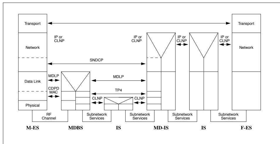
Figure 3.5: CDPD Example Interface Profiles for Network Services
