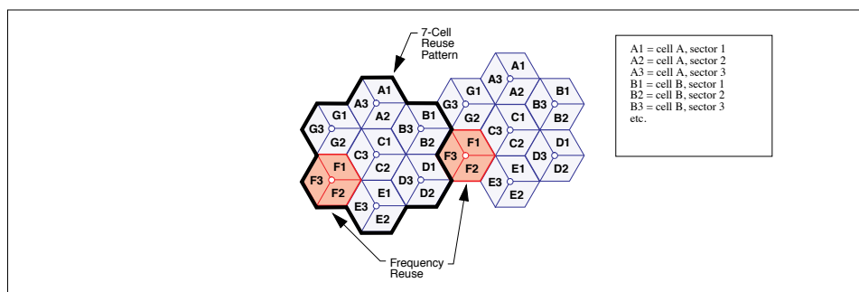
Figure 2.2: Frequency Reuse
