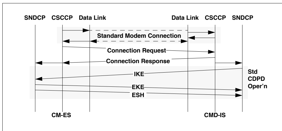
Figure 5.32: CM-ES Initial Connection
