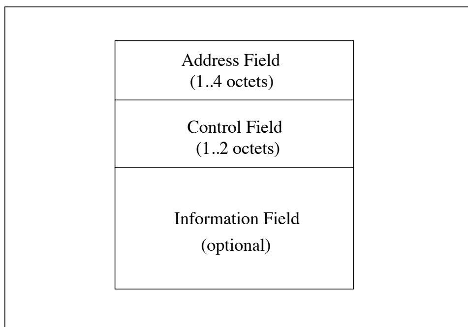
Figure 5.10: MDLP Frame Format
