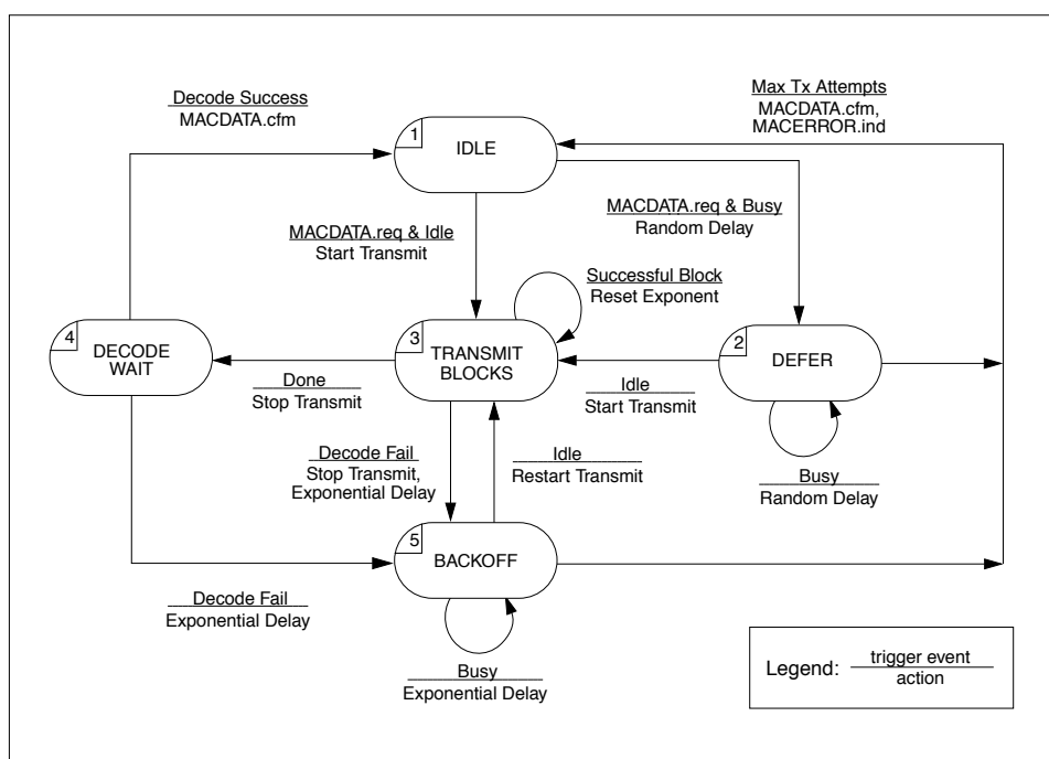
Figure 5.7: M-ES Procedure for Reverse Channel Access
