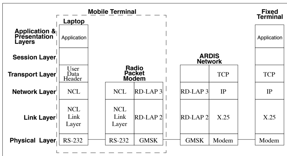
Figure 9.4: ARDIS Communications Architecture
