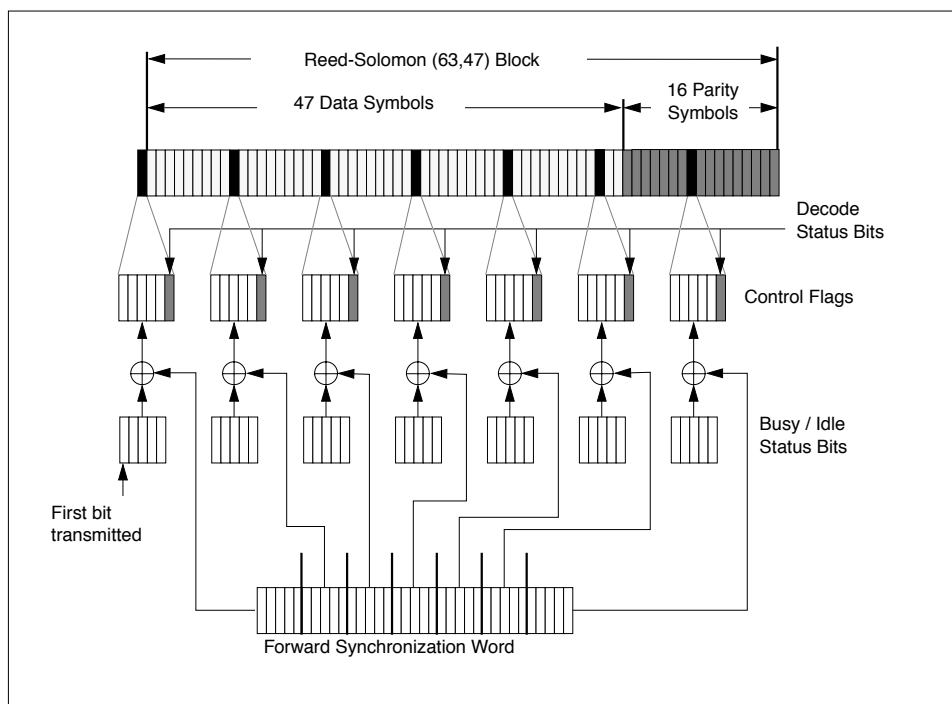
Figure 5.6: Forward Channel Transmission Structure
