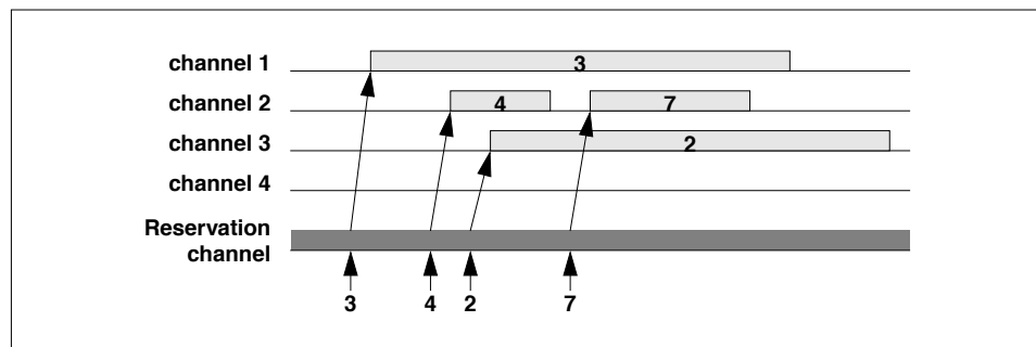
Figure 5.5: Frequency Based Demand Assigned with Reservation Example
