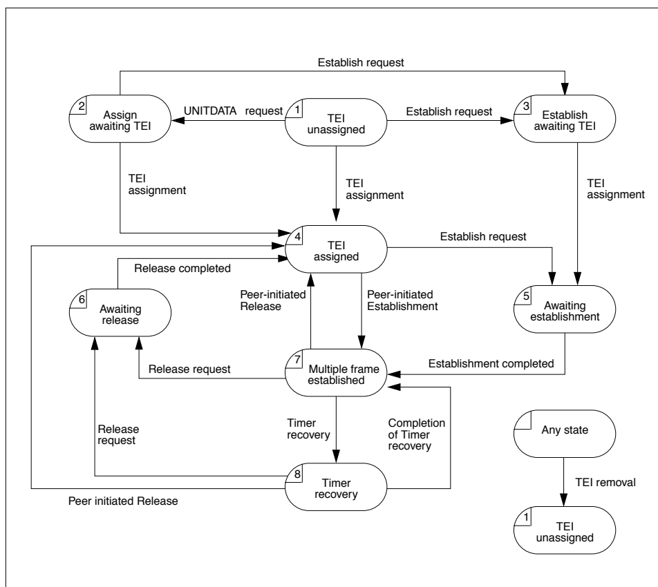
Figure 5.11: Overview of States of the Point-to-Point Procedures
