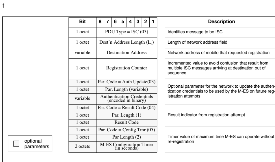
Figure 4.9: MD-IS Hello Confirm (ISC) Message Format
