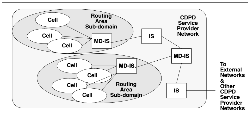
Figure 4.2: CDPD Network Routing Architecture
