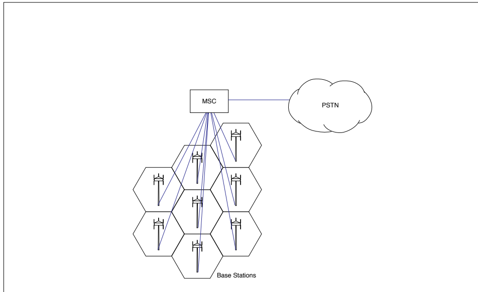
Figure 2.1: AMPS Architecture
