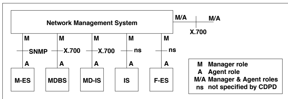
Figure 7.1: CDPD Network Management Model
