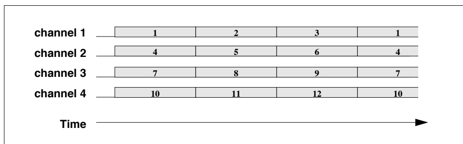
Figure 2.6: Time vs. Frequency for a TDMA System (e.g., IS-54/136)
