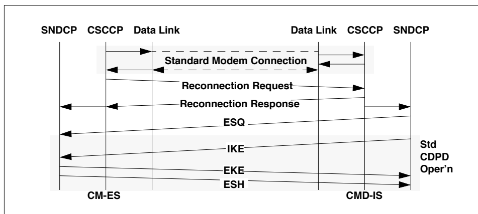
Figure 5.33: CM-ES Initiated Reconnection
