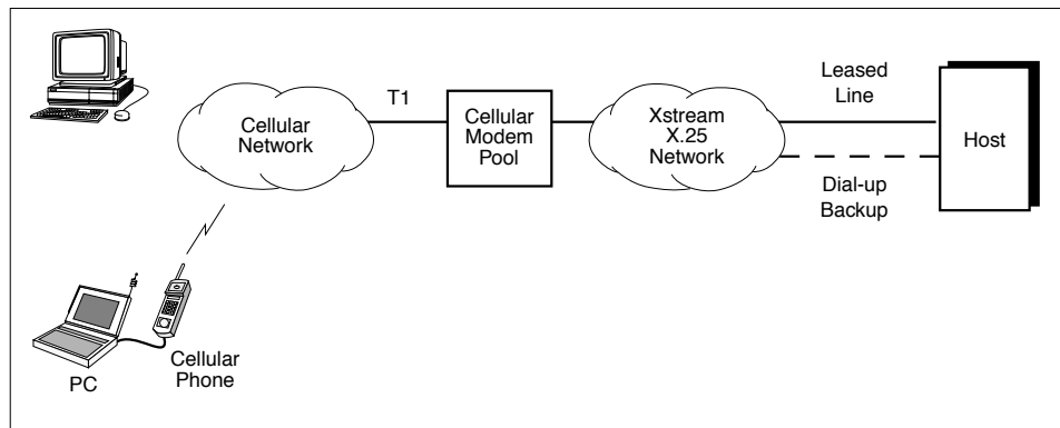
Figure 2.4: MCI's Xstream Air Network
