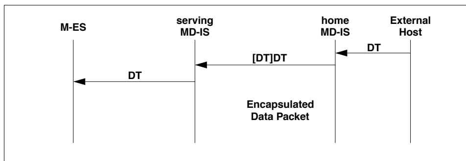
Figure 4.11: CDPD Data Routing
