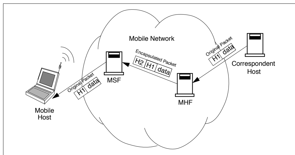
Figure 1.11: Packet Encapsulation in CDPD
