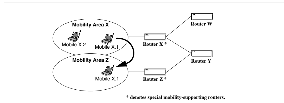
Figure 1.10: Embedded Network Scheme (ENS)
