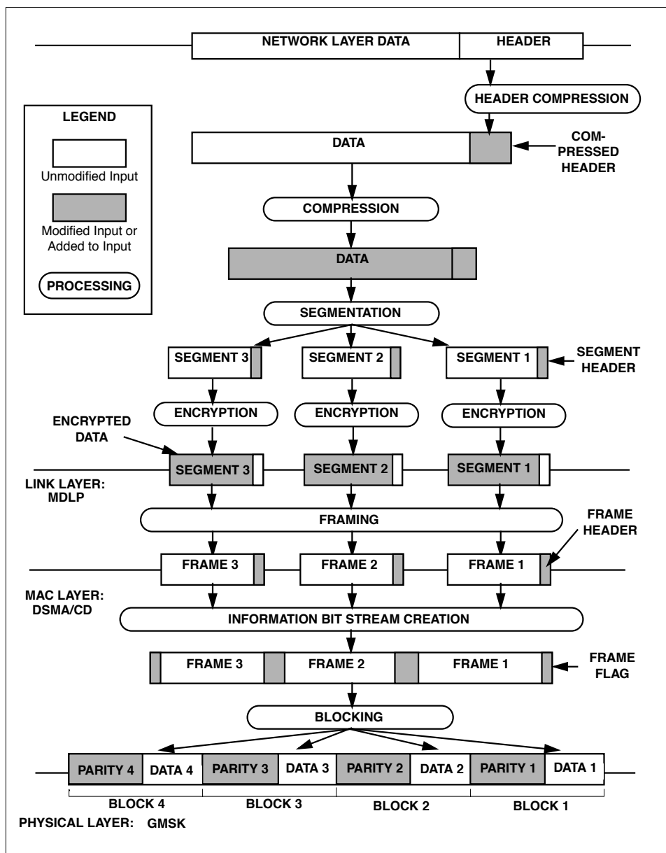
Figure 5.19: Packet Transformation Data Flow
