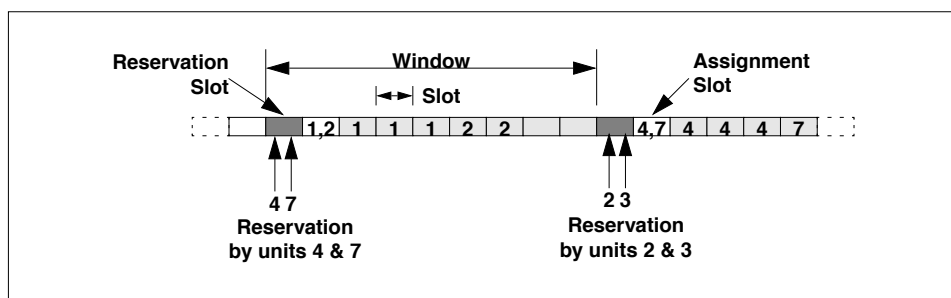
Figure 5.4: Time Based Demand Assigned with Reservation Example
