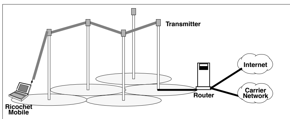
Figure 9.1: Metricom Ricochet
