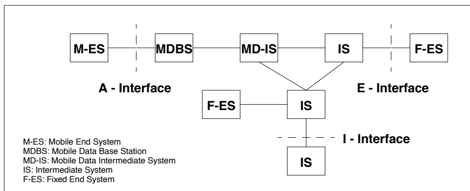
Figure 3.7: CDPD Reference Architecture
