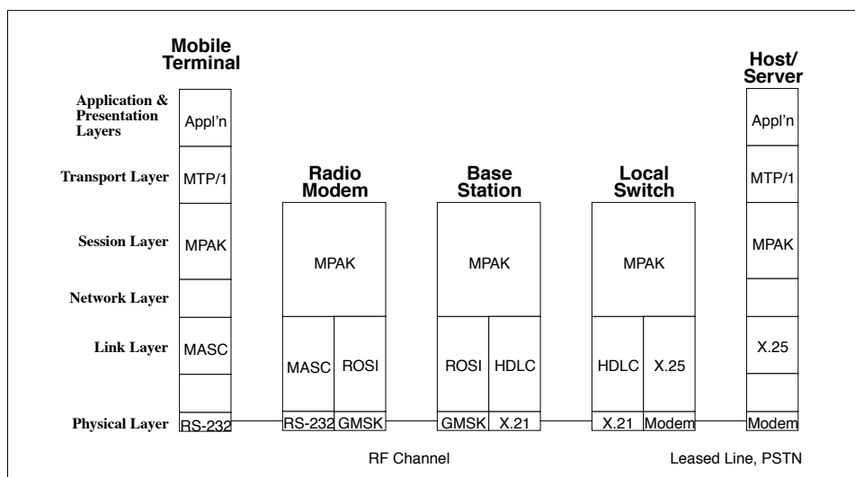
Figure 9.6: Mobitex Communications Architecture
