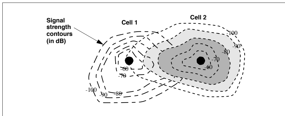
Figure 5.21: Example of Absolute Received Signal Strength Based Selection
