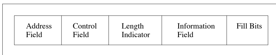
Figure 2.9: LAPDm Frame Format
