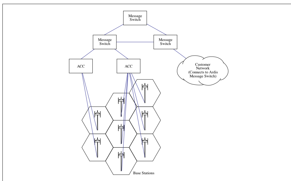
Figure 9.3: ARDIS Architecture
