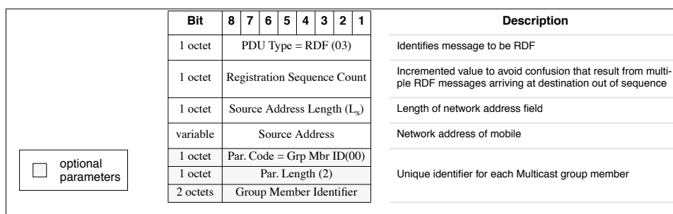
Figure 4.16: Redirect Flush (RDF) Message Format
