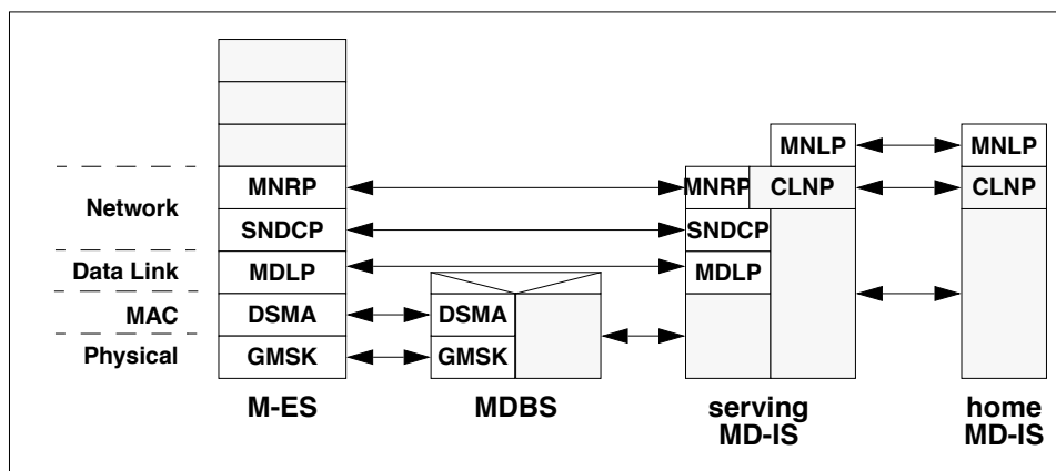
Figure 4.4: CDPD Support Protocol Architecture
