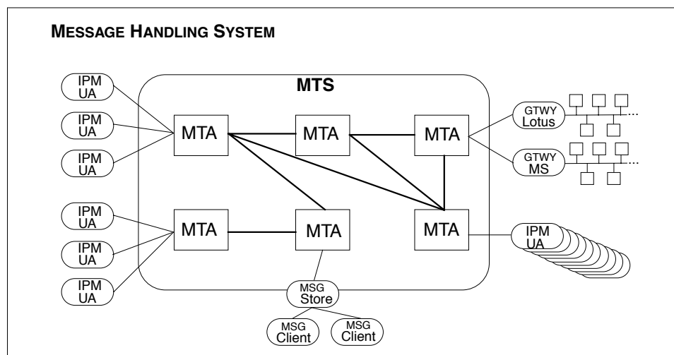
Figure 7.4: MHS Architecture
