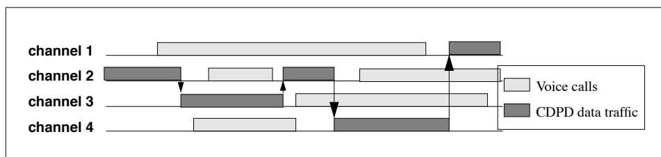
Figure 5.30: Channel Hopping example
