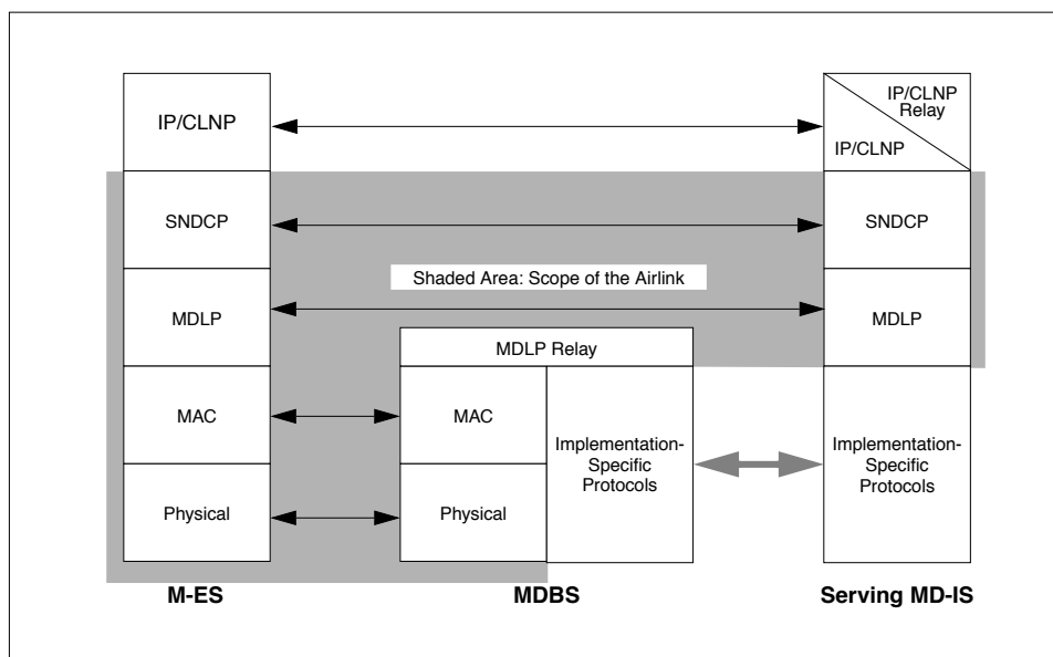
Figure 5.1: Airlink Protocol Profile
