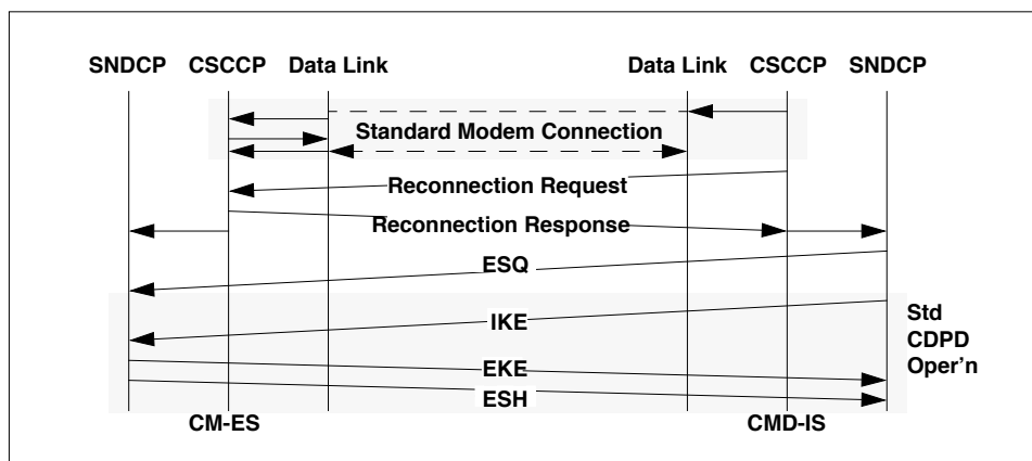
Figure 5.34: CMD-IS Initiated Reconnection
