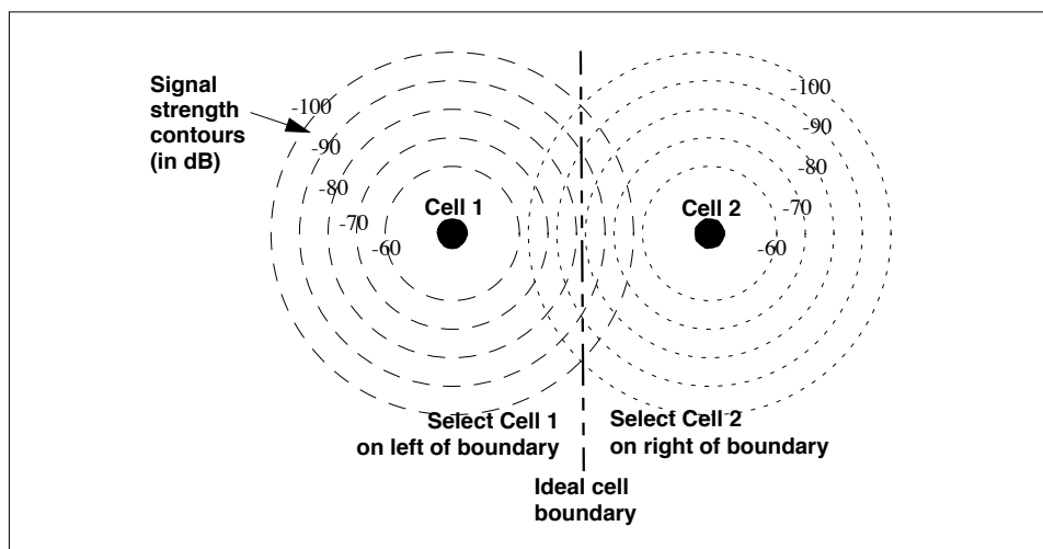
Figure 5.20: Theoretical Cell Selection
