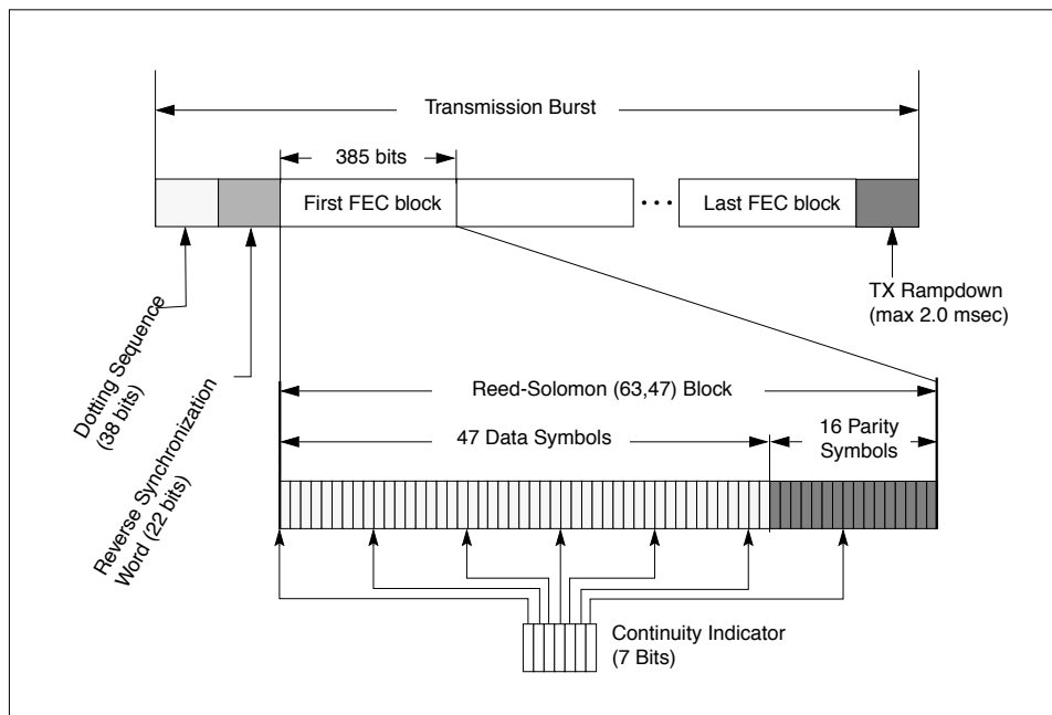
Figure 5.8: Reverse Channel Transmission Structure
