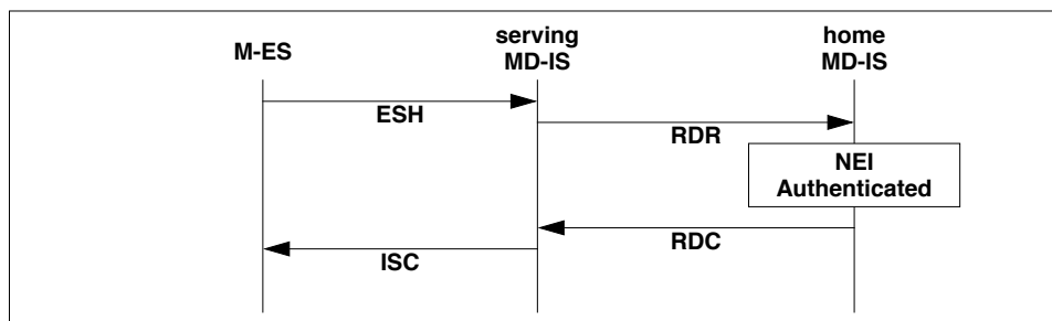
Figure 4.5: M-ES Registration
