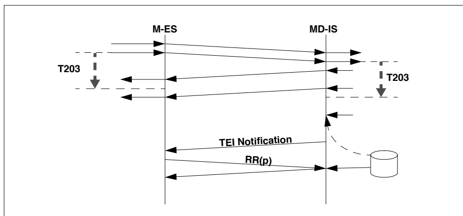
Figure 5.12: Sleep Mode Operation
