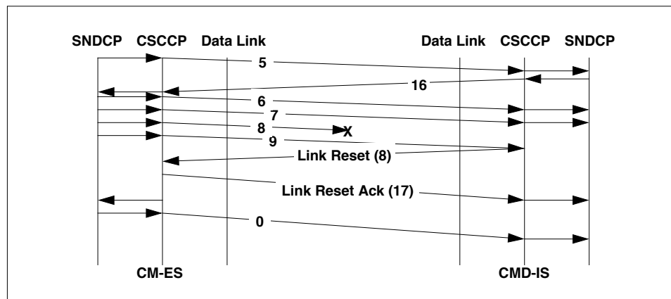
Figure 5.37: CSCCP Link Reset Procedure
