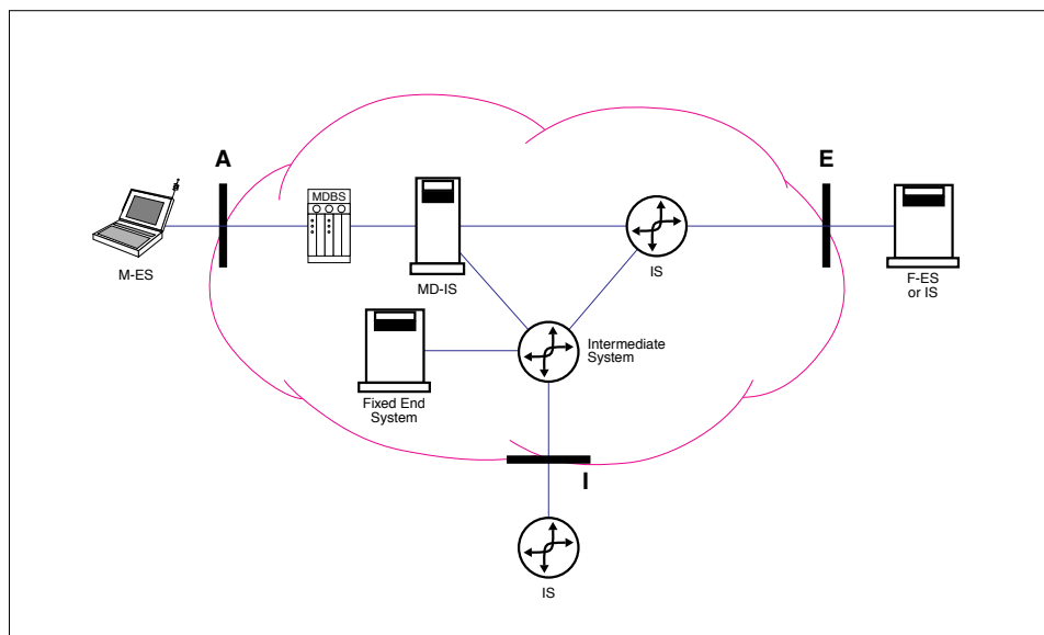
Figure 3.4: CDPD Network Layer Reference Model
