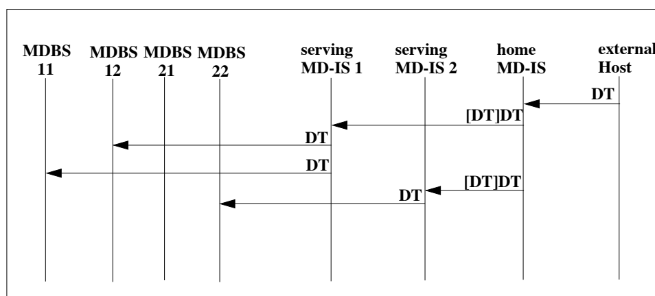
Figure 4.23: Multicast Data Redirection and Forwarding
