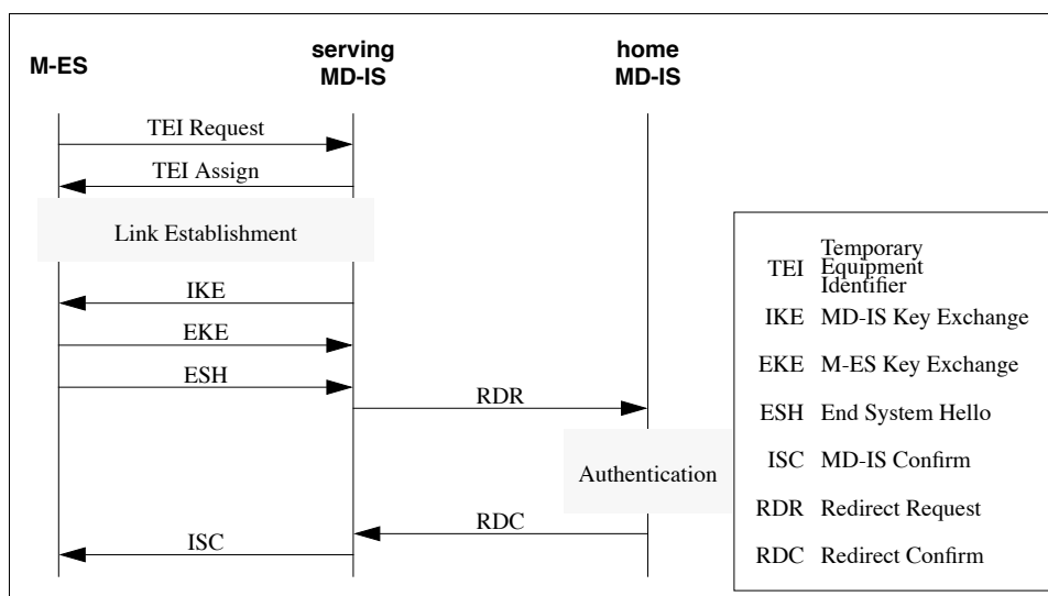
Figure 6.3: CDPD Security Protocol Events
