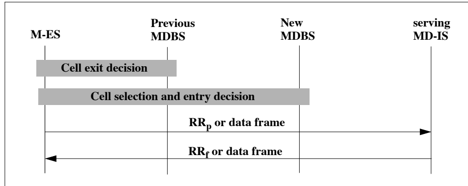
Figure 4.13: Intra-area Cell Transfer Protocol Events
