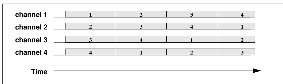
Figure 2.7: Time vs. Frequency for a FH-CDMA System
