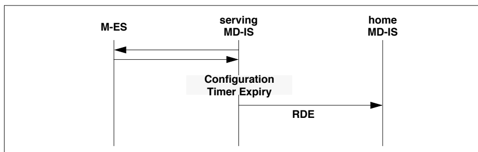
Figure 4.17: Configuration Timer Expiry Protocol Events
