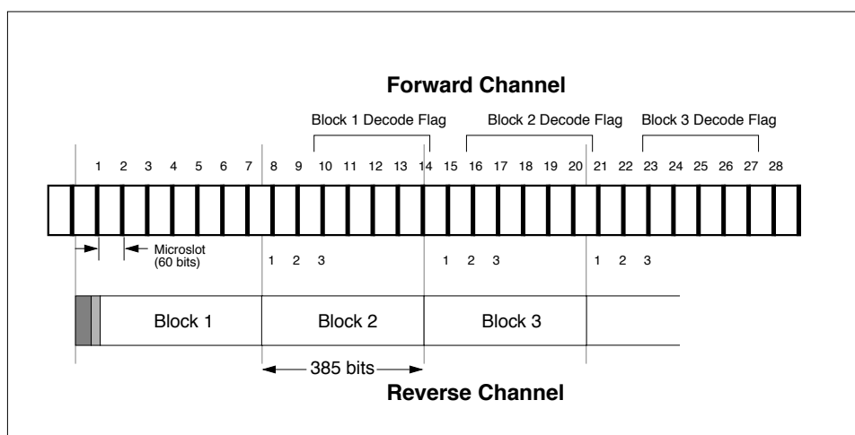
Figure 5.9: Decode Status Flag Timing Relationship
