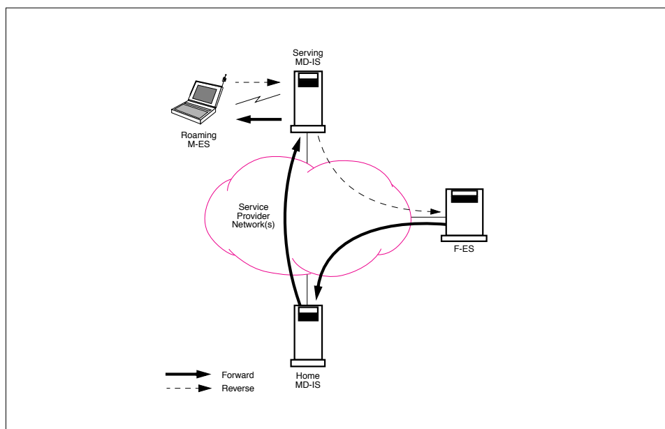
Figure 3.9: CDPD Traffic Flows
