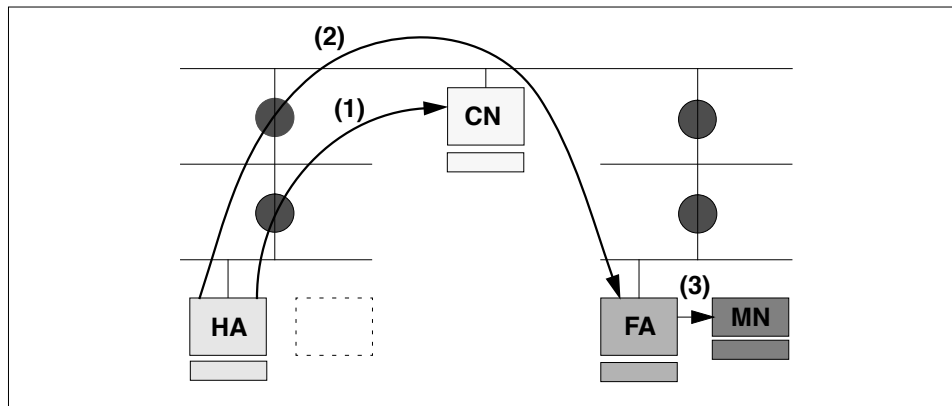
Figure 10.1: Mobile IP Routing to Mobile Node
