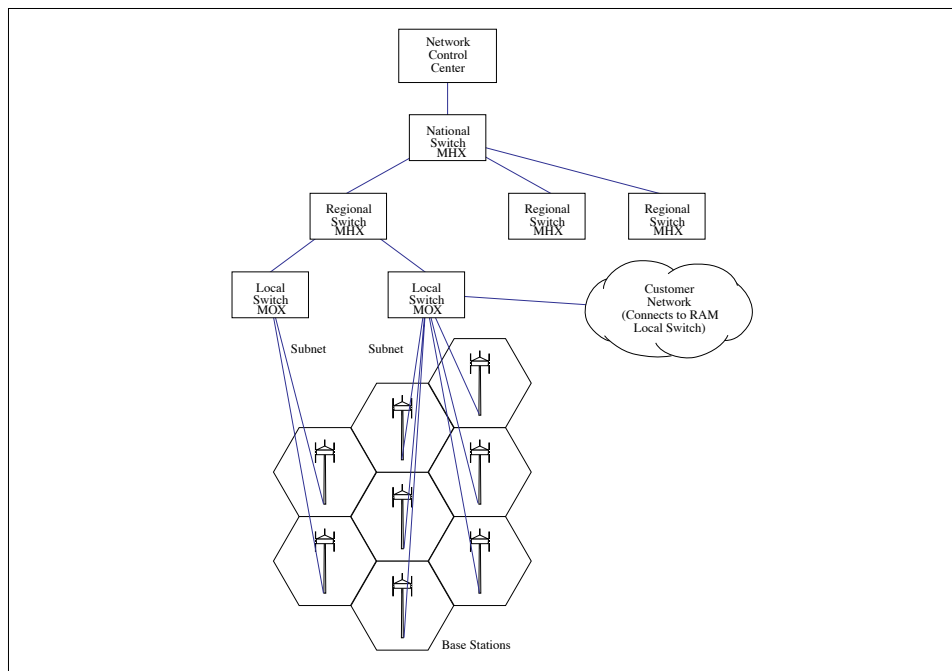
Figure 9.5: RAM Architecture
