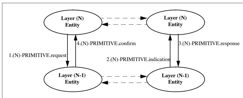
Figure 0.8: Layer (N) Protocol Primitives
