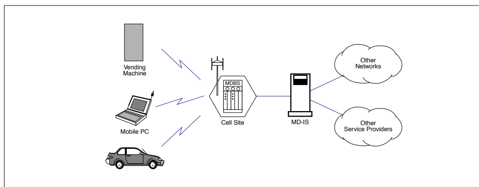
Figure 3.2: The CDPD System
