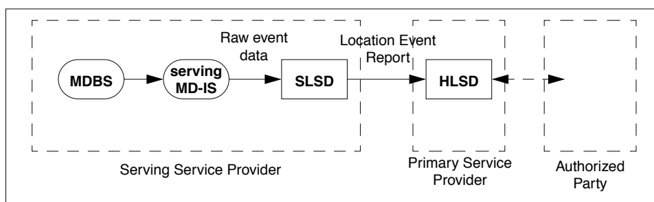
Figure 8.5: CDPD Subscriber Area Location Service
