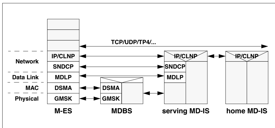
Figure 4.3: CDPD Protocol Architecture
