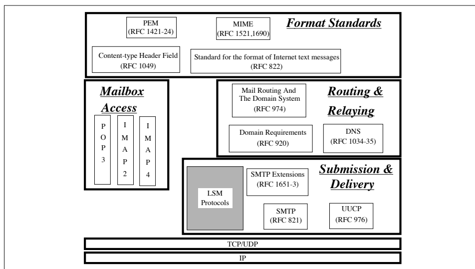
Figure 8.2: Messaging Communication Stack and LSM
