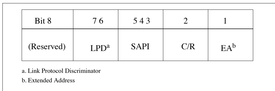
Figure 2.10: LAPDm Address Field
