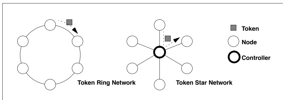
Figure 5.3: Token Passing Networks
