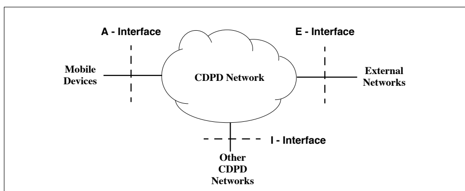
Figure 3.3: CDPD Interface Model
