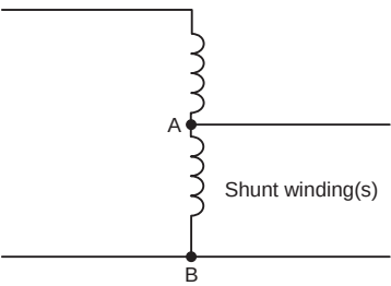
Figure 450.4 Autotransformer.
