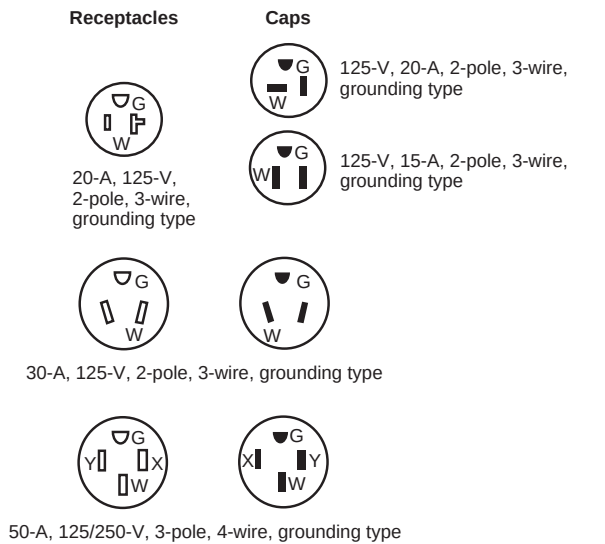
Figure 551.46(C) Configurations for Grounding-Type Receptacles and Attachment Plug Caps Used for Recreational Vehicle Supply Cords and Recreational Vehicle Lots.
