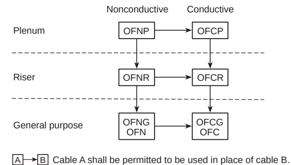
Figure 770.154(E) Cable Substitution Hierarchy.
