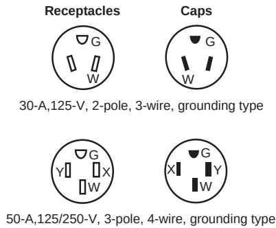
Figure 552.44(C) Attachment Cap and Receptacle Configurations.
