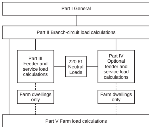
Figure 220.1 Branch-Circuit, Feeder, and Service Calculation Methods.
