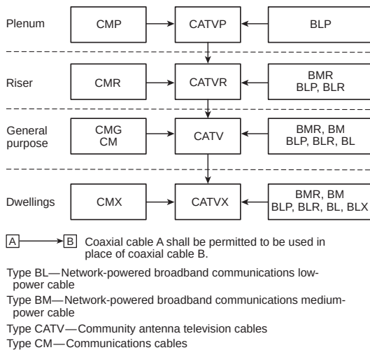
Figure 820.154(E) Cable Substitution Hierarchy.
