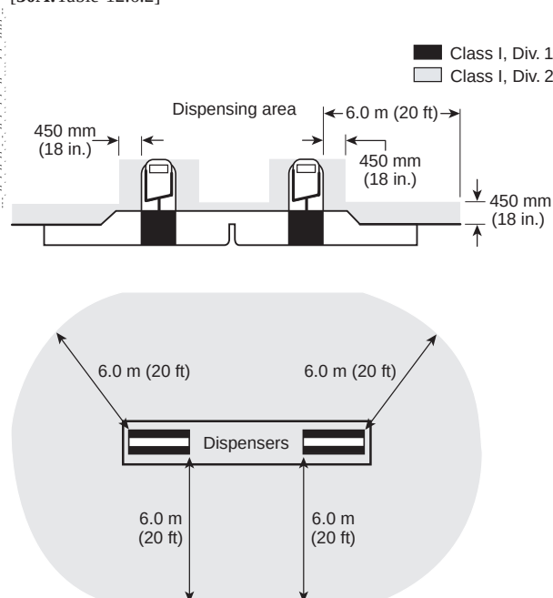
Figure 514.3 Classified Areas Adjacent to Dispensers as Detailed in Table 514.3(B)(1). [30A:Figure 8.3.1]
