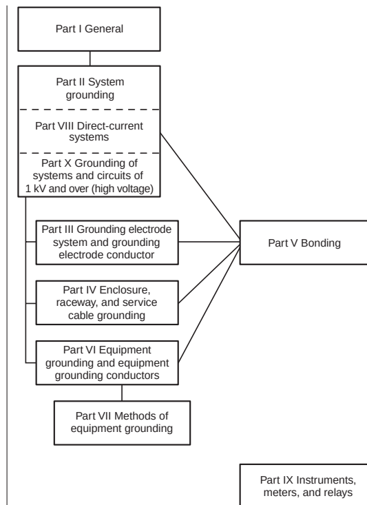
Figure 250.1 Grounding and Bonding.
