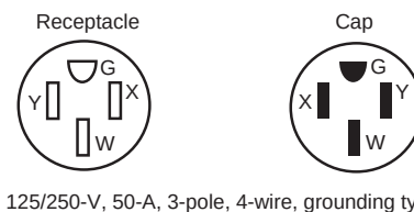
Figure 550.10(C) 50-Ampere, 125/250-Volt Receptacle and Attachment Plug Cap Configurations, 3-Pole, 4-Wire, Grounding-Types, Used for Mobile Home Supply Cords and Mobile Home Parks.
