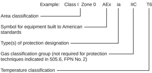
FPN Figure 505.9(C)(2) Zone Equipment Marking.
