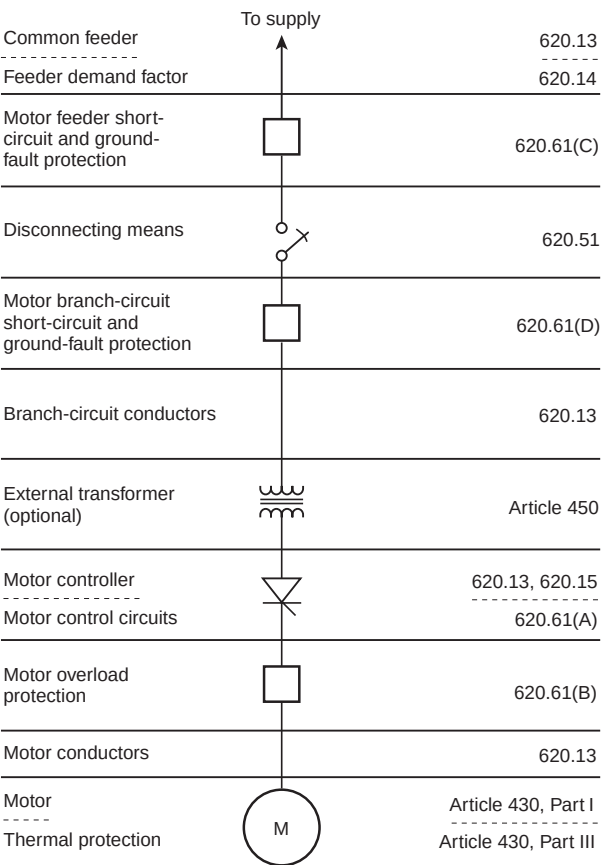
Figure 620.13 Single-Line Diagram.
