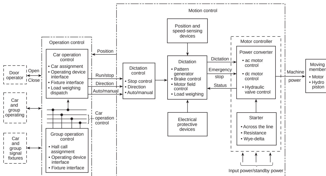
FPN Figure 620.2 Control System.
