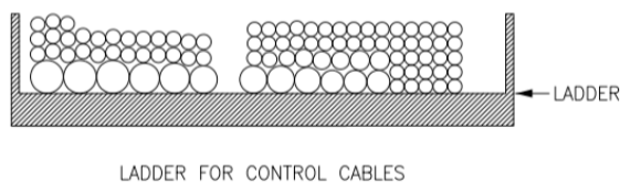
Figure 5. The comparison for cable fill allowance
