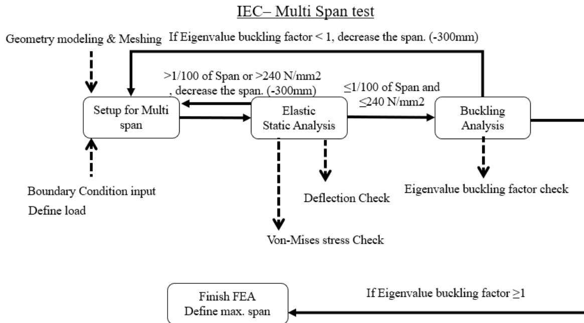
Figure 7. IEC-Test flow diagram
