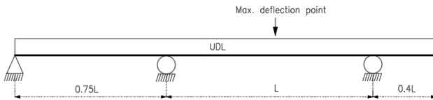
Figure 12. Continuous simply supported beam with over-hanging
