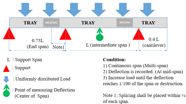
Figure 4. Deflection load test with multiple span according to IEC 61537 type test II
