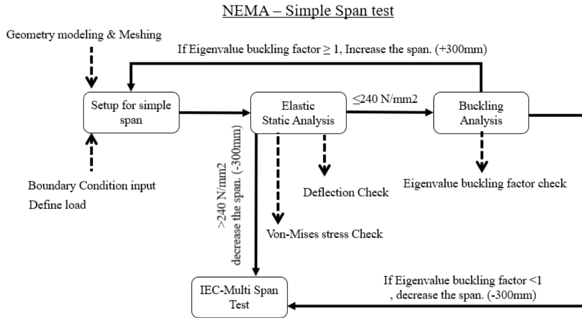
Figure 6. NEMA-Test flow diagram
