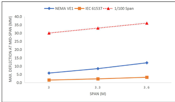
Figure 20. Max. deflection at the middle of span
