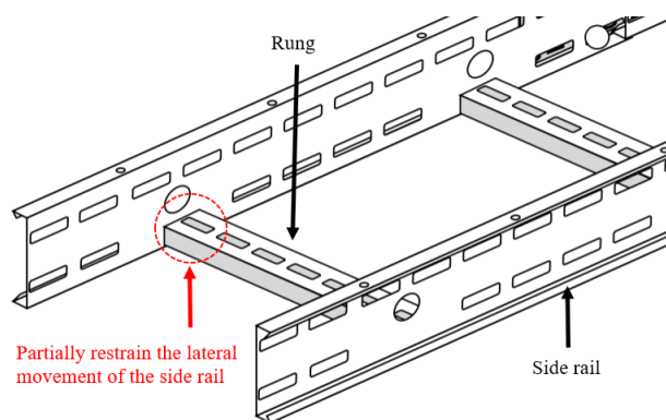
Figure 1. Partial lateral restraint of cable ladder [13]
