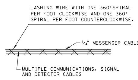
DOUBLE LASHING DETAIL
