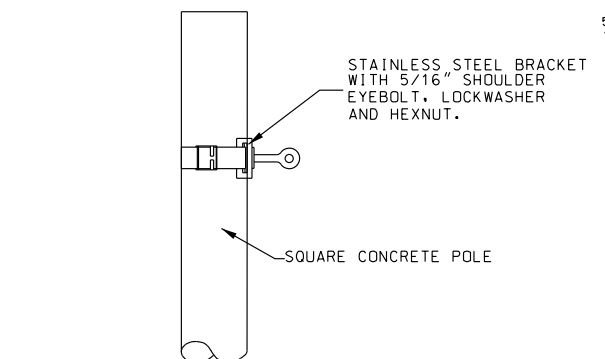
TYPICAL POLE ATTACHMENT FOR SQUARE CONCRETE POLE
