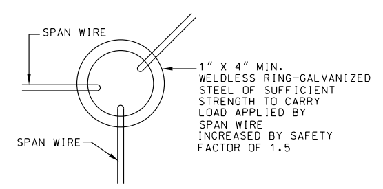
DETAIL A TENSION RING (TYP.)
