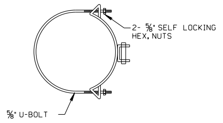
U-BOLT CLAMP
