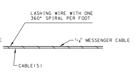
TYPICAL LASHING DETAIL
