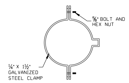
SPLIT CLAMP
