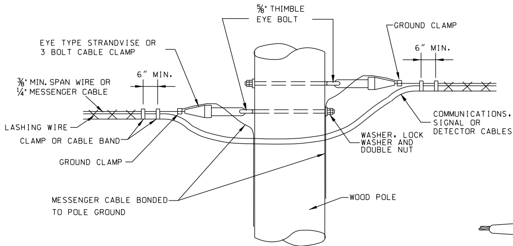
ALTERNATE CABLE CONTINUATION-SEPARATE MESSENGER CABLE
