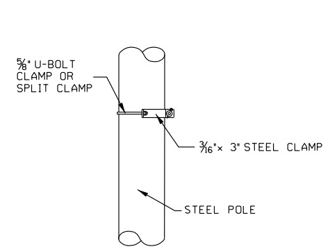
TYPICAL POLE ATTACHMENT FOR STEEL POLE
