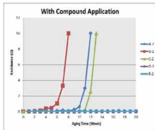
Figure 5 Resistance change for all No.2 connectors under salt mist aging
