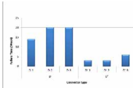
Figure 8 Failure time comparisons for connector D following torque requirements and not (D')
