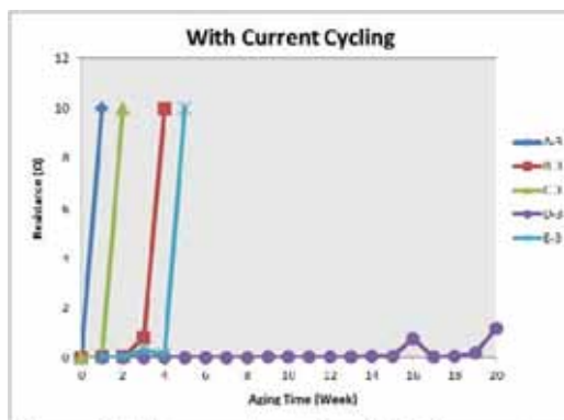
Figure 6 Resistance change for all No.3 connectors under salt mist aging
