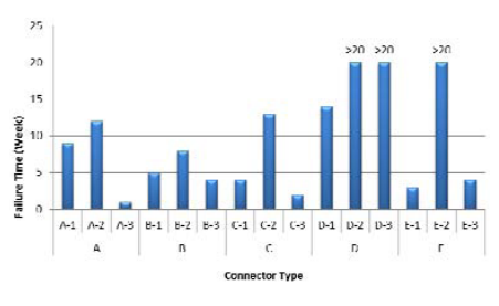
Figure 7 Failure time analysis for all connectors under salt mist aging
