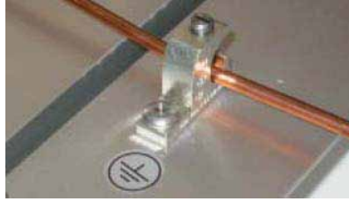
Figure 1 Lay-in lug Listed for direct burial (DB) and outdoor use
