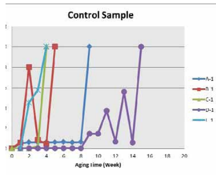
Figure 4 Resistance change for all No.1 connectors under salt mist aging
