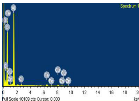
Figure 11 EDX measurements for the white oxidation on the aluminum frames
