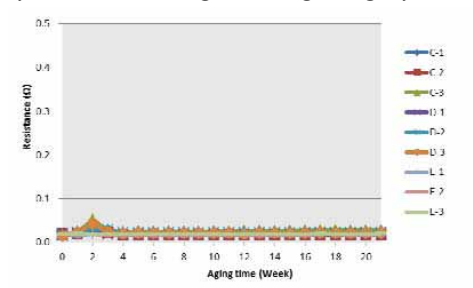
Figure 3 Resistance measurements for group C, D and E connectors under damp heat aging
