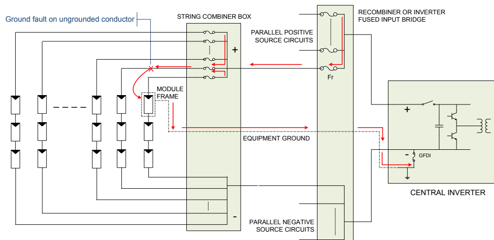
Figure 4: Representation of a DC Ground Fault to a Module Frame
