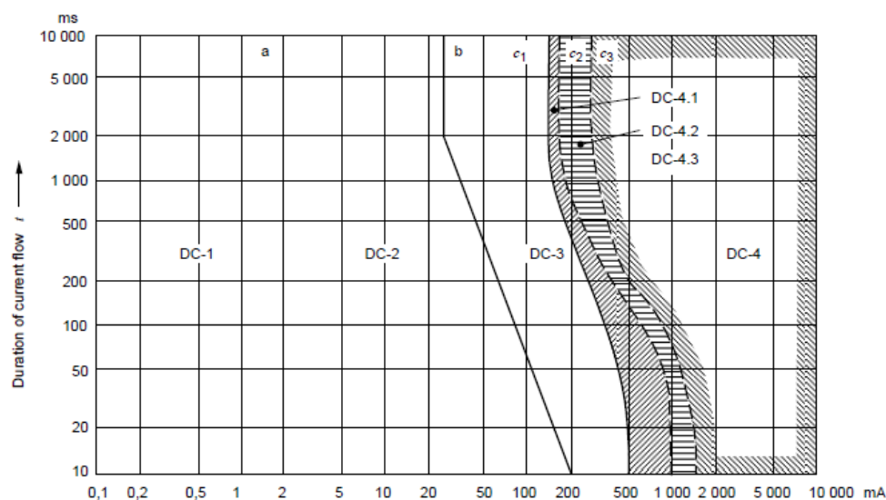
Figure 3: DC Time-Current Curves and Zones Defining the Typical Impact on Human Beings (IEC, 2005)
