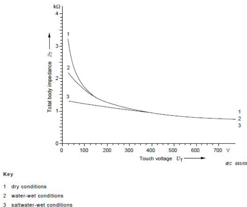
Figure 1: Total Body Impedances for a Current Path of Hand-to-Hand for a Percentile Rank of 50% of the Population (50/60 Hz AC) (IEC, 2005)
