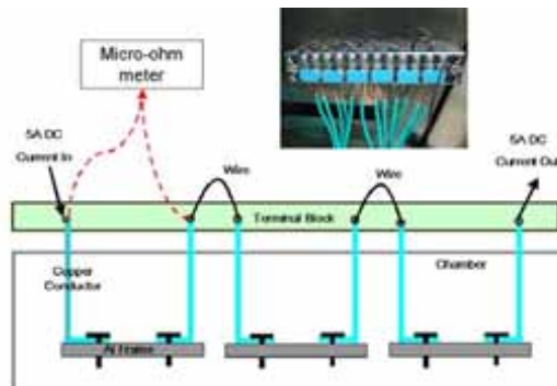
Figure 2 Sample layout for the corrosion cycling
