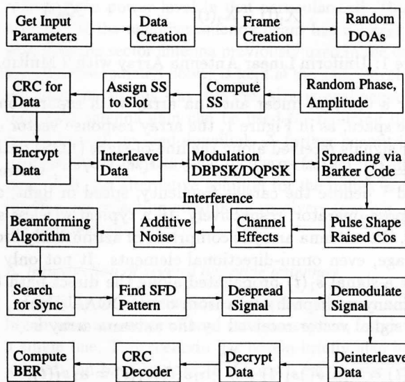
Figure 2: The SWL Physical Layer Block Diagram
