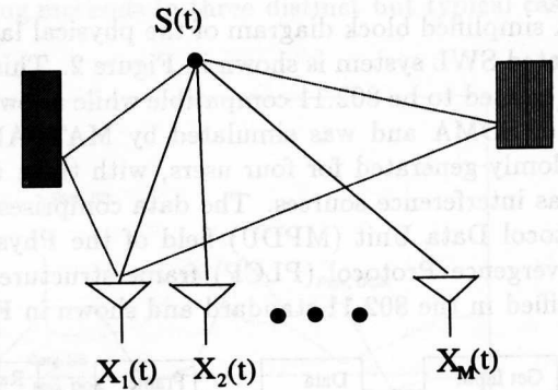
Figure 1: Uniform Linear Antenna Array with 2 Multipath
