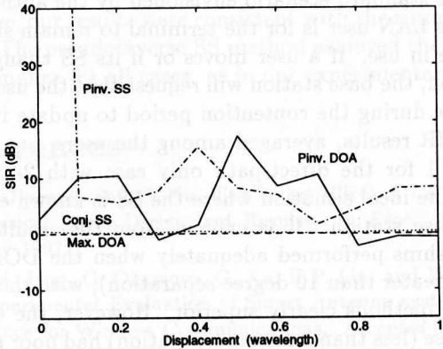
Figure 5: SIR Results for LOS User for Small Displacement
