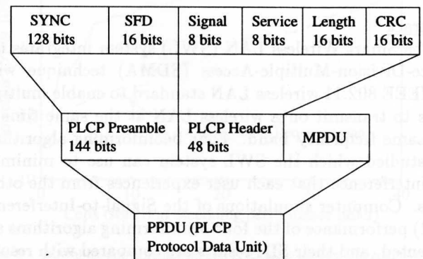
Figure 3: The Physical Layer Convergence Protocol Frame
