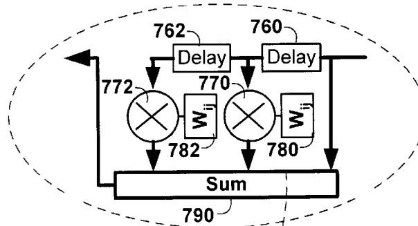
Space-Time Processor FIG. 7C
