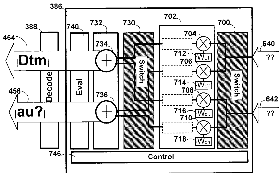
Spatial Processor
