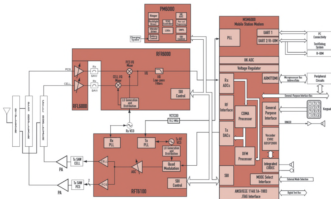
Figure 1. MSM6000 Chipset Architecture Using QCT's radiOne Zero Intermediate Frequency (ZIF)
