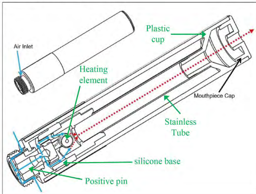
Figure H-12: Vuse Ciro Cartridge Air Flow Path
