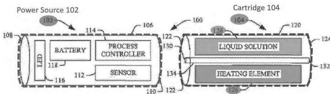
JX-0005 (881 Patent) at Fig. 1 (annotated to identify two pieces pieces—power source 102 and cartridge 104)
