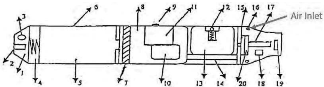
JX-0544 (Han 311) at Fig. 1 (annotated)
