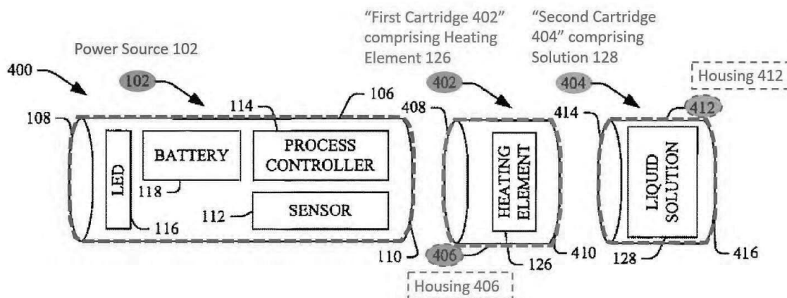
JX-0005 (881 Patent) at Fig. 4 (annotated to identify three pieces—power source 102, atomizer/cartridge 402, and cartridge 404)
