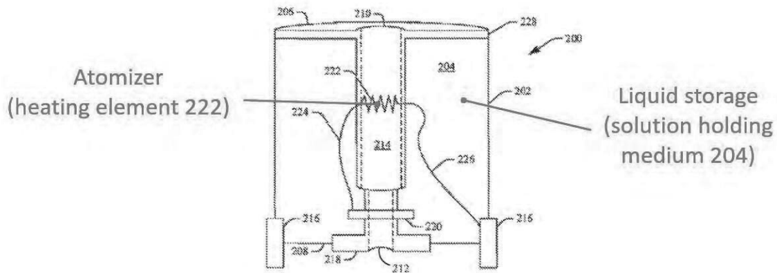
JX-0005 (881 Patent) at Fig. 2 (annotated to identify atomizer and liquid storage integrated into cartridge 200)
