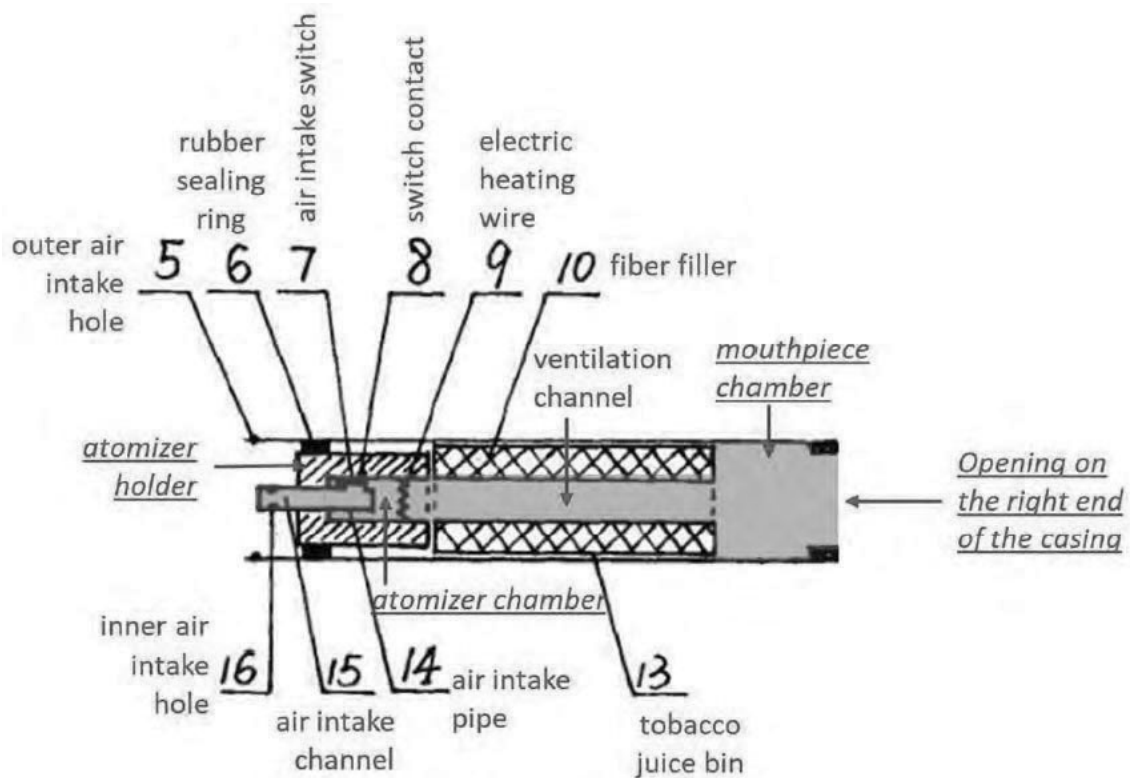
JX-0632C (Leinsing Opening Report) (Mr. Leinsing's Second Proposed Airflow Passageway ¶ 349)
