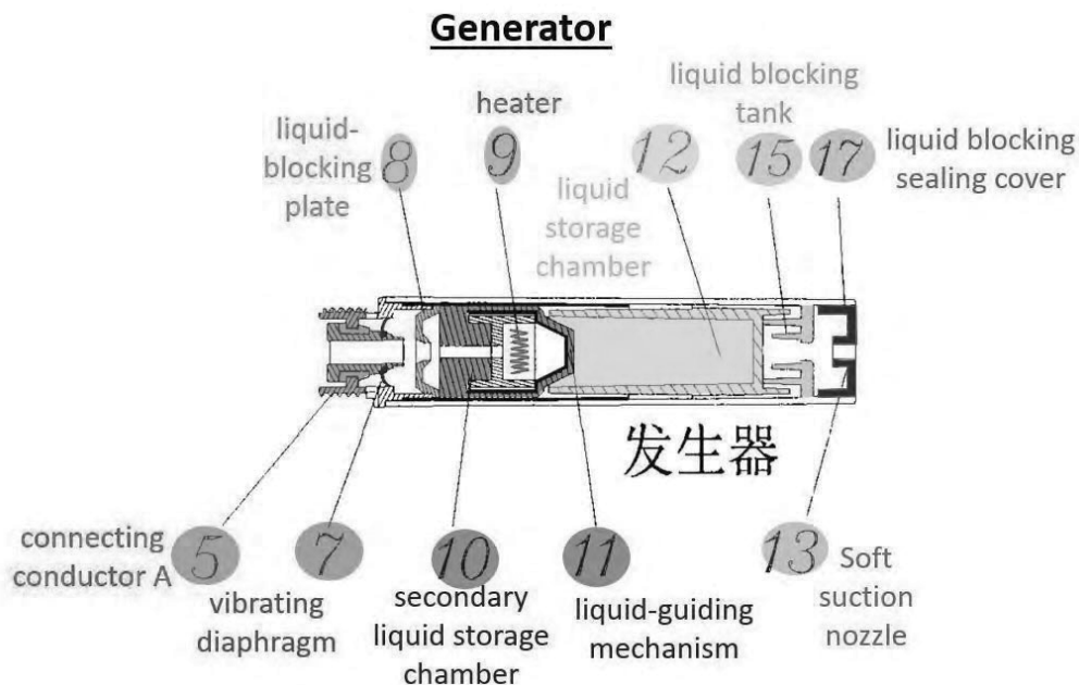
JX-0633 (Xia 610) at Fig. 2 (partial, annotated)
