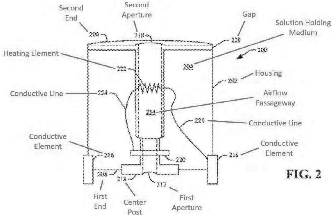
JX-0005 (881 Patent) at Fig. 2 (annotated) 3
