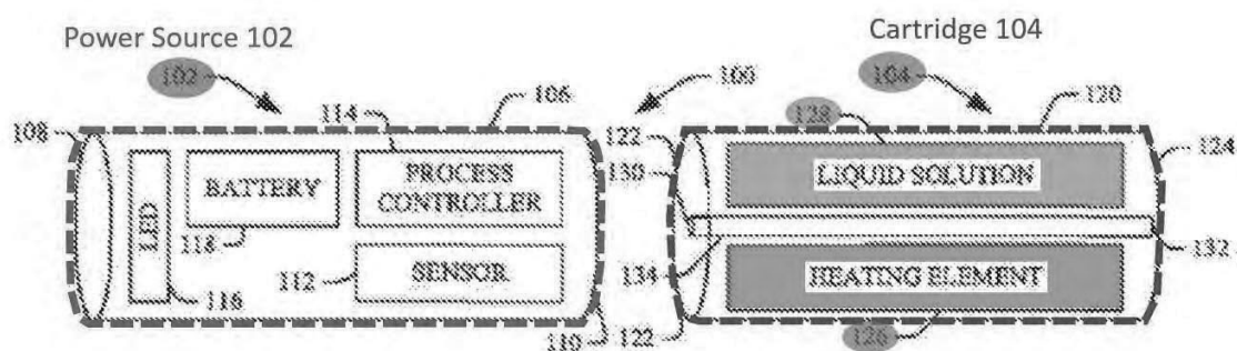
JX-0005 (881 Patent) at Fig. 1 (annotated to identify two pieces—power source 102 and cartridge 104)
