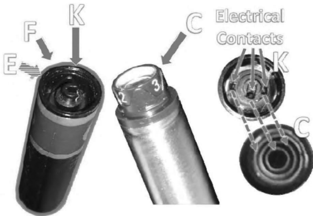
CX-2157 (Vallee Opening Report) ¶ 1873 (Photo of VUSE Solo G1 Cartridge Housing [E] With a First End [F] Adapted to Electrically Couple [K] and Mechanically Couple to a Conductive Portion [C] of the VUSE Solo Power Unit)
