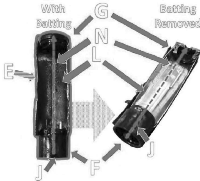
CX-2157 (Vallee Opening Report) ¶ 1892 (Photo of VUSE Solo G1 Cartridge Showing Interior of Housing [E] With a Solution Holding Medium [L] that Surrounds the Airflow Passageway [J] and Heating Element [N] Between the First and Second Ends [F, G])
