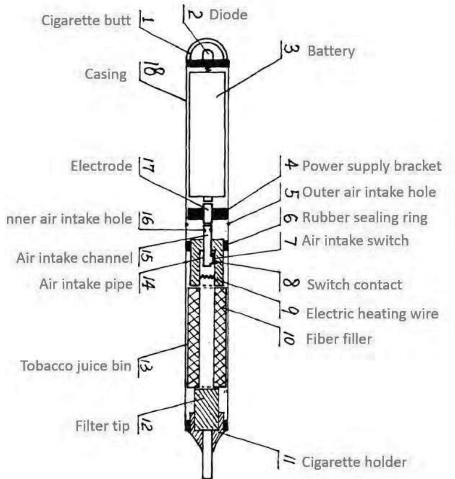
JX-0594 (Wang 927) at Fig. 1 (annotated)
