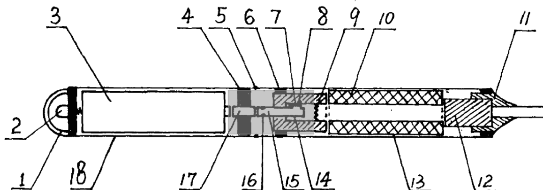
JX-0594 (Wang 927) at Fig. 1 (Depicting Components Between Battery 3 and Heating Wire 9)
