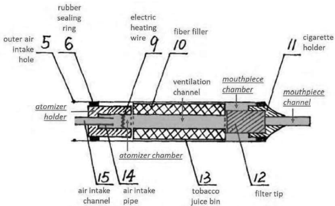
JX-0632C (Leinsing Opening Report) (Mr. Leinsing's Third Proposed Airflow Passageway ¶ 351)
