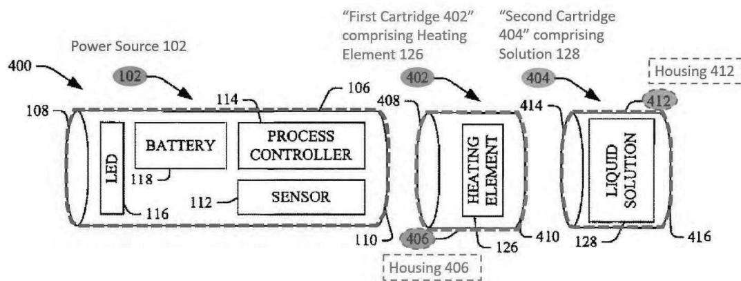
JX-0005 (881 Patent) at Fig. 4 (annotated to identify three pieces—power source 102, cartridge 402 comprising heating element 126, and cartridge 404 comprising solution 128)
