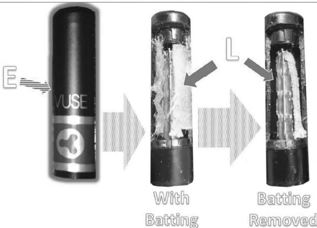
CX-2157 (Vallee Opening Report) ¶ 1880 (Photo of VUSE Solo G2 Cartridge Housing [E] (Left), Interior with Batting [L] (Middle), and Without Batting to Show the Portions Wick Outside the Heating Coil [L] (Right))
