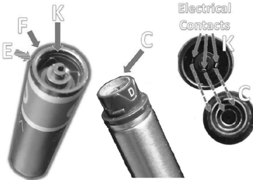
CX-2157 (Vallee Opening Report) ¶ 1873 (Photo of VUSE Solo G2 Cartridge Housing [E] With a First End [F] Adapted to Electrically Couple [K] and Mechanically Couple to a Conductive Portion [C] of the VUSE Solo Power Unit)
