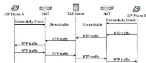
Figure 7. Behind different NATs
