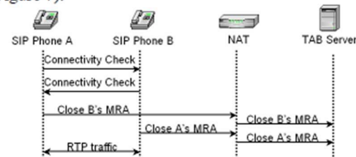
Figure 6. Behind the same NAT
