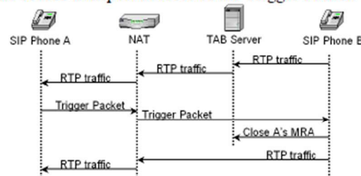
Figure 5. Trigger the shortest path
