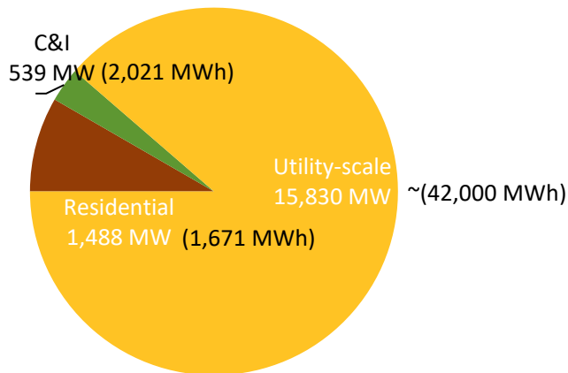
Cumulative U.S. BESS Installations as of December 2023 (17.9 \text{GW}_{\text{ac}} / ~44 GWh)
