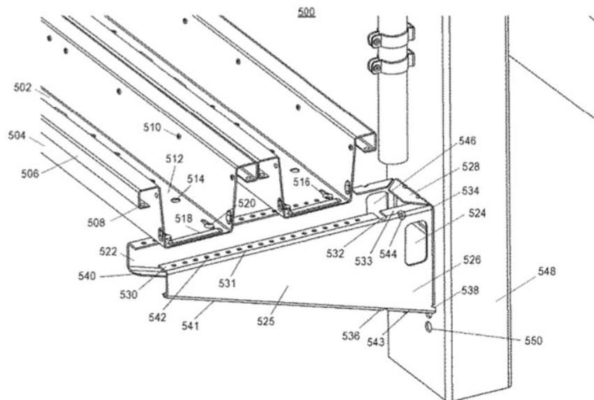
EX1003, FIG. 5.
