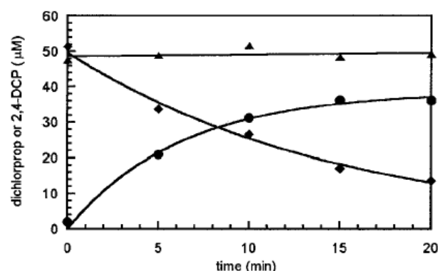
Fig. 4. Stereospecificity of dichlorprop-degrading activity of A. denitrificans cell extracts as measured by chiral HPLC. Concentrations of (S)-dichlorprop (▲), (R)-dichlorprop (◆), and 2,4-DCP (●) were measured at selected time points after incubation of A. denitrificans cell extracts (50 \mu l) with racemic dichlorprop (0.1 mM) and the standard reaction components. Dichlorprop was quantitated by using chiral HPLC and 2,4-DCP was quantitated colorimetrically. Data for the (S)-dichlorprop were fit to a straight line of slope 0.05 \mu\text{M min}^{-1} , for (R)-dichlorprop to exponential decay with an exponent of -0.067 \text{ min}^{-1} ; and for 2,4-DCP to Eq. (1) with an apparent inactivation rate of 0.16 \text{ min}^{-1} .
