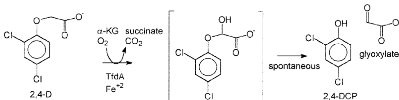
Scheme 1. Reaction catalyzed by TfdA with 2,4-D.
