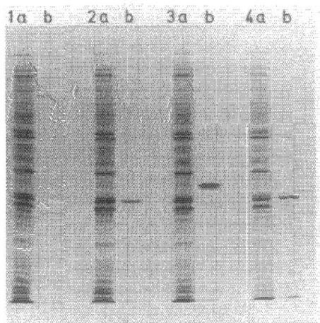
FIG. 4. Omega mutagenesis of gene tfdA . The omega fragment, which carries transcriptional and translational stop signals, was inserted at a Bgl II site situated within the coding region of tfdA on plasmid pTJS'X535. Gene expression was induced using the T7 RNA polymerase-promoter system. Protein was labeled with L-[ 35 S]methionine, loaded onto a 12.5% SDS-polyacrylamide gel, and revealed by autoradiography. No protein is expressed from the vector plasmid pT7-5 (lanes 1). A truncated tfdA gene product is expressed from both omega-mutagenized plasmids pTJS'X535omega (lanes 2 and 4), whereas a full-length protein is expressed from pTJS'X535 (lanes 3). Samples were labeled after heat induction and addition of rifampin (lanes b) or omitting induction and rifampin addition (lanes a).
