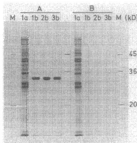
FIG. 2. Expression of gene tfdA by T7 RNA polymerase. Three DNA fragments able to confer PAA degradation on A. eutrophus JMP222 (1, 2.8-kb Sac I- Sac I; 2, 2.1-kb Bam HI- Sac I; 3, 1.4-kb Xba I- Sac I) were cloned in T7 promoter plasmids pT7-5 (A) and pT7-6 (B), yielding constructions with both orientations of the insert in relation to the T7 promoter. Strains of E. coli K38 carrying a heat-inducible T7 RNA polymerase gene on plasmid pGP1-2 and one of the hybrid pT7 plasmids were used for specific labeling of plasmid-encoded proteins: gene expression was induced by heat, the host RNA polymerase was inhibited with rifampin, and cells were pulsed with L-[ 35 S]methionine as described in Materials and Methods (lanes b). For labeling of total cell protein, samples were treated omitting both heat induction and rifampin addition (lanes a). Proteins were separated by electrophoresis on a 12.5% SDS-polyacrylamide gel and revealed by autoradiography. Transcription from the Xba I to the Sac I site resulted in expression of a 32,000-dalton protein (panel A), whereas no protein was expressed from opposite orientations (panel B). M, Molecular weight markers (transferred from Coomassie blue-stained gel).
