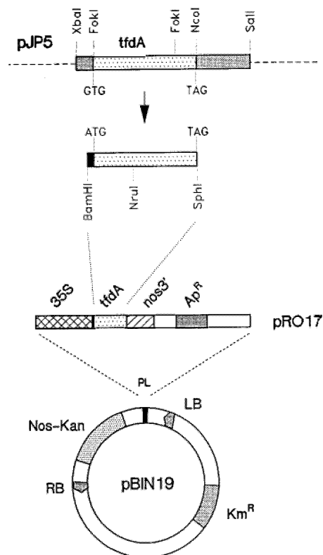
Fig. 1. Schematic representation of the tfdA gene from pJP5 leading to constructs pRO17 and pBIN19::pRO17. Only restriction sites relevant to the text are shown. 35S cauliflower mosaic virus 35S promoter, nos3' polyadenylation signal-containing fragment from nopaline synthase gene, Ap R bacterial ampicillin resistance gene, Km R bacterial kanamycin resistance gene, Nos-Kan nopaline synthase promoter-kanamycin chimeric gene which confers resistance to kanamycin to plant cells, RB T-DNA right border sequence, LB T-DNA left border sequence, PL polylinker cloning site
