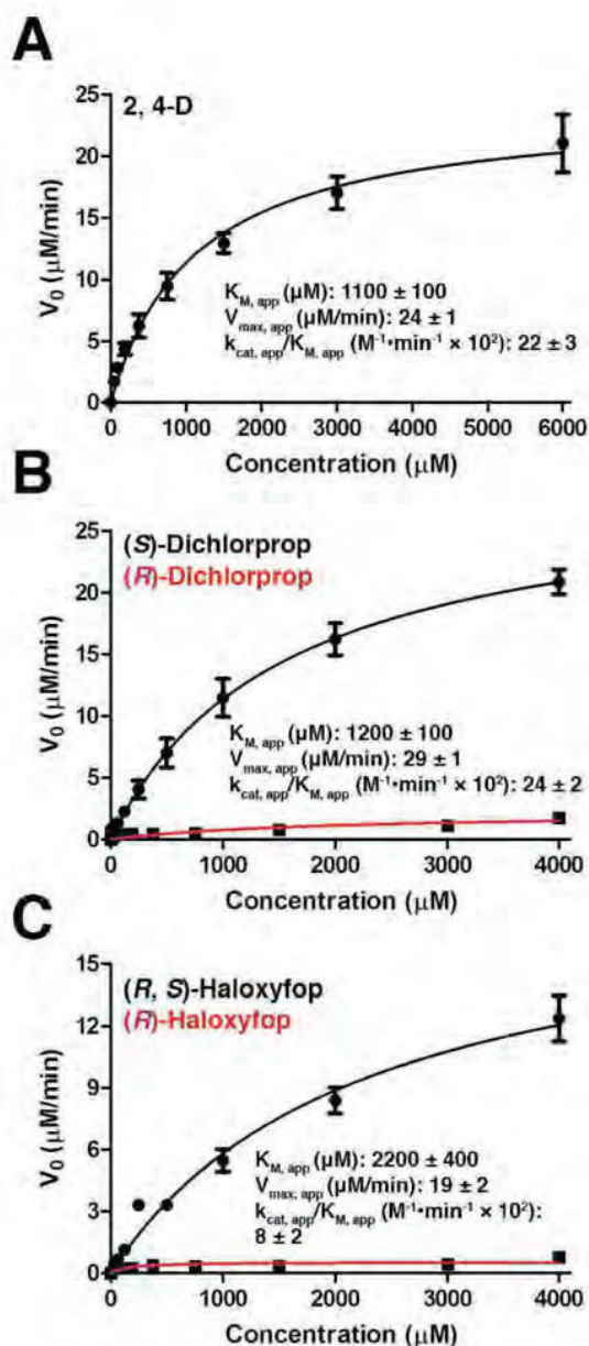
Supplementary Figure 6. Kinetic curves for the AAD-2 reaction using various substrates. (A) Kinetic curve of AAD-2 with 2,4-D at various concentrations. (B) Kinetic curves of AAD-2 with (S)-dichlorprop (black curve) or (R)-dichlorprop (red curve). (C) Kinetic curves of AAD-2 with (R,S)-haloxyp (black curve) or (R)-haloxyp (red curve). For racemic substrates, the concentration noted is the effective concentration of the (S) enantiomer in the sample. Kinetic parameters noted in each panel correspond to values calculated using the black curve in each panel.
